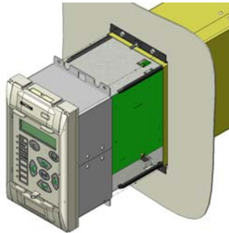
Figure 4: Fit P120R module into vacant MCGG case
