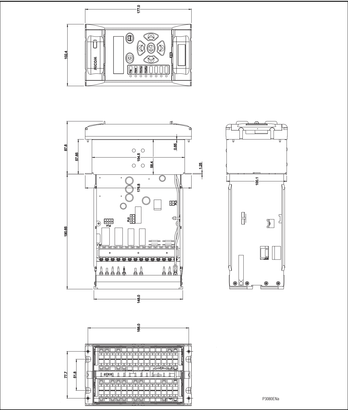
FIGURE 13: MiCOM P120R DIMENSIONS (WITHOUT MCGG CASE)
