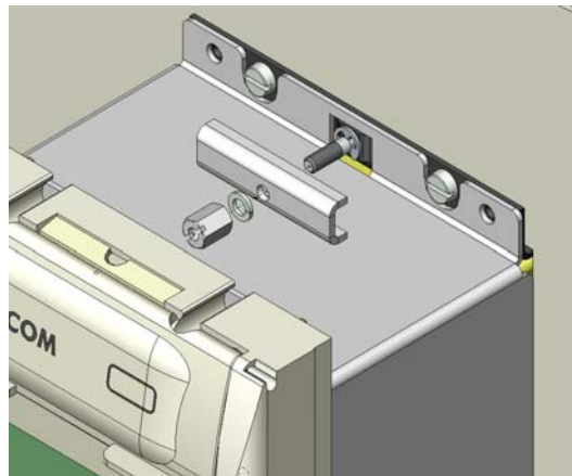
Figure 8: To remove P120R open top & bottom flaps and remove 4 fixing screws shown below, leaving mating collar in place (retain screws).
