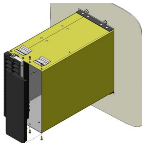
Figure 10: Where an RS485 communication port is required, remove MCGG22 rear blank panel (retain screws).
