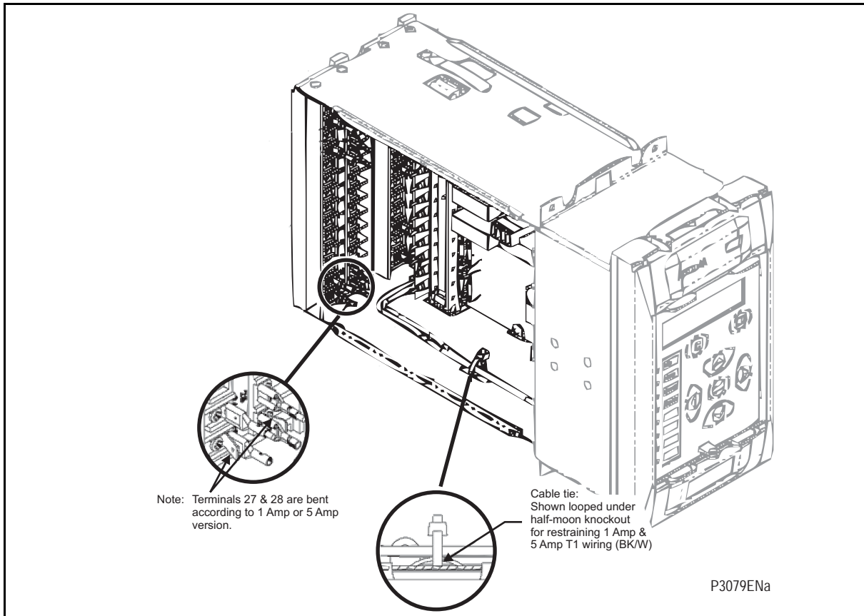
FIGURE 14: P120R INTERNAL WIRING OVERVIEW
