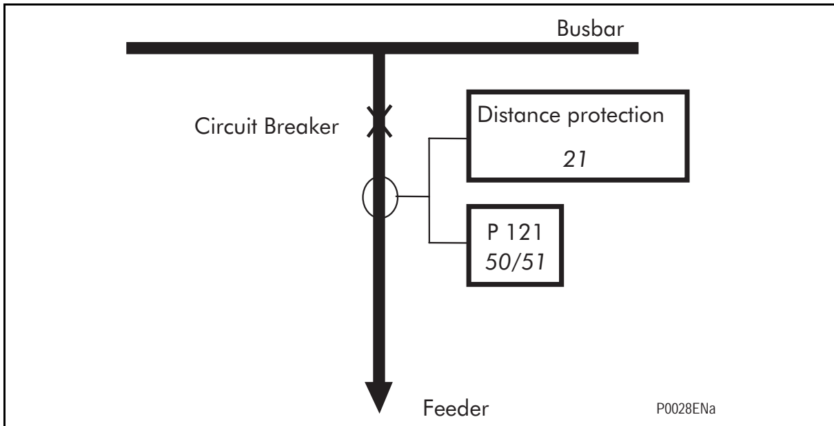
FIGURE 9: ASSISTANCE OF REMOTE PROTECTION BY A MiCOM P121 PROTECTION
