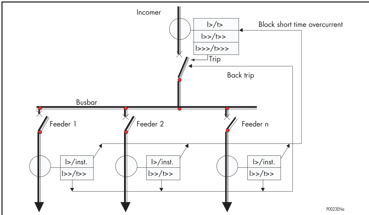
FIGURE 2: BLOCKED OVERCURRENT FOR BUSBAR PROTECTION
