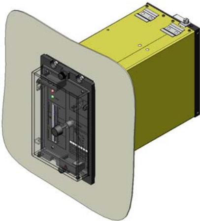
Figure 3: Withdraw MCGG22 relay active part
