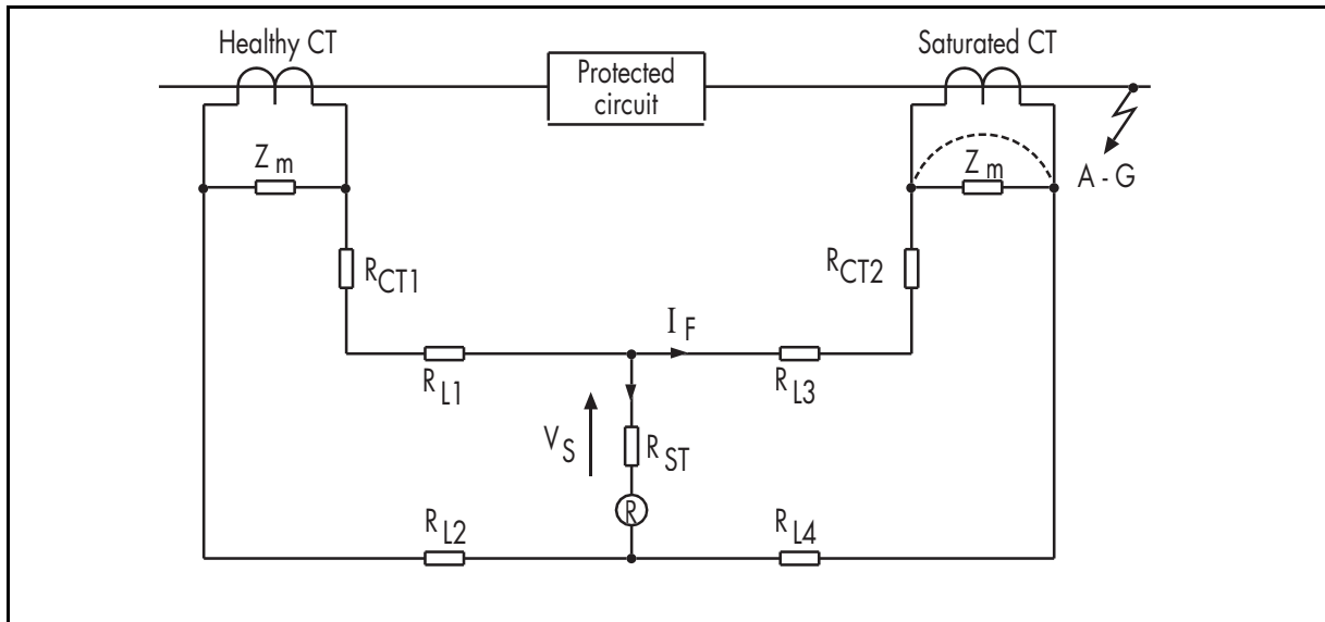
FIGURE 4: HIGH IMPEDANCE SCHEME PRINCIPLE
