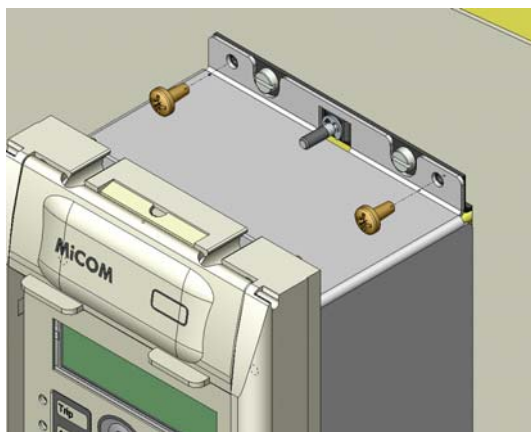
Figure 9: Refit P120R to collar using screws removed in figure 8 and close top and bottom flaps.
