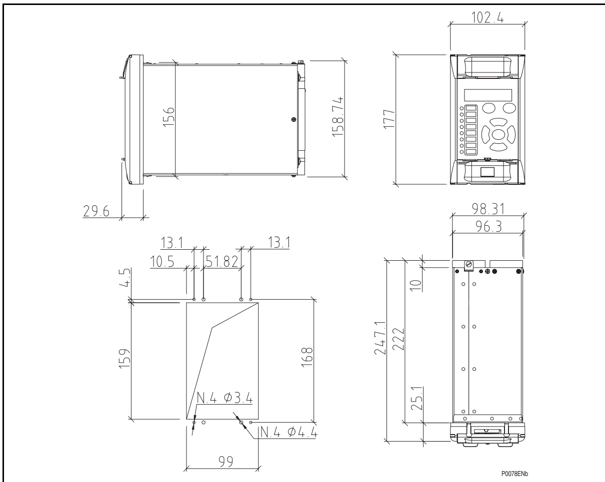
MiCOM P120, P121, P122 AND P123 RELAYS CASE DIMENSIONS
