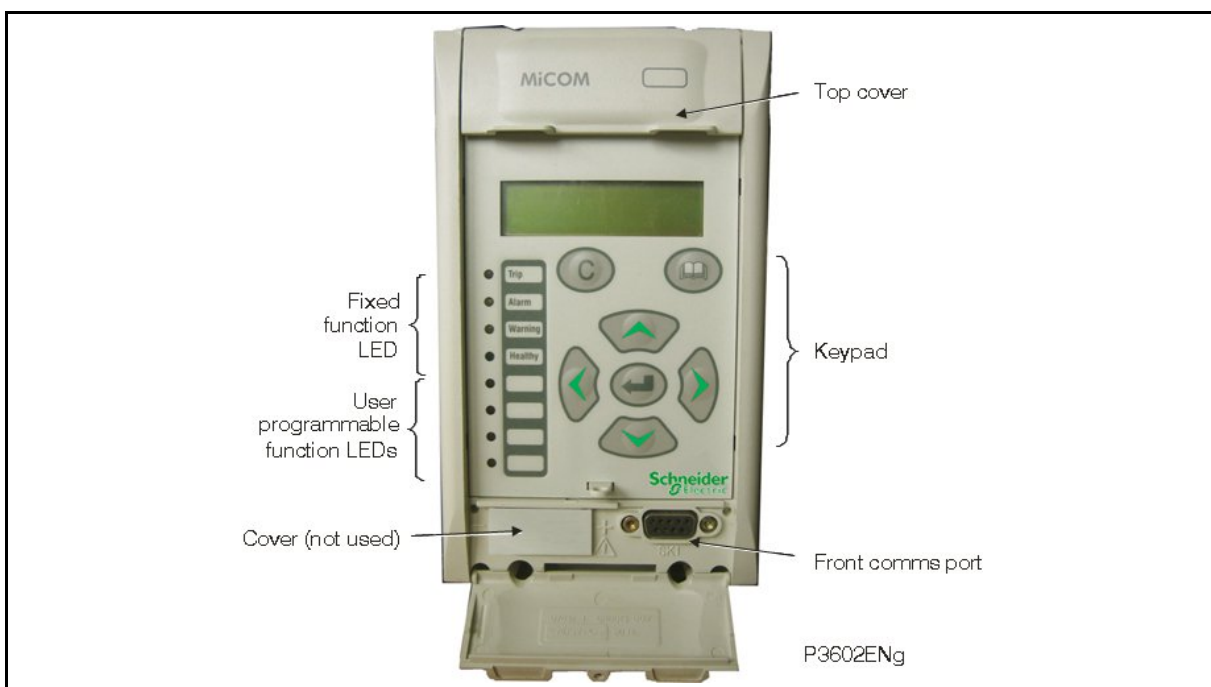
FIGURE 1: MiCOM P120, P121, P122 AND P123 FRONT PANEL DESCRIPTION
