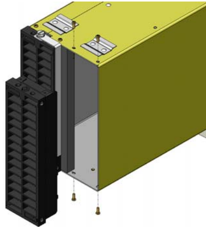
Figure 12: Fit rear terminal block using screws removed in figure 9.
