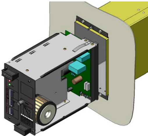
Figure 3: Withdraw MCGG22 relay active part
