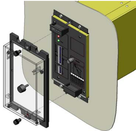
Figure 4: Fit P120R module into vacant MCGG case
