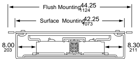
Typical Mounting of BD, BG, BJ, BK, HD, HG, HJ, HL, JD, JG, JJ, JL, LA, LG, LJ, LL, LR, MG, MJ, PG, PJ, PK, PL, QB, QD, QG, QJ Circuit Breakers
