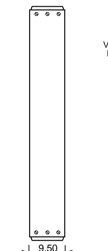
Typical Box Side View
