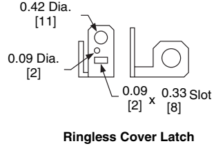
Ringless Cover Latch
