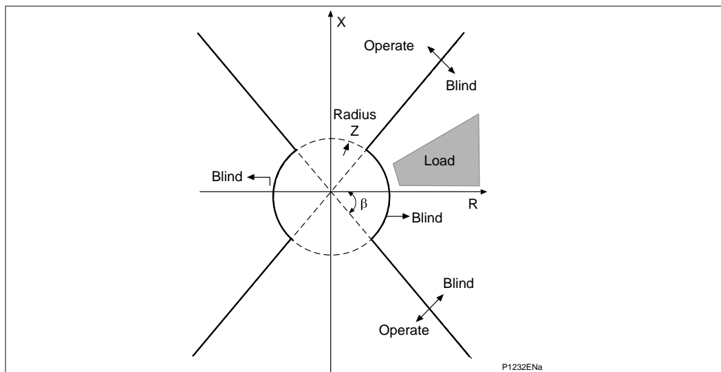
Figure 27 - Load blinder characteristics
