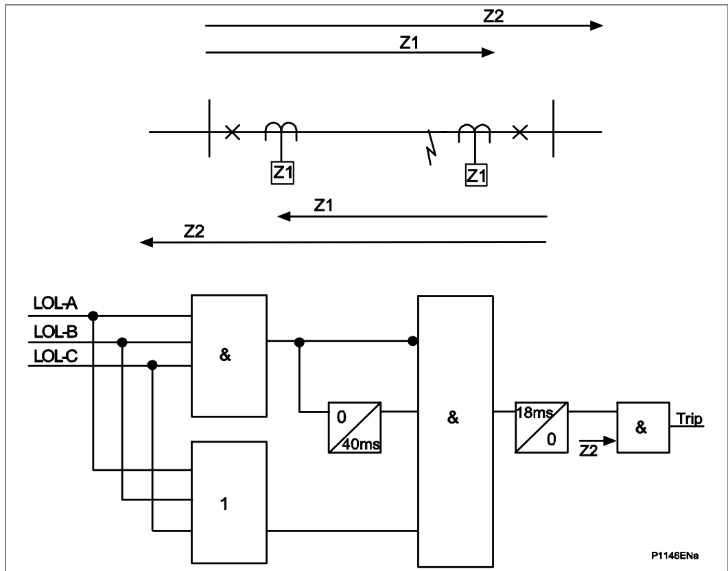
Figure 56 - Loss of load accelerated trip scheme (Distance option only)
