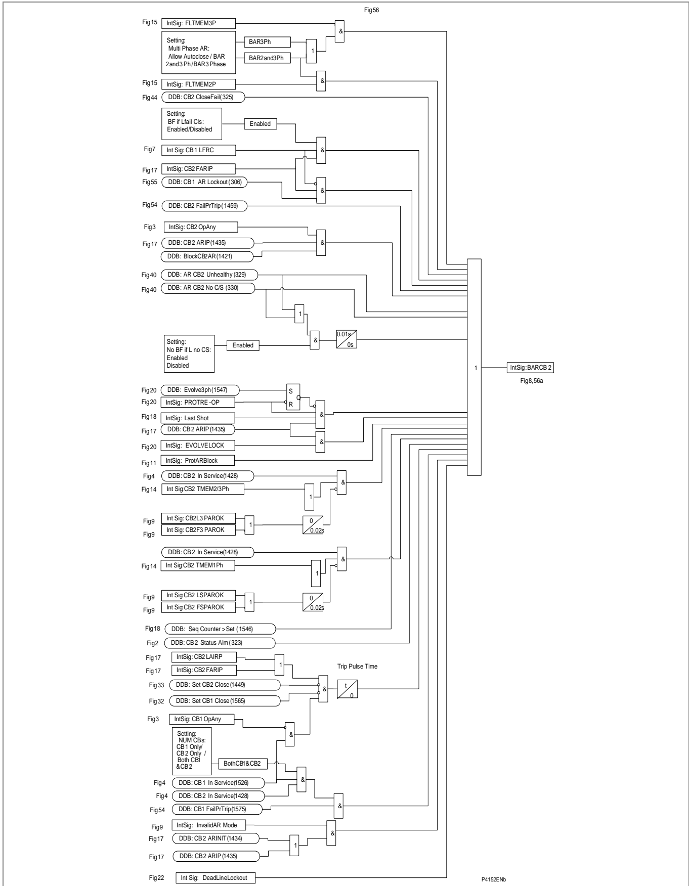
Figure AR-56 - Auto-reclose lockout – CB2 (for Software Versions H1 and later)
