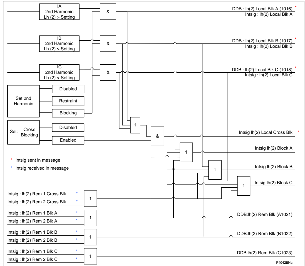
Figure 9 - Second harmonic restraint and blocking logic
