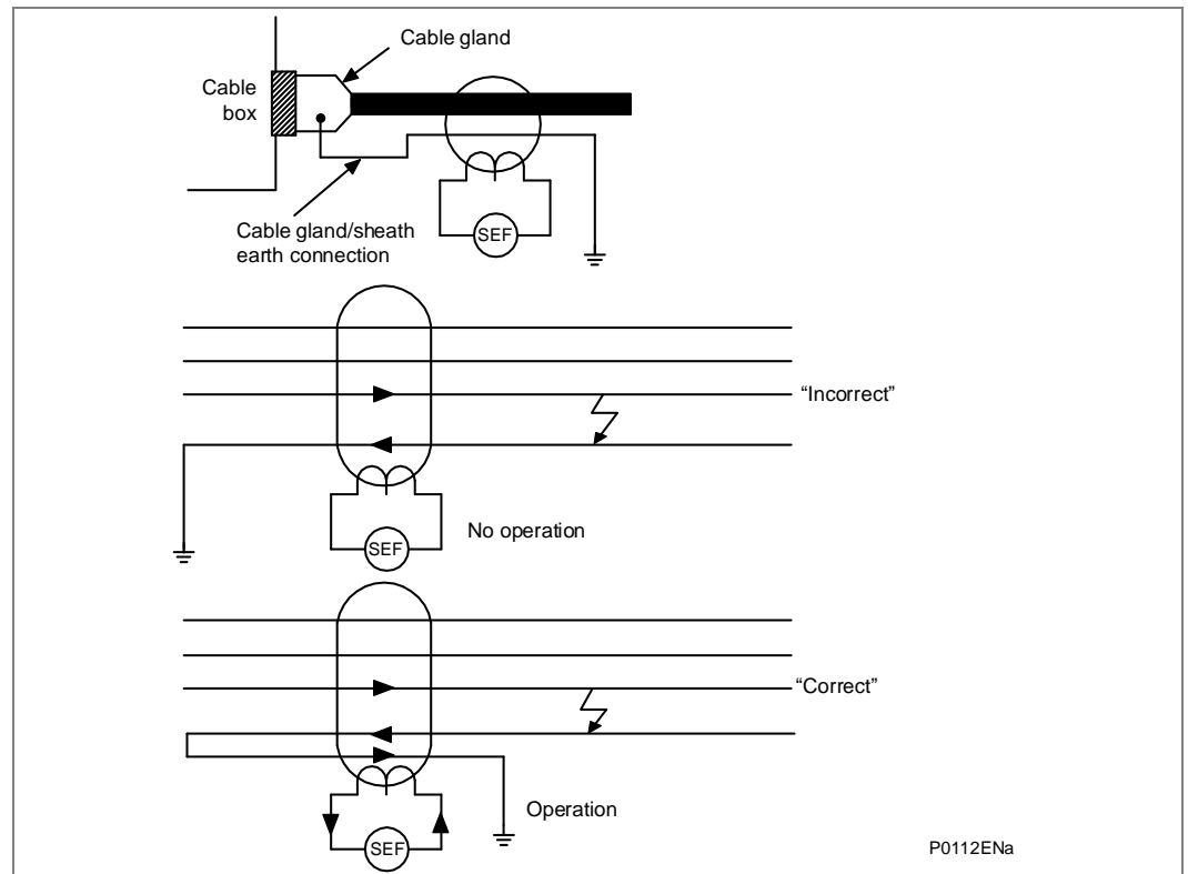
Figure 20 - Positioning of core balance current transformers
