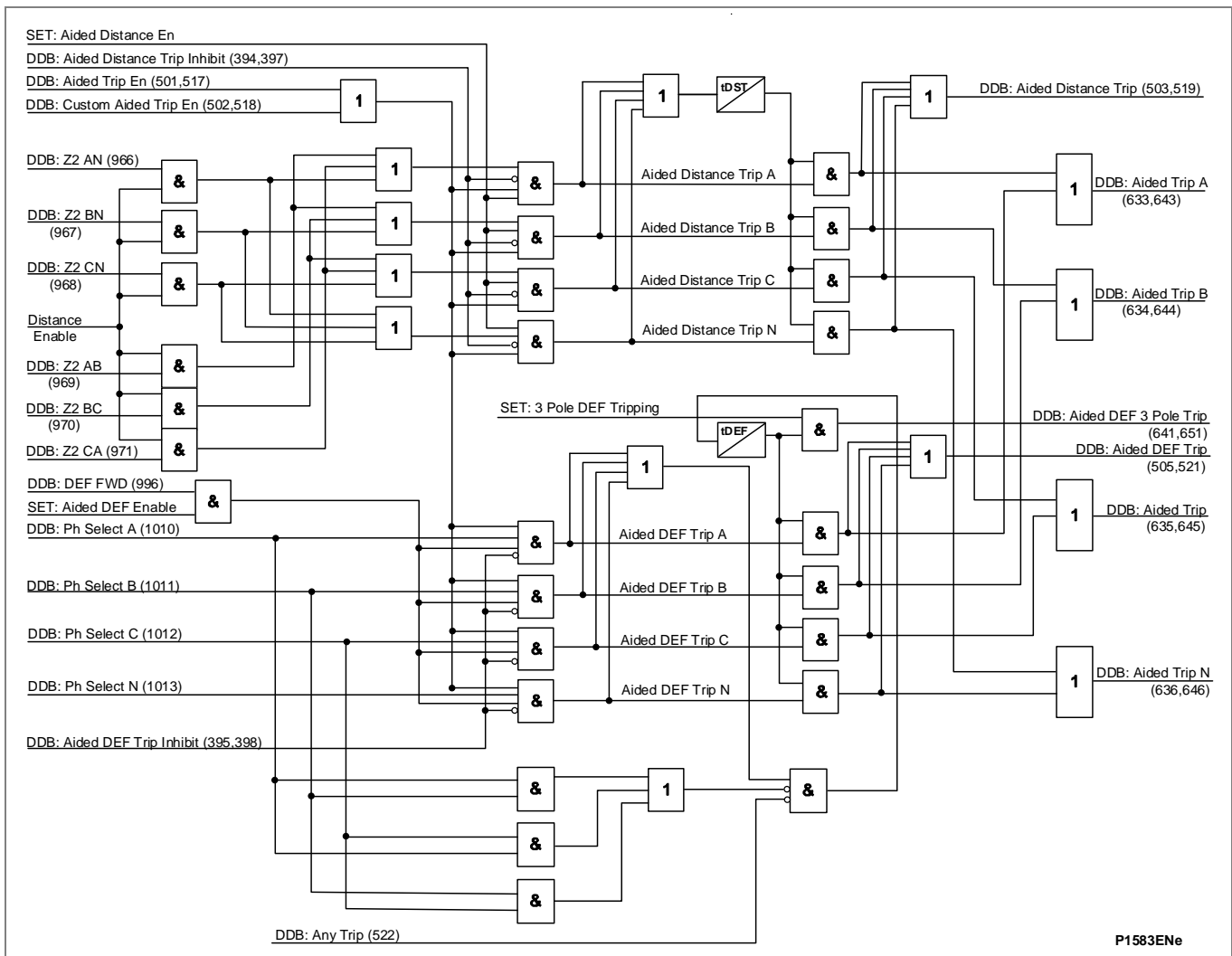
Figure 39 - Aided tripping logic
