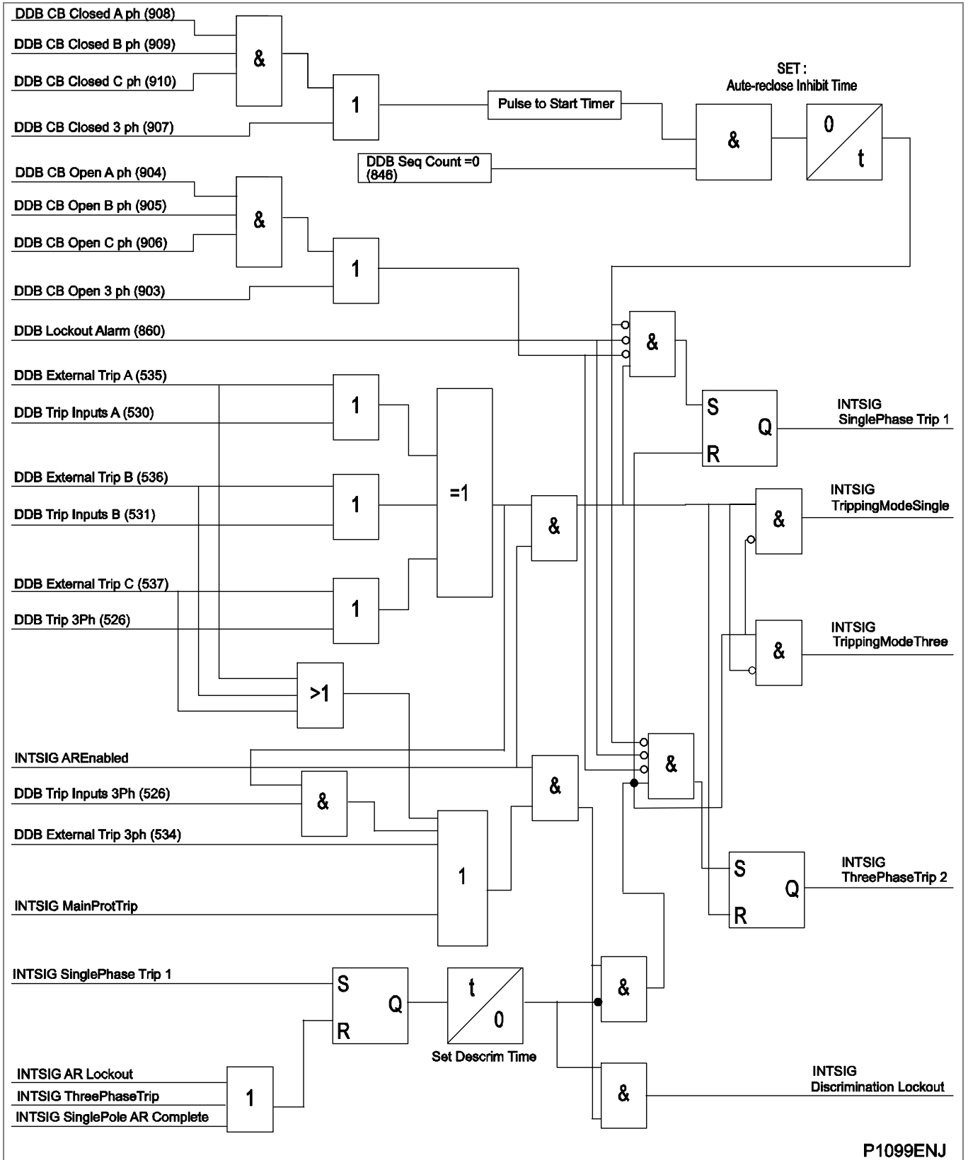
Figure 112 - Auto-reclose single/three pole tripping
