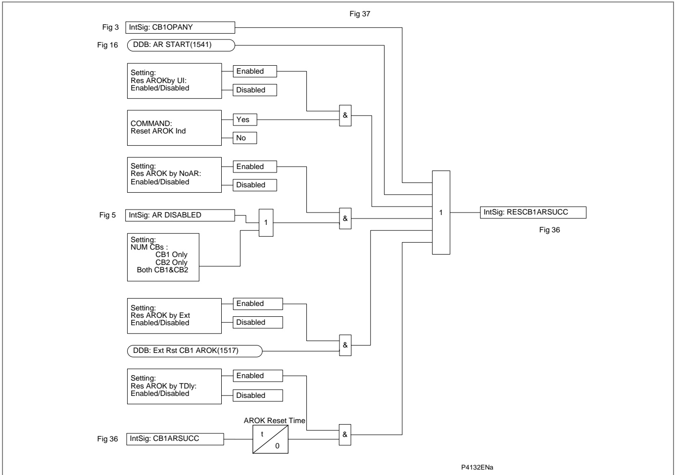
Figure AR-36 - Reset CB1 successful AR indication
