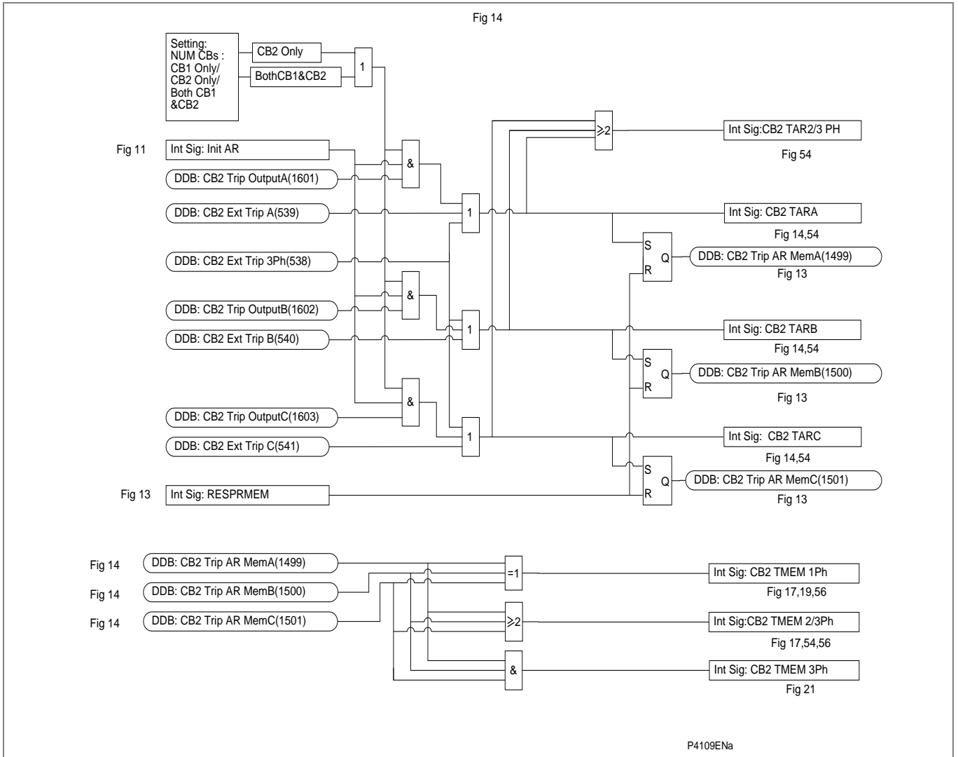
Figure AR-15 - CB2 1 pole / 3-pole trip + AR initiation
