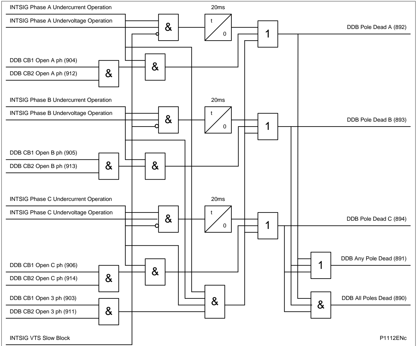
Figure 17 - Pole dead logic for P544/P546
