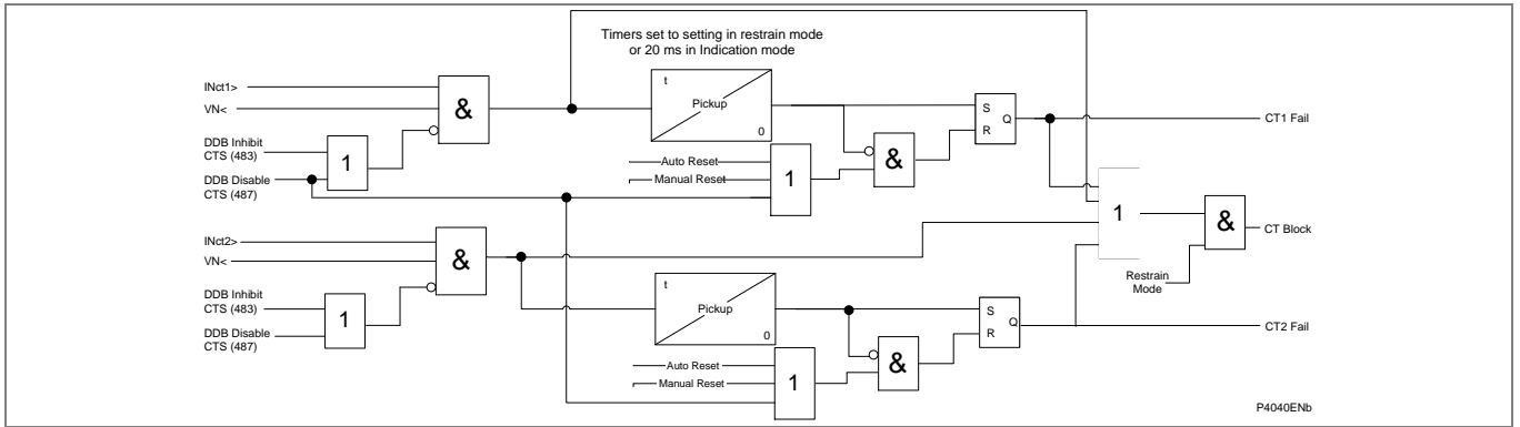
Figure 104 - Standard CTS
