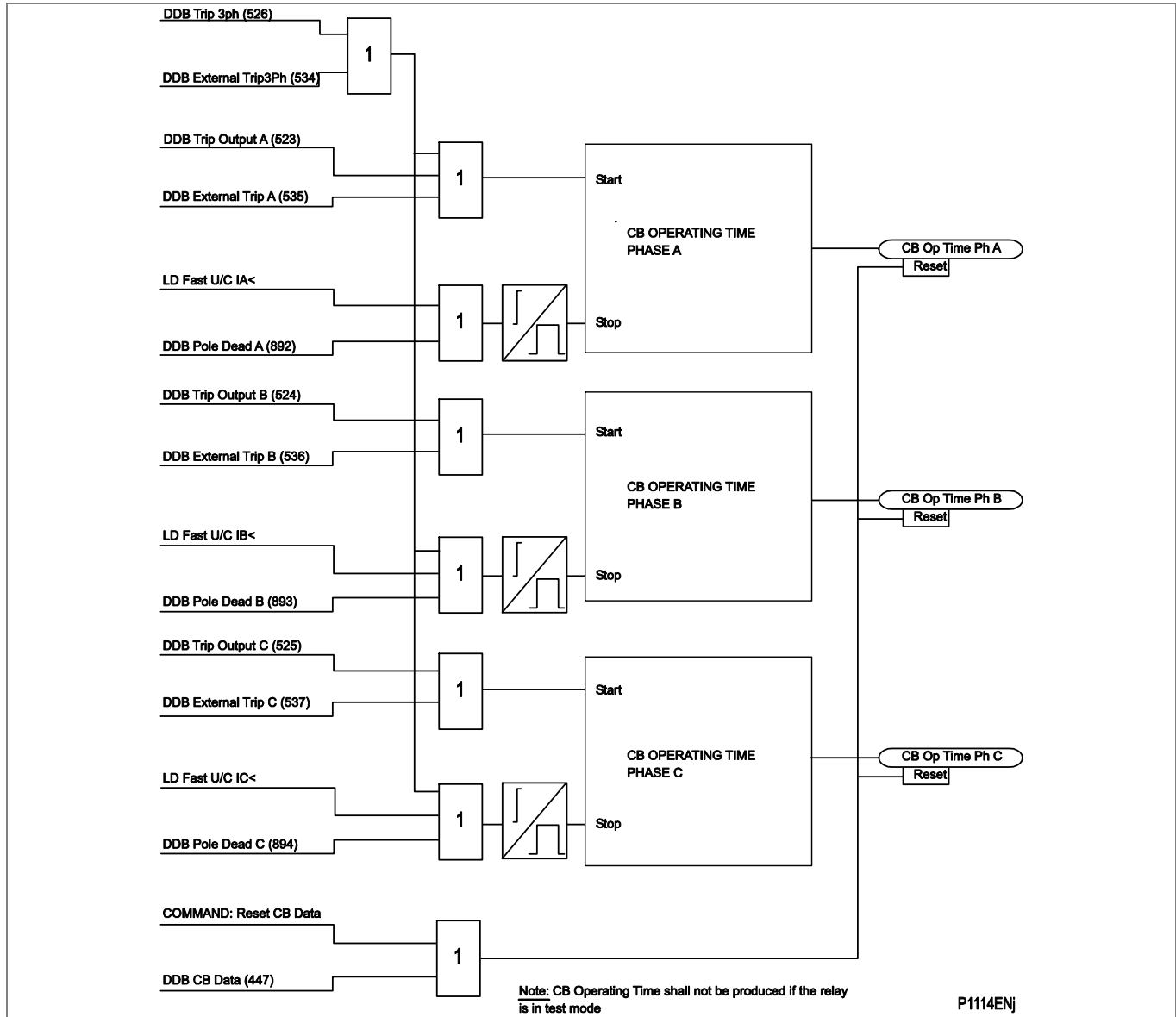
Figure 122 - Circuit breaker condition monitoring - operation time (P543/P545)
