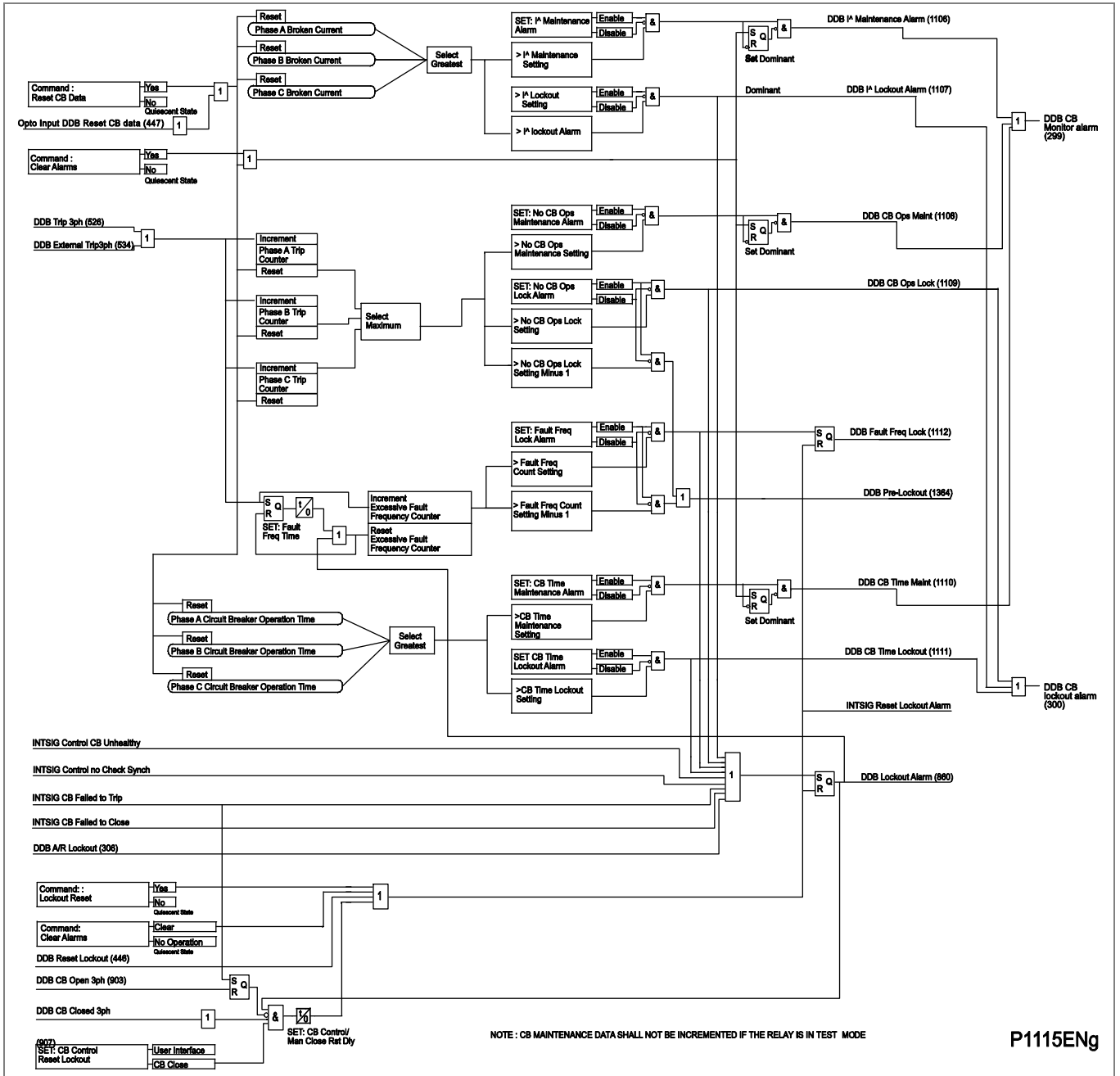
Figure 123 - CB monitoring (P543/P545)
