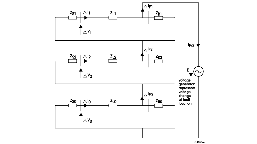
Figure 35 - Sequence networks connection for an internal A-N fault (Distance option only)
