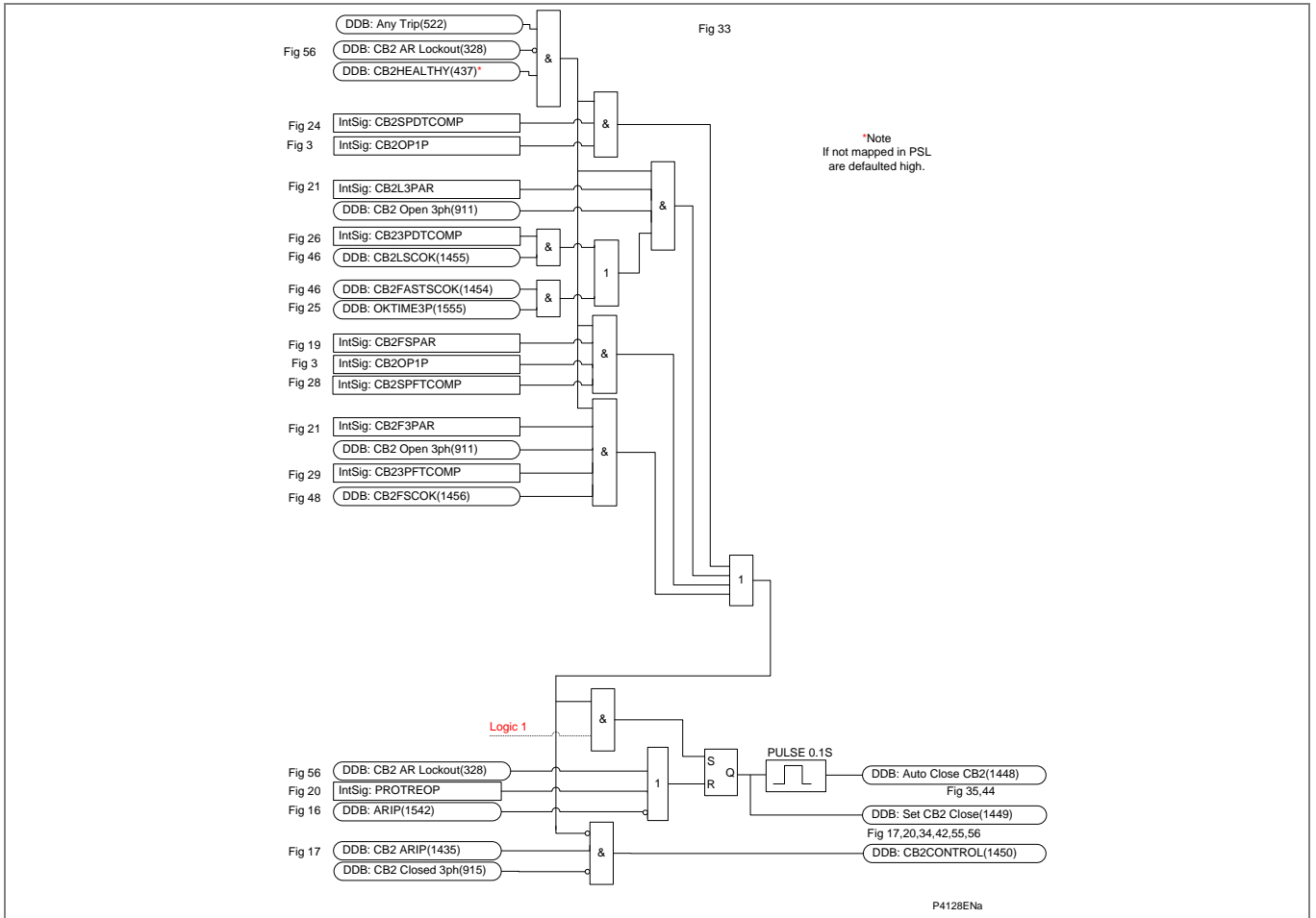
Figure AR-32 - CB2 Auto close
