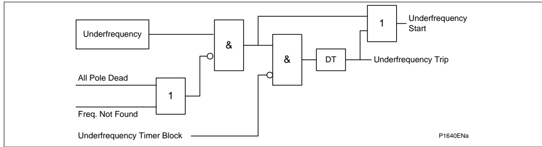
Figure 75 - Underfrequency logic (single stage)
