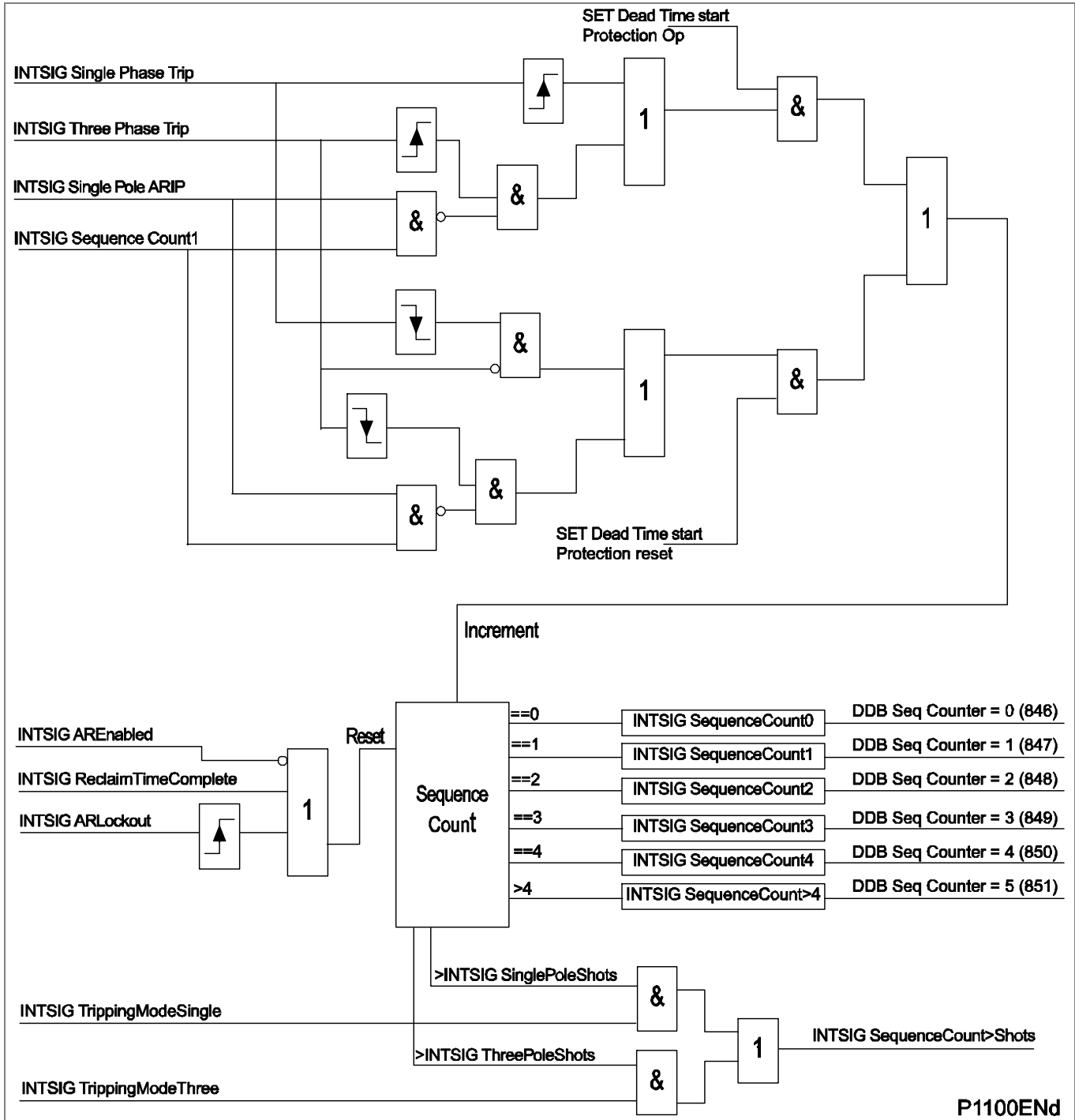
Figure 113 - Auto-reclose inhibit sequence count (P543/P545)
