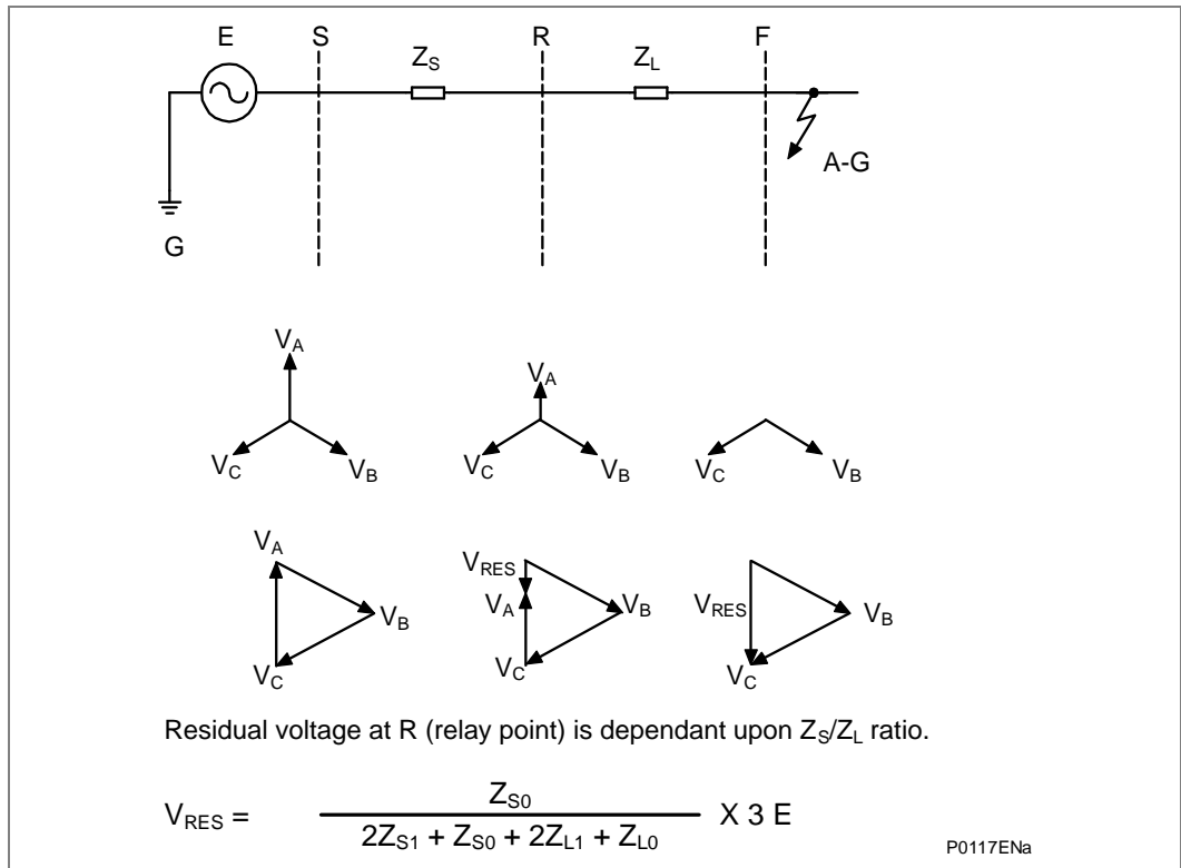
Figure 22 - Residual voltage, solidly earthed system
