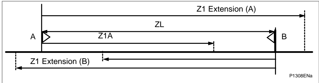
Figure 54 - Zone 1 extension scheme
