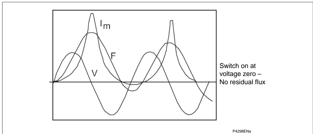
Figure 4 - Magnetizing inrush current during energization
