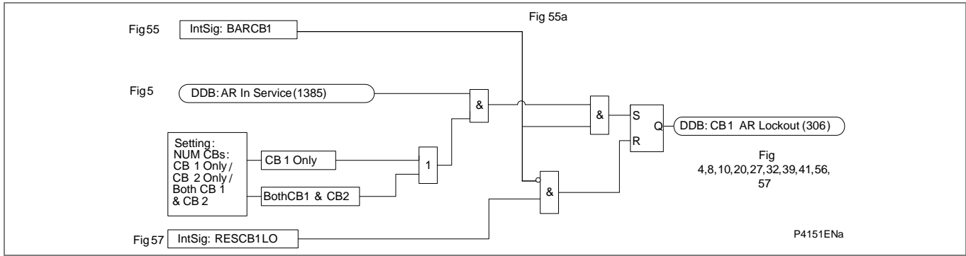
Figure AR-54 - Auto-reclose lockout – CB1
