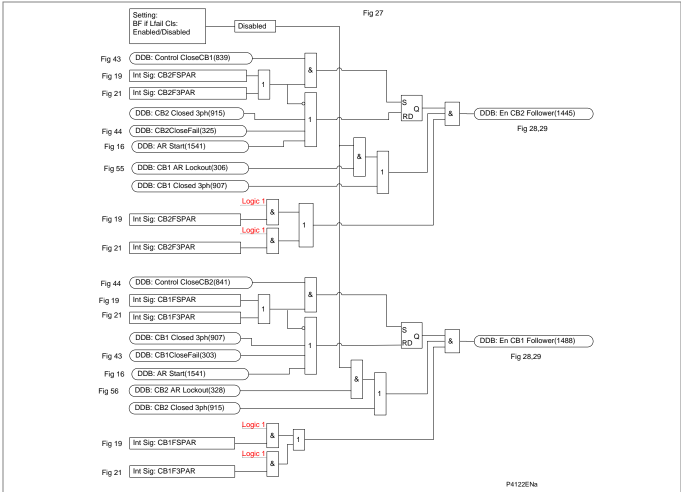
Figure AR-27 - Follower AR enable (for Software Versions BEFORE H1)
