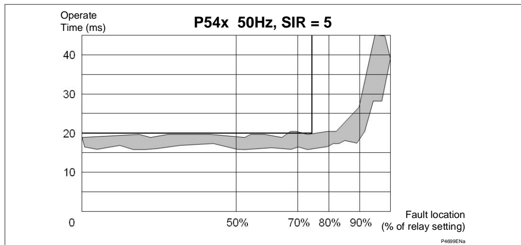
Figure 1 - Operating Time vs Reach % at 50 Hz
