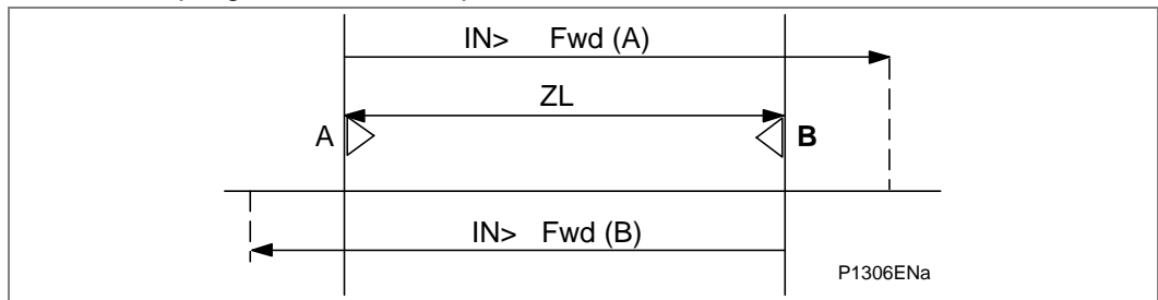
Figure 48 - The DEF permissive scheme (Distance option only)
