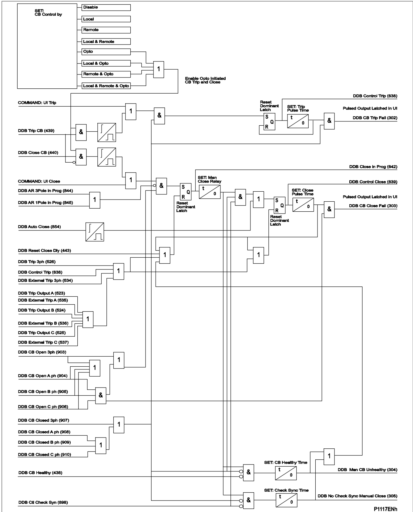
Figure 125 - Circuit breaker control (P543/P545)
