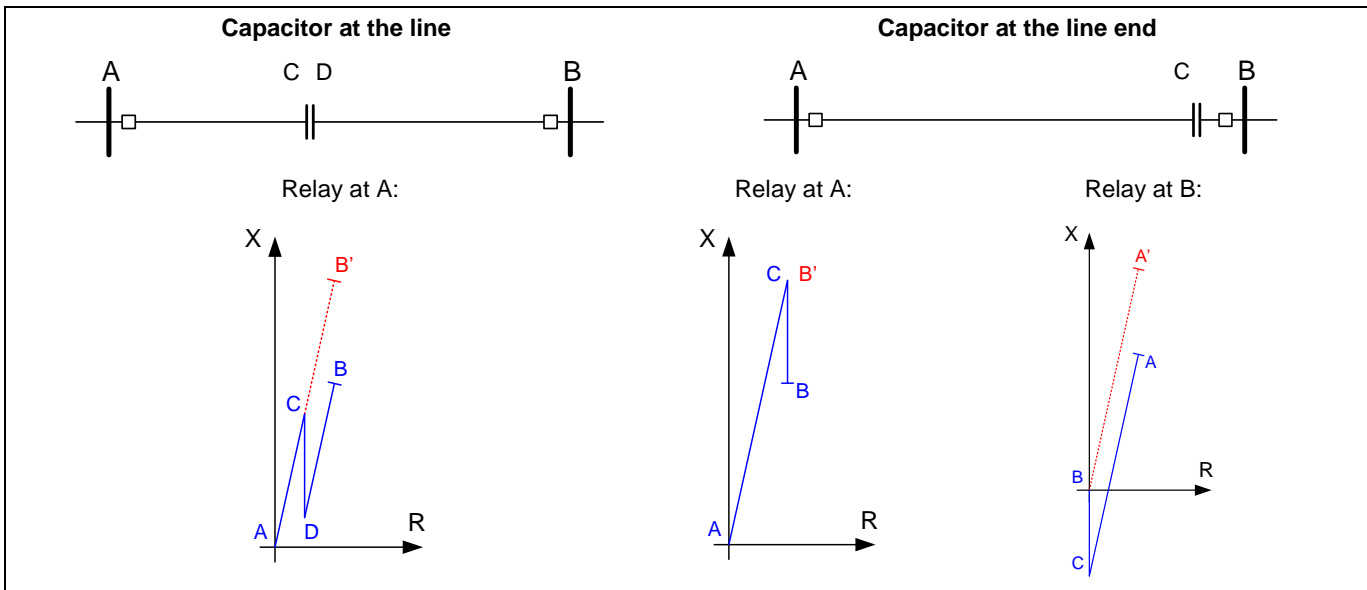
Figure 18 - Effect of series capacitor location to apparent impedance for faults along the line A-B
