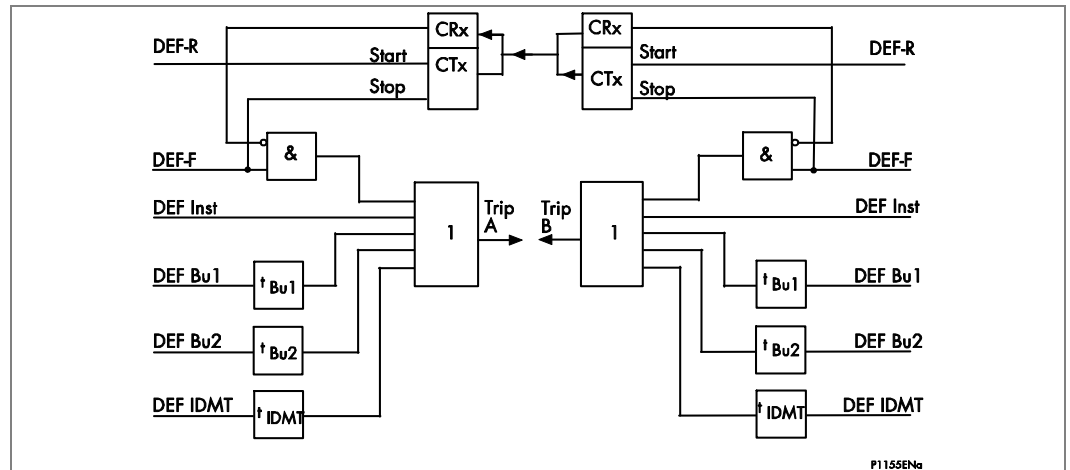
Figure 51 - Aided DEF (ground) blocking scheme logic (Distance option only)
