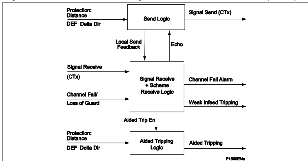
Figure 36 - Aided scheme logic overview (Distance option only)
