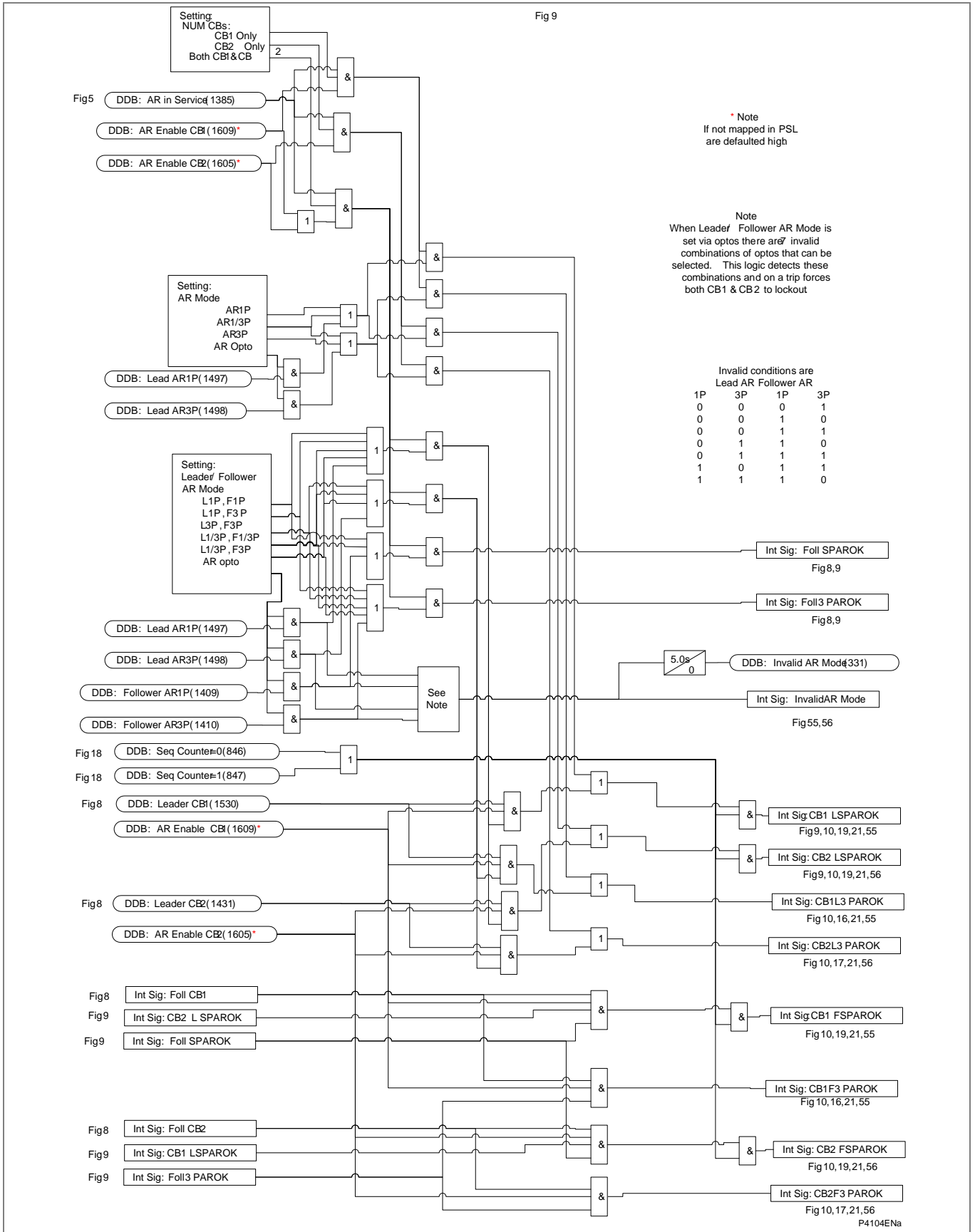
Figure AR-10 - Leader & follower AR modes enable
