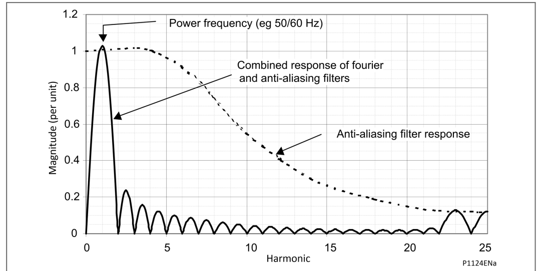
Figure 9 - Frequency response (for P14x, P24x, P341, P34x and P64x) diagram
