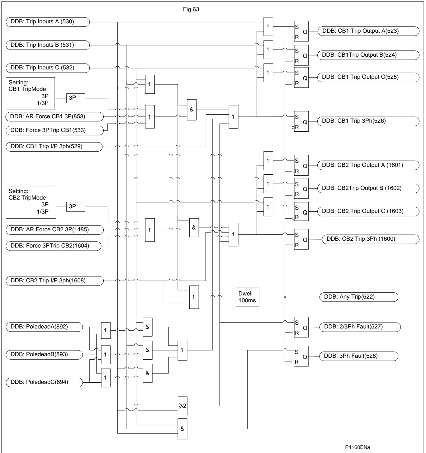
Figure AR-65 - CB trip conversion
