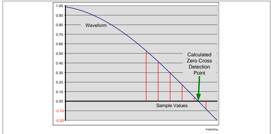
Figure 71 - Calculating a Zero Cross Detection Point using sample values
