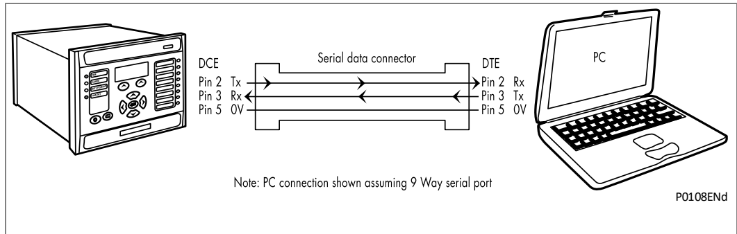
Figure 9 - PC relay signal connection
