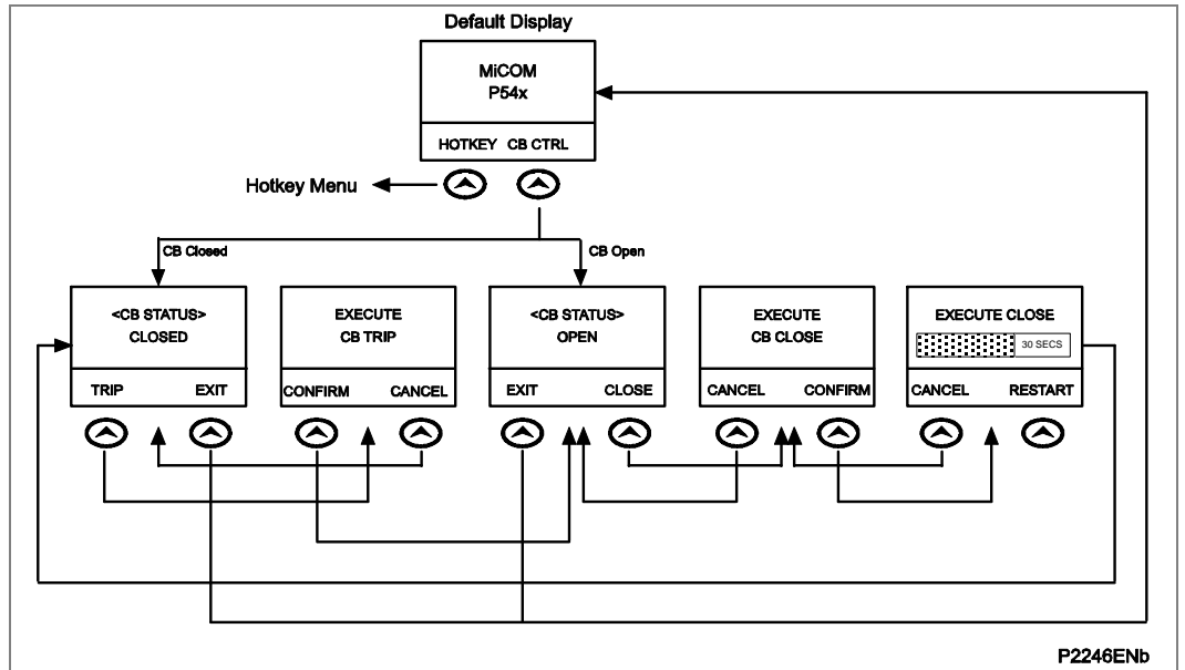
Figure 126 - CB control hotkey menu
