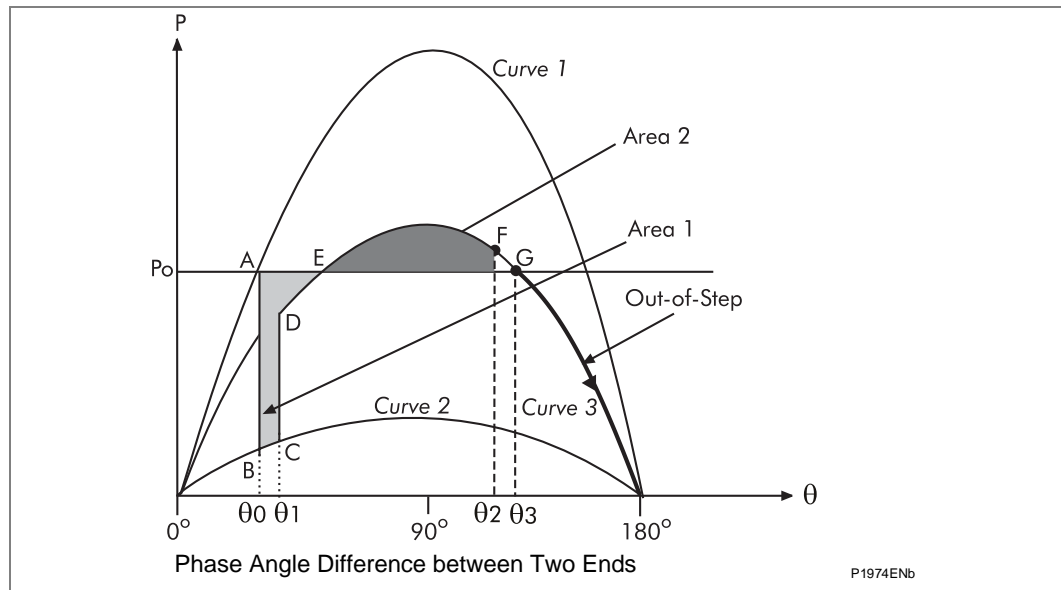
Figure 13 - Power transfer in relation to angle difference \theta between 2 ends
