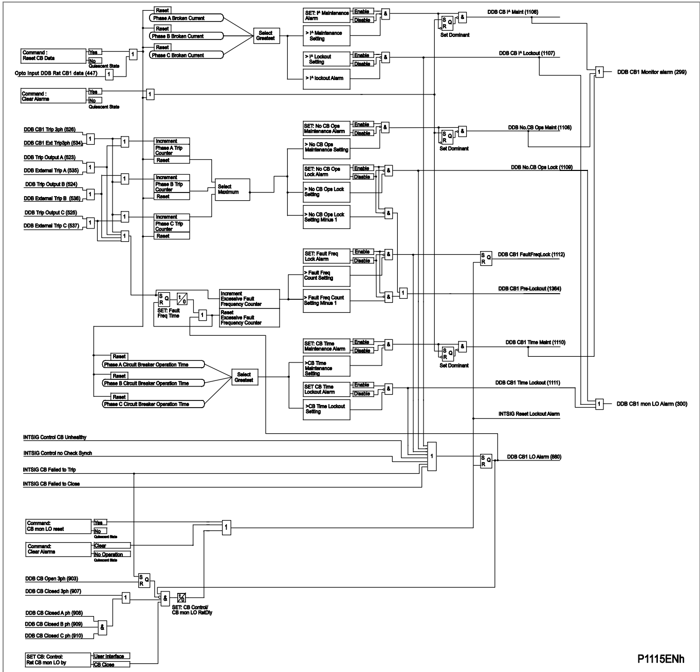
Figure 132 - Circuit breaker 1 – monitoring
