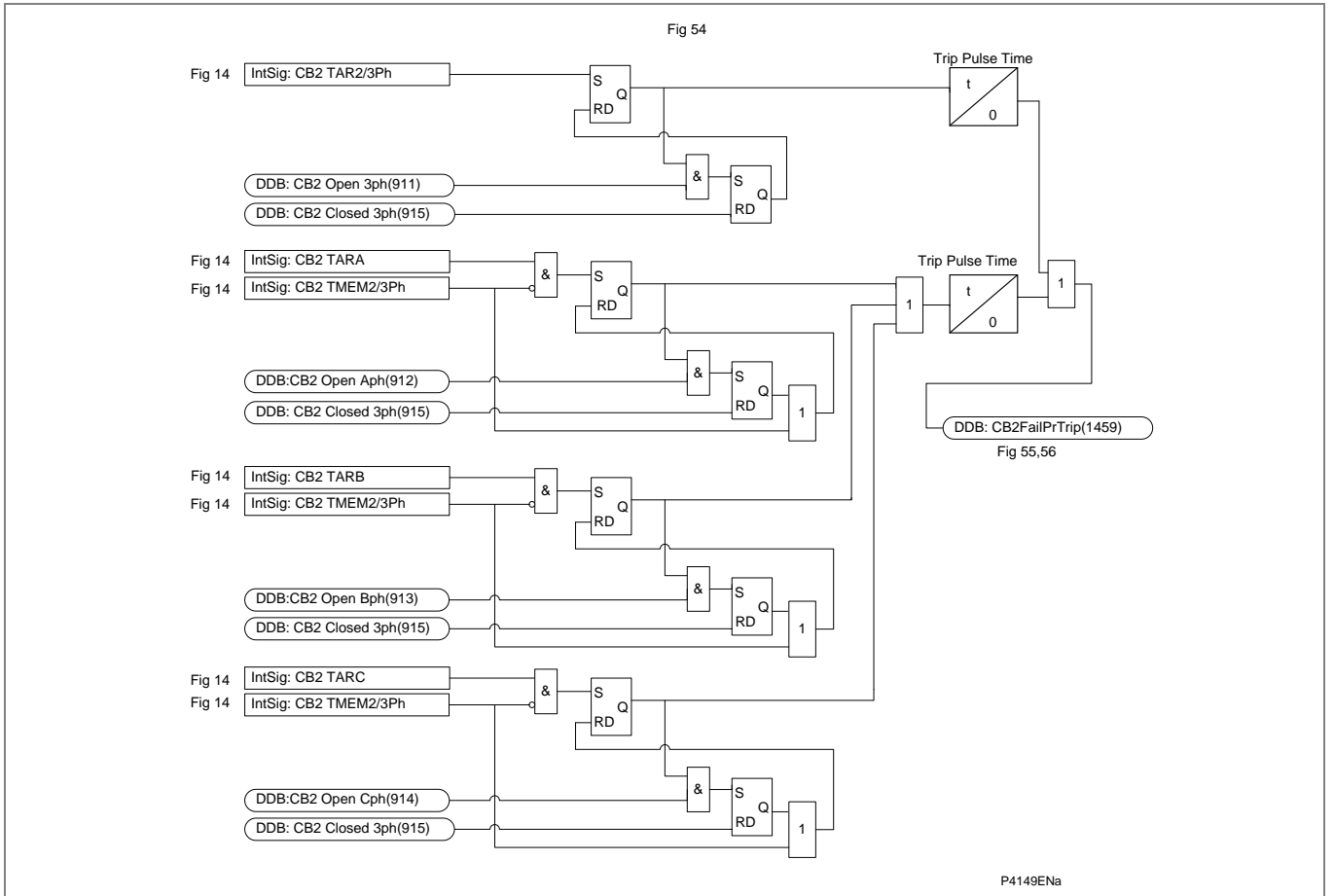
Figure AR-51 - CB2 trip time monitor
