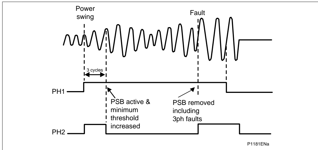
Figure 29 - Power swing detected for 3 cycles continuous \Delta I (Distance option only)
