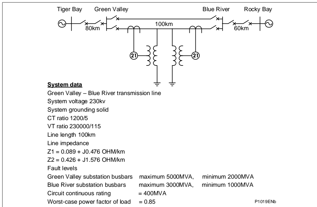
Figure 28 - System assumed for worked example
