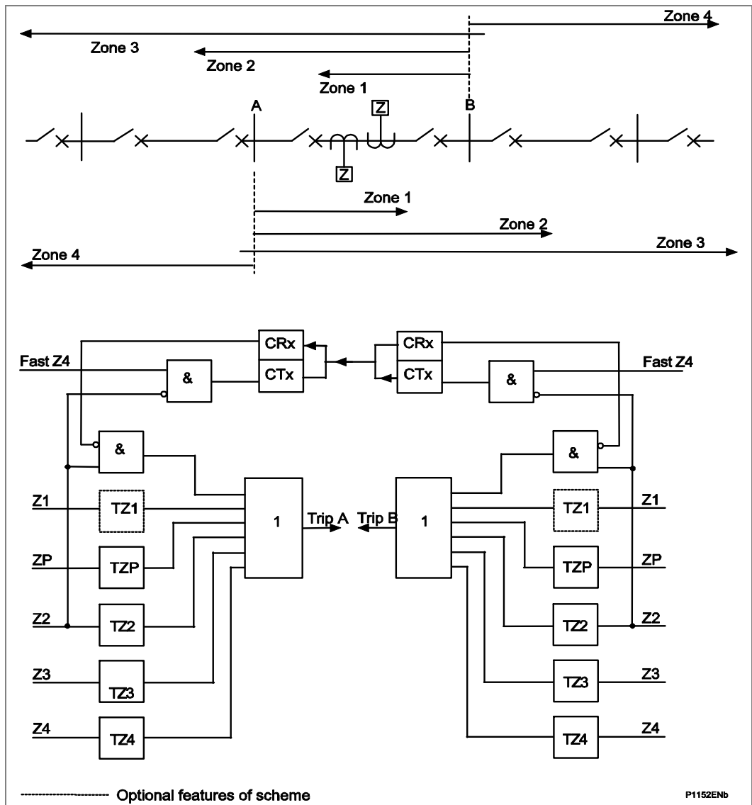
Figure 44 - Distance blocking scheme (BOP) (Distance option only)
