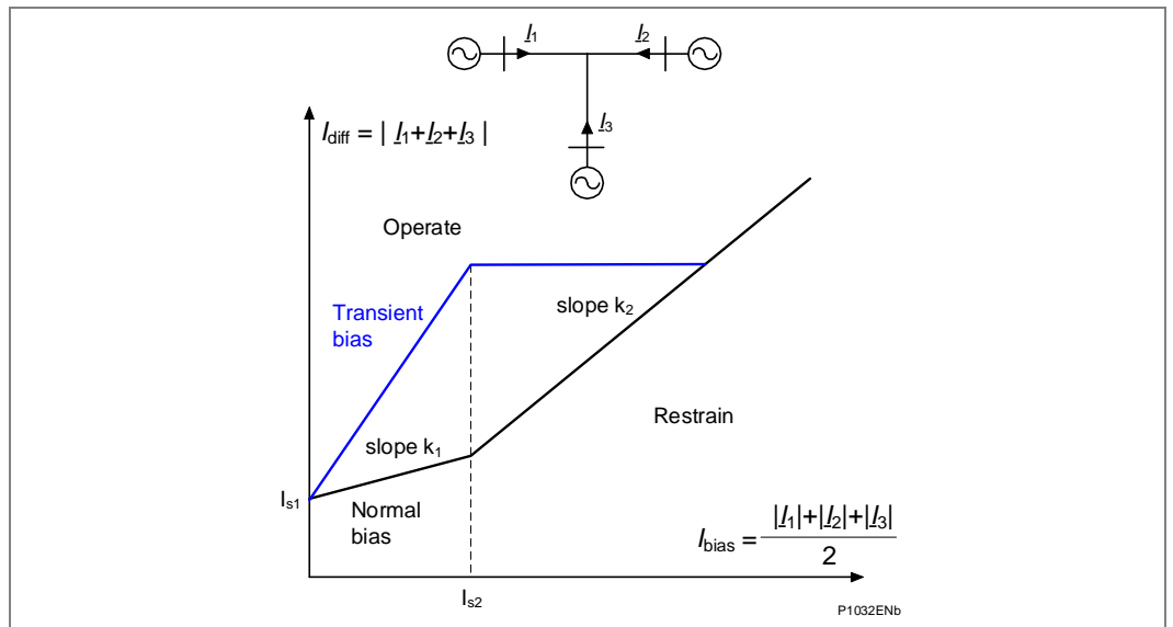
Figure 87 - Transient bias characteristic
