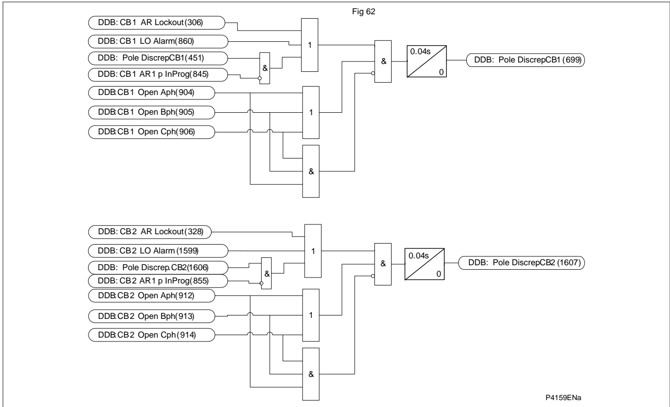
Figure AR-63 - Pole discrepancy (for P54x except P546)
