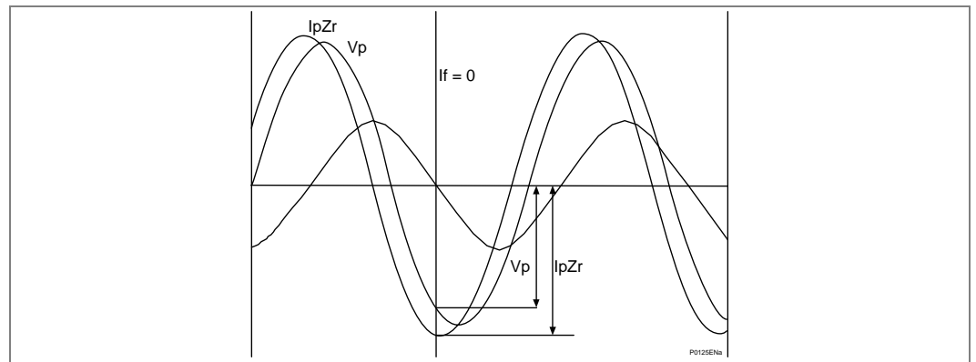
Figure 106 - Fault locator selection of fault current zero
