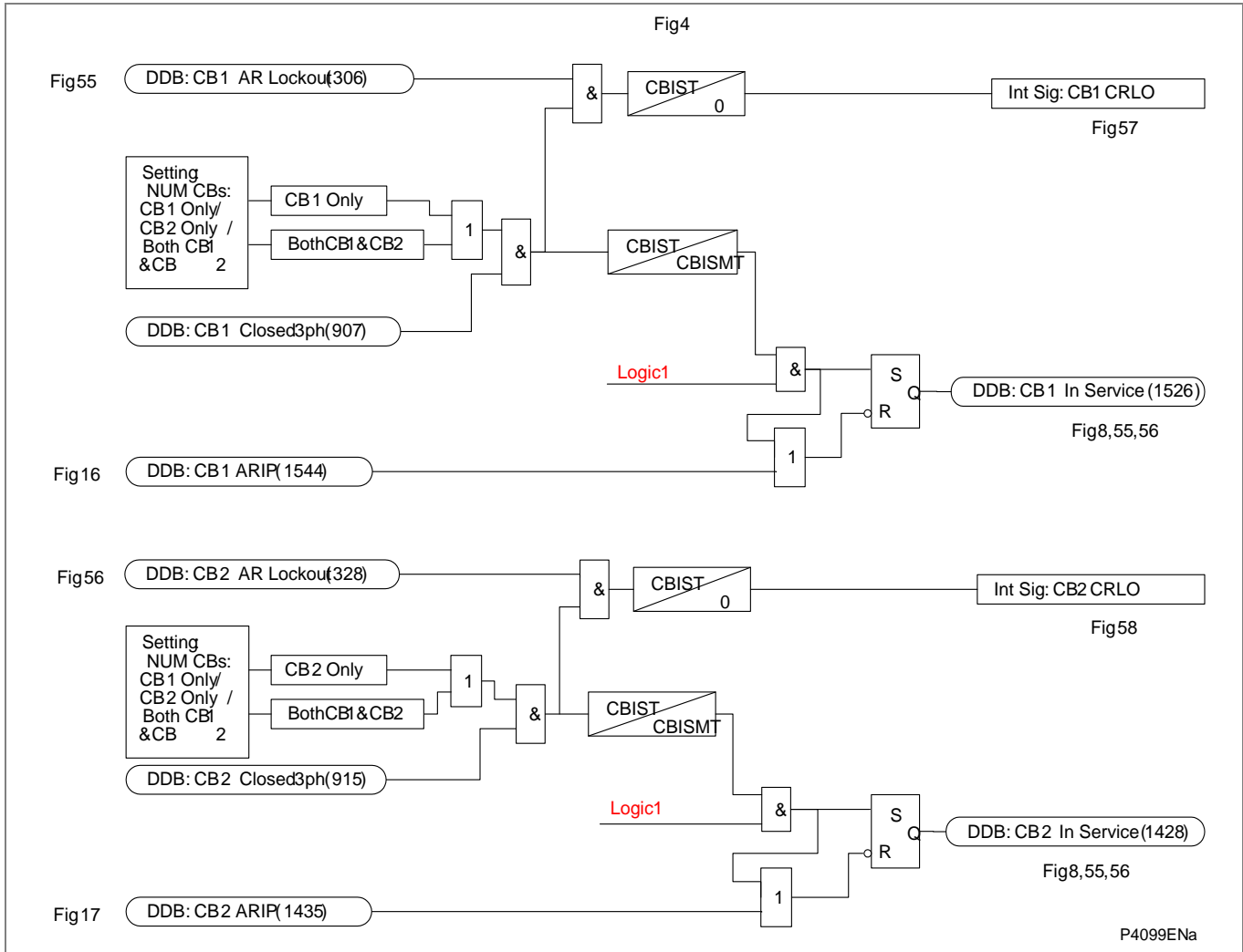
Figure AR-4 - Circuit breaker in service
