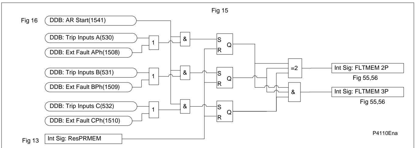
Figure AR-16 - 1Ph, 2Ph & 3Ph fault memory
