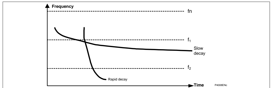
Figure 77 - Rate of change of frequency protection
