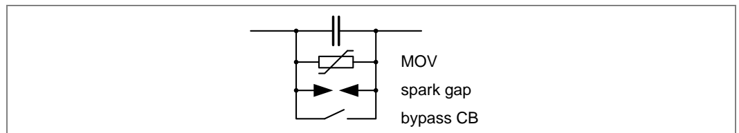
Figure 17 - Overvoltage protection for series compensation (simplified)
