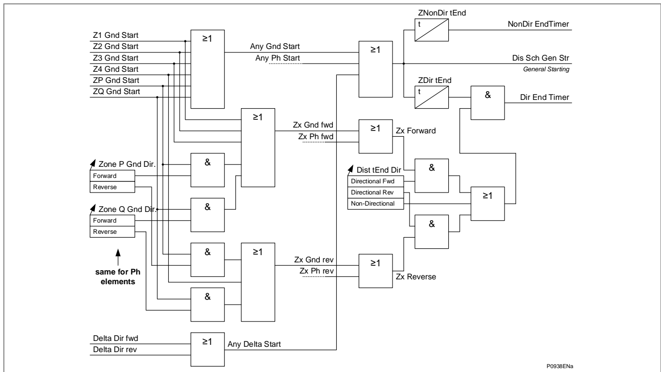
Figure 20 - General starting logic and end timers
