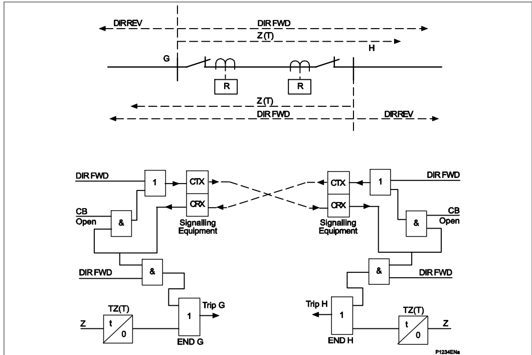
Figure 52 - Delta directional comparison POR scheme (Distance option only)
