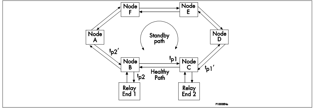
Figure 4 - Example of switched synchronous digital hierarchy
