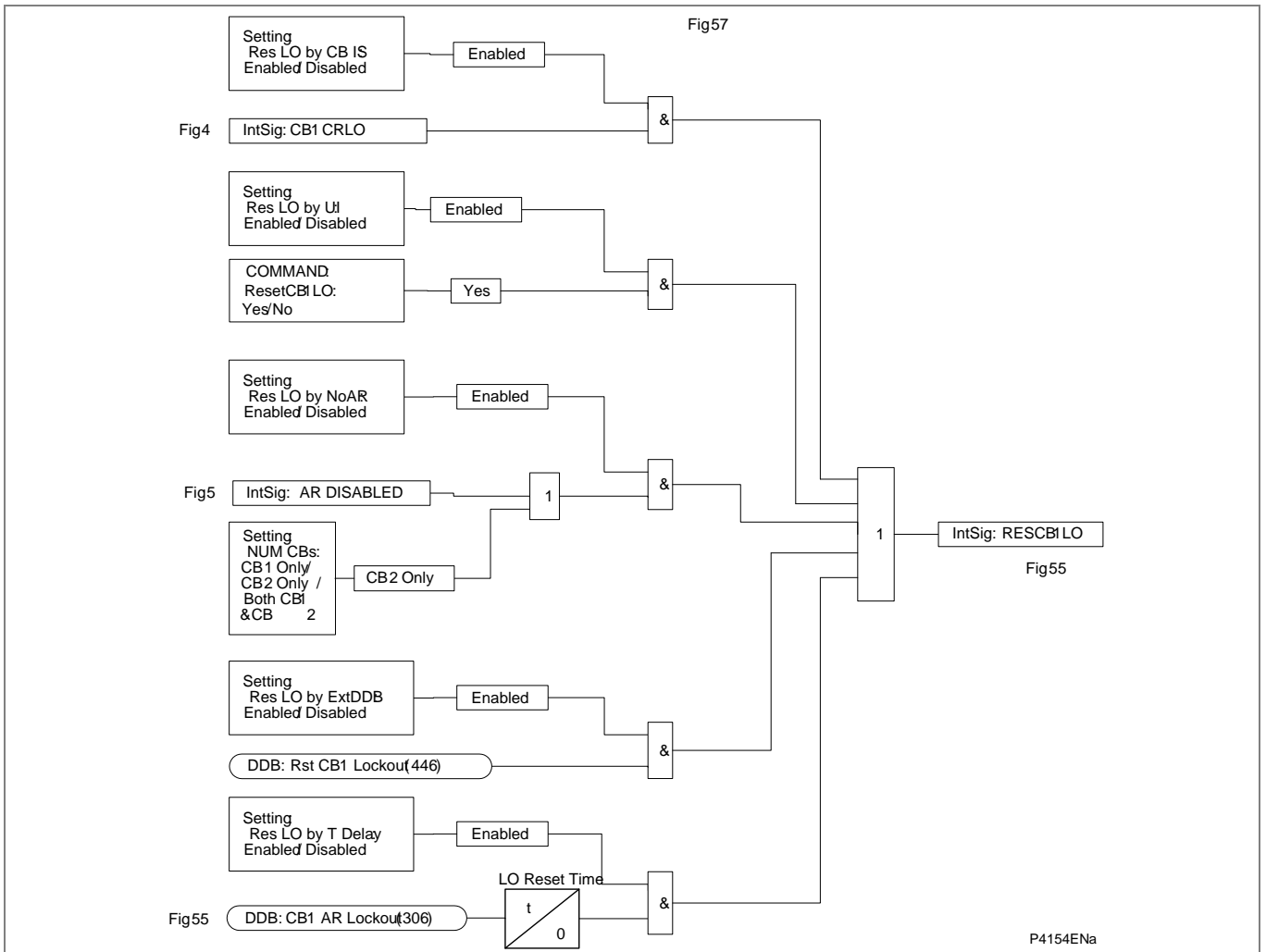
Figure AR-58 - Reset CB1 lockout
