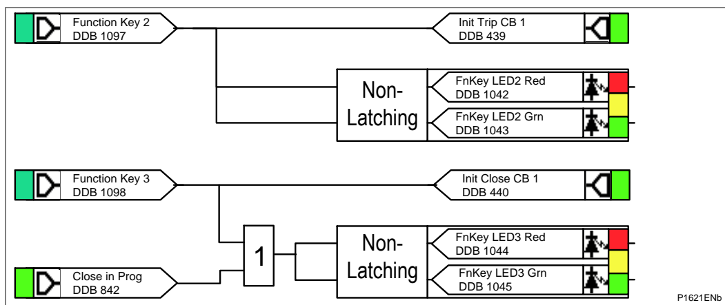
Figure 127 - CB control via function keys default PSL
