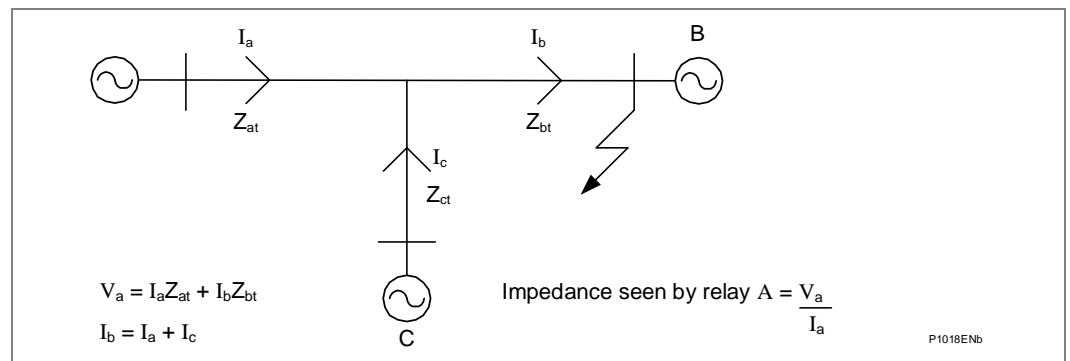
Figure 29 - Teed feeder application - apparent impedances seen by relay
