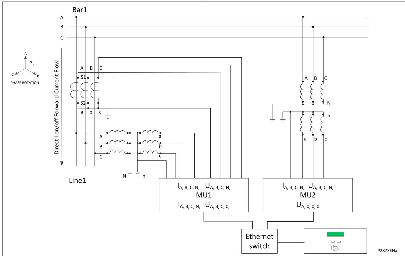
Figure 26 - Connection
