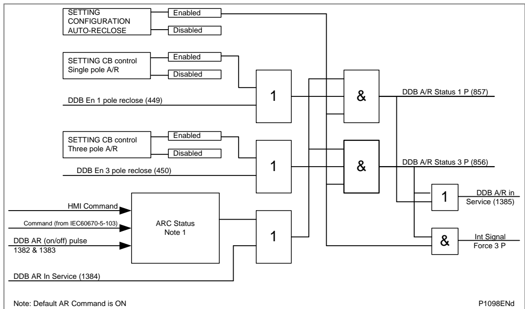
Figure 111 - Auto-reclose enable logic
