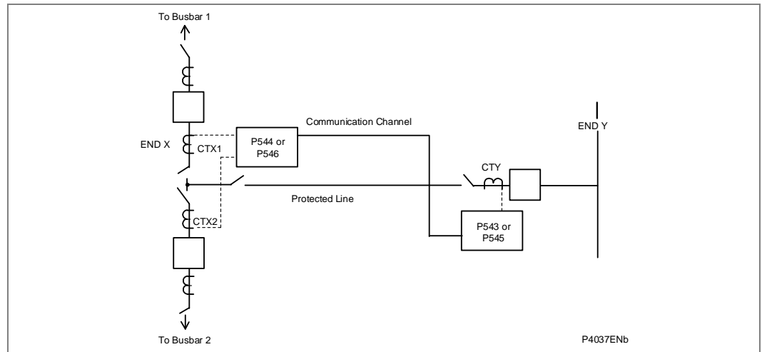
Figure 13 - Breaker and a half application
