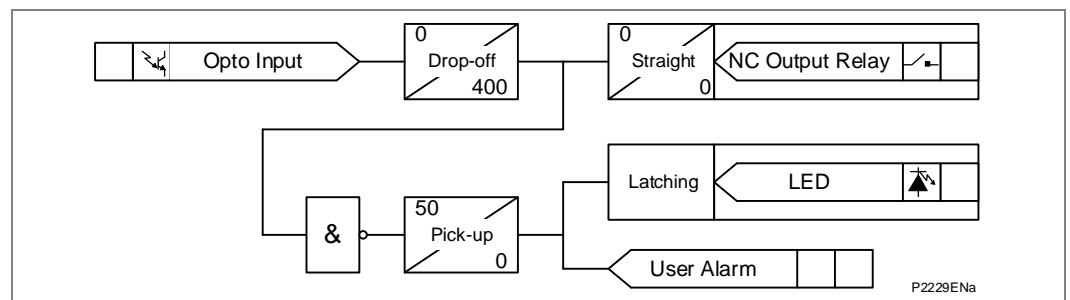
Figure 32 - PSL for TCS schemes 1 and 3
