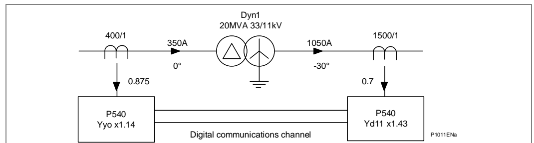
Figure 25 - Typical transformer feeder circuit
