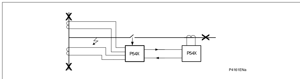
Figure 14 - Stub bus protection
