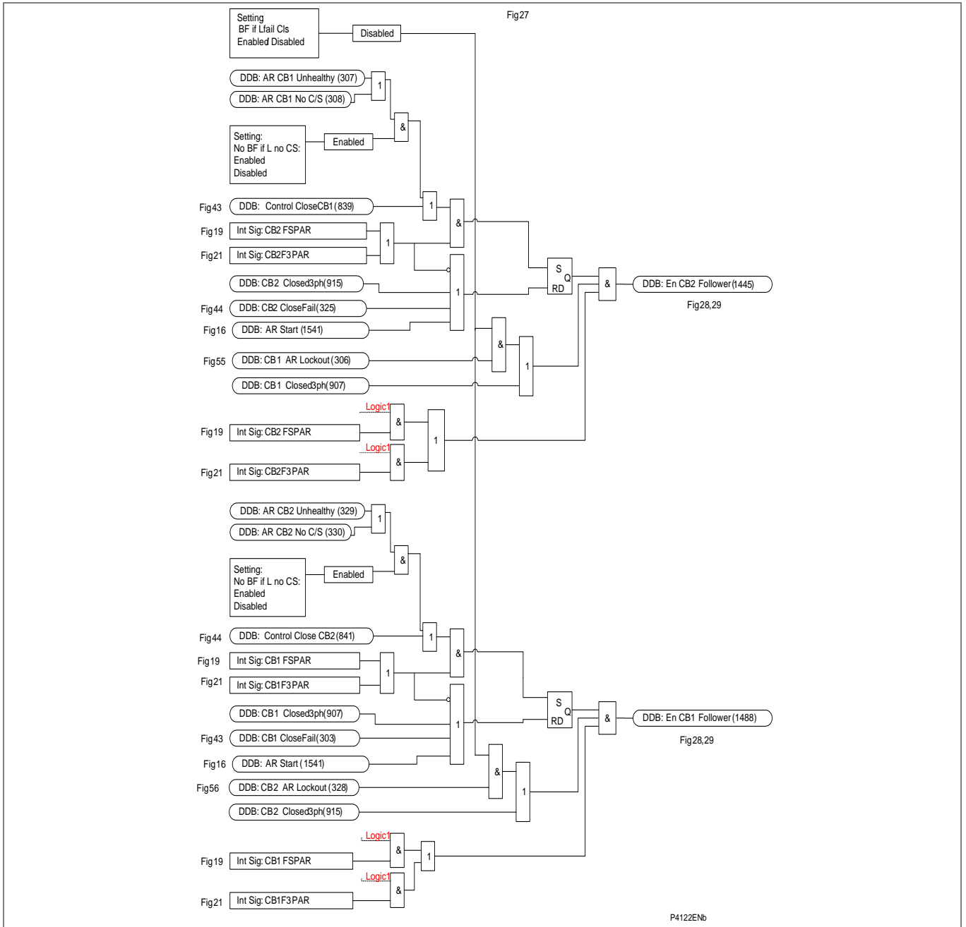
Figure AR-28 - Follower AR enable (for Software Versions H1 and later)
