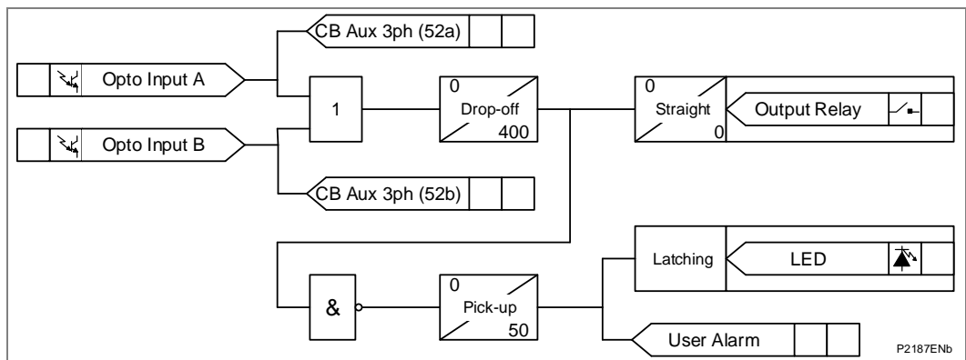
Figure 34 - PSL for TCS schemes 2a
