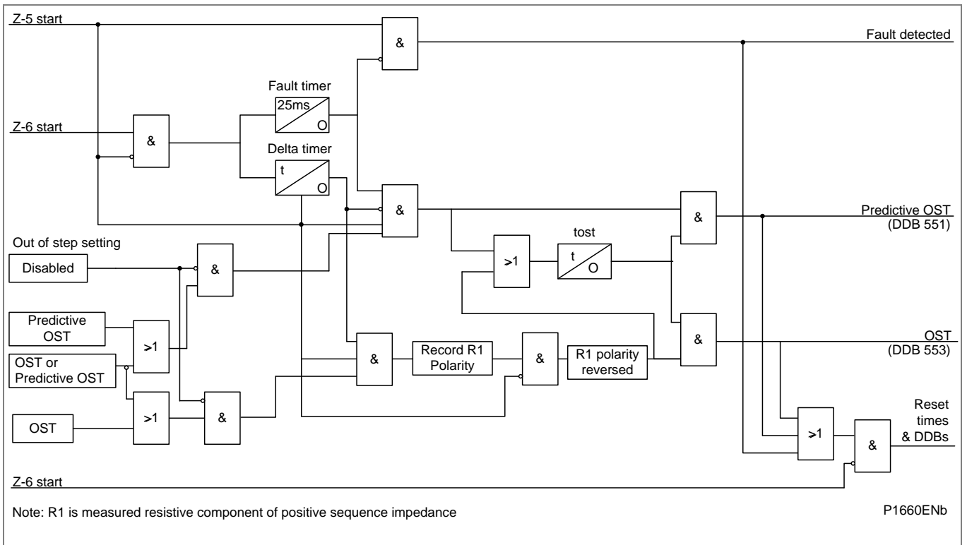
Figure 32 - Out of step algorithm (Distance option only)
