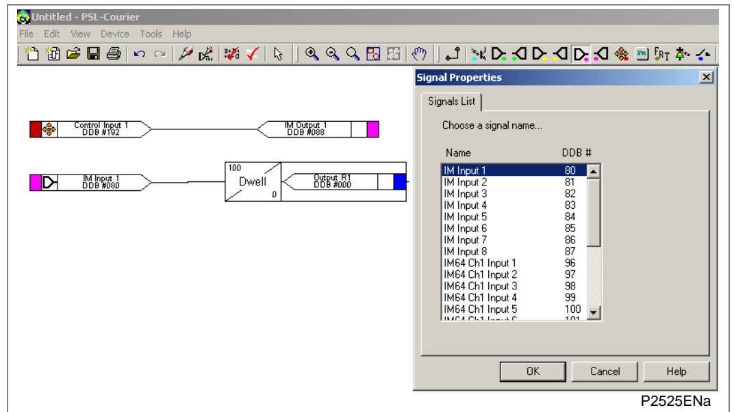
Figure 96 - Example assignment of signals within the PSL
