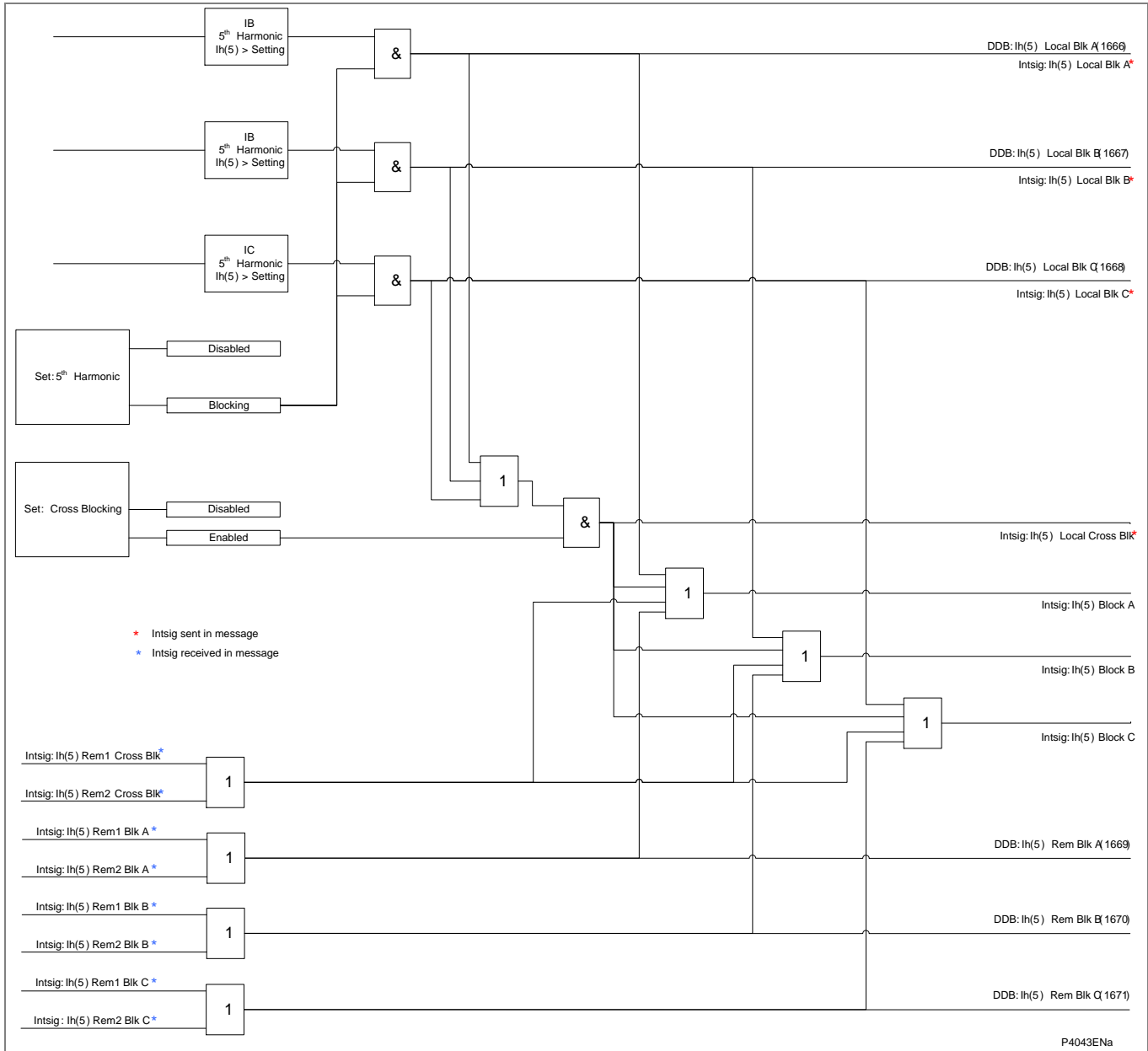
Figure 10 - Fifth harmonic blocking logic
