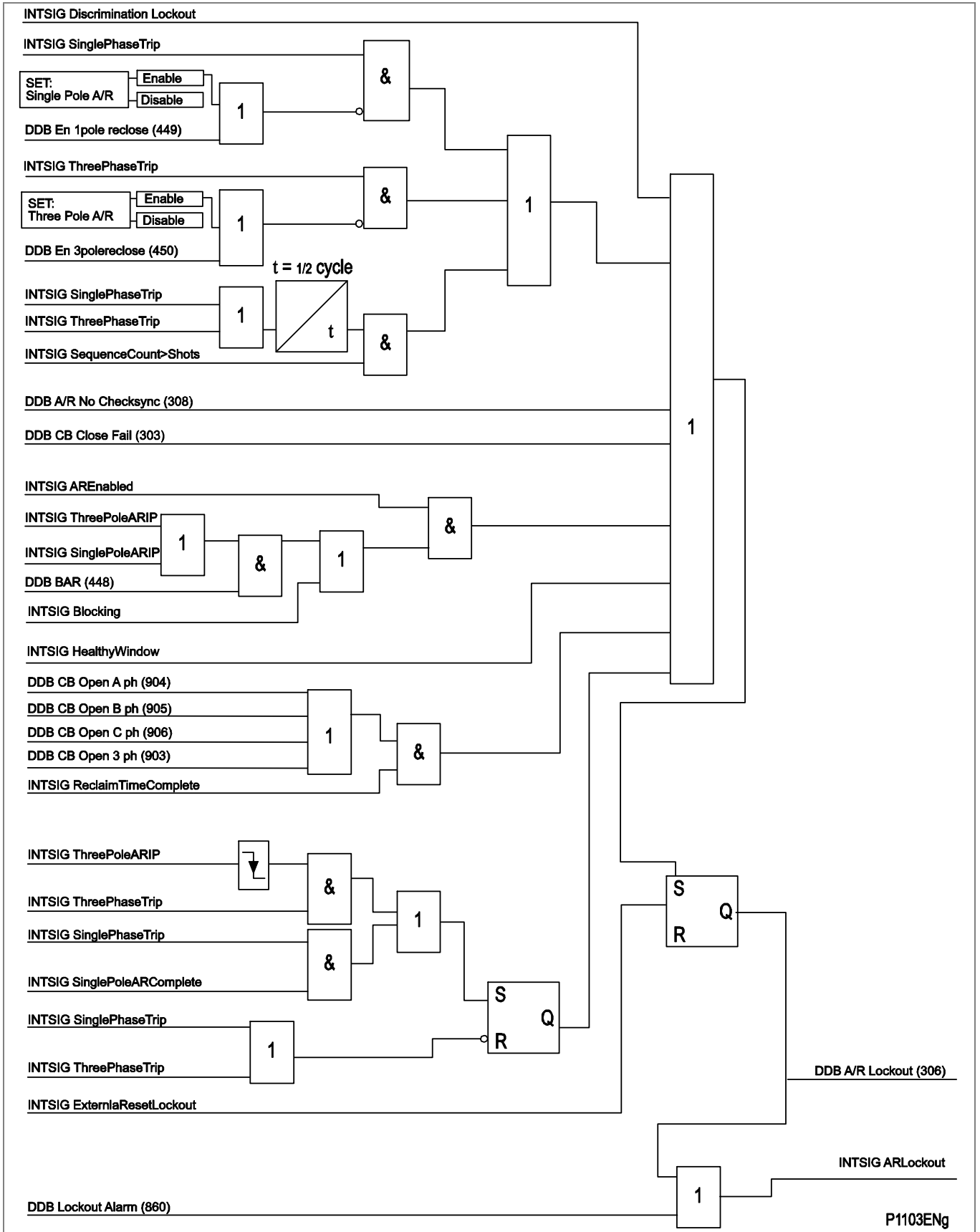
Figure 116 - Auto-reclose lockout logic (P543/P545)
