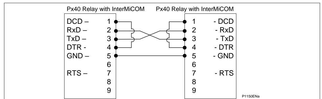
Figure 92 - Direct connection within the local substation
