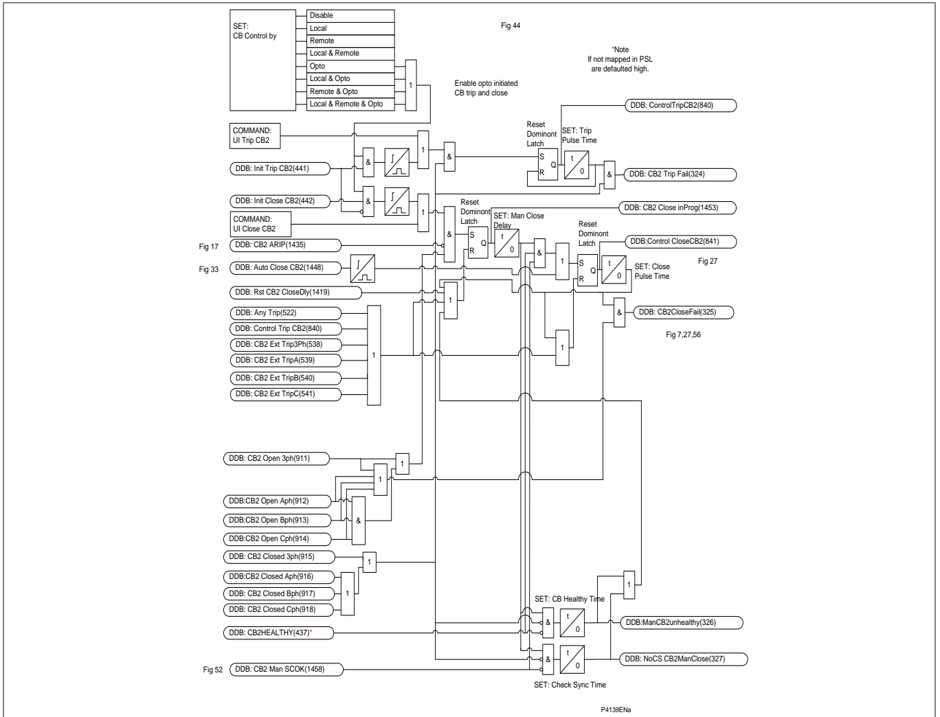
Figure AR-43 - CB2 circuit breaker control
