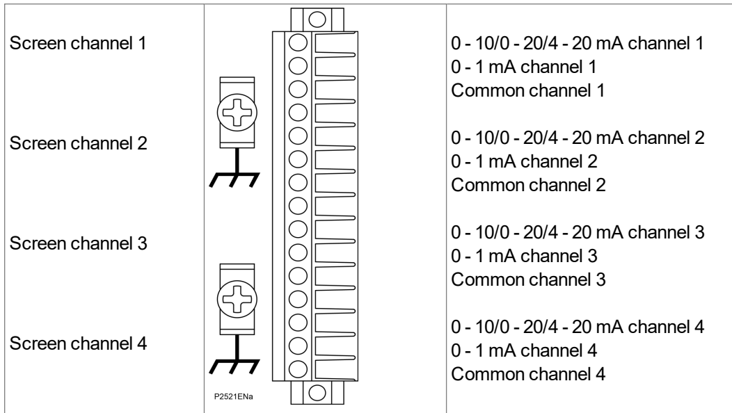
Figure 5 - Current loop input output board diagram
