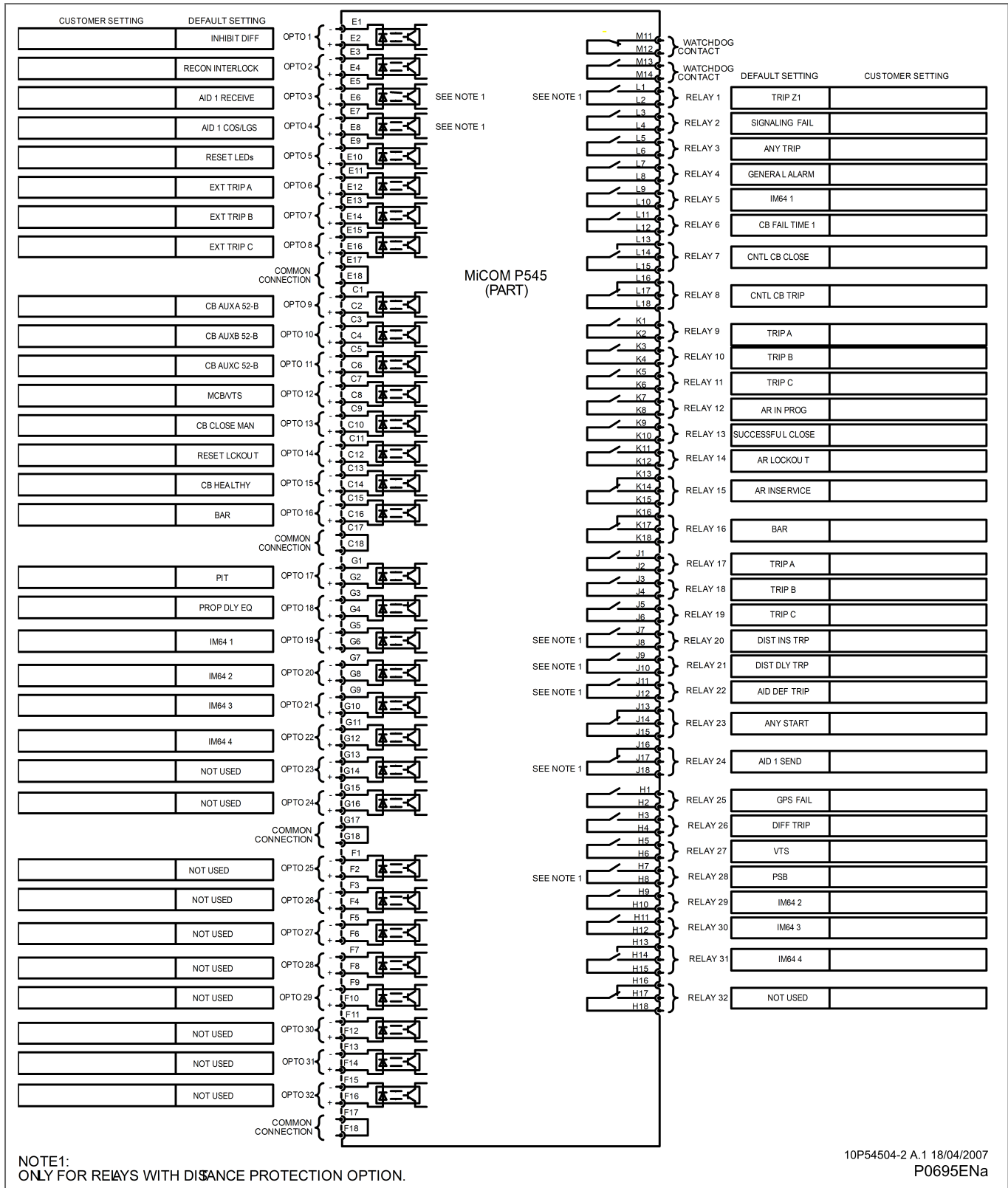
Figure 19 - P545 - 32 optos, 32 relays, Distance, 1 or 3 Pole Tripping, Auto-Reclose and Chk Sync Sheet 2
