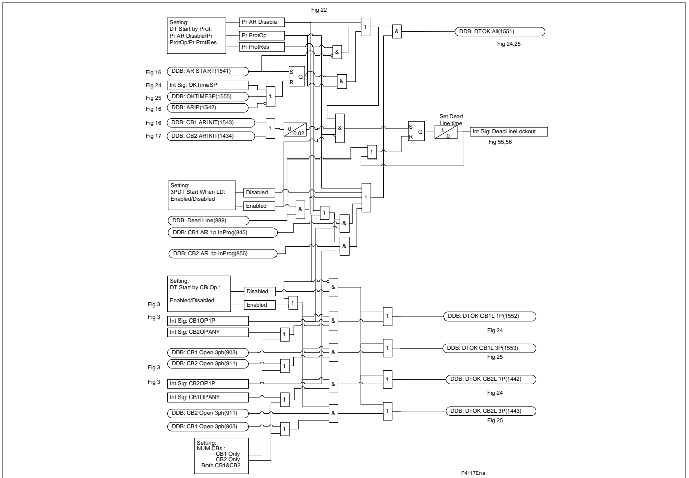
Figure AR-23 - Dead time start enable
