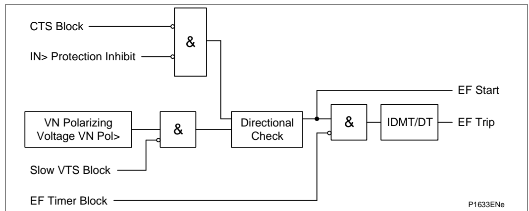
Figure 63 - Directional EF with neutral voltage polarization (single stage)
