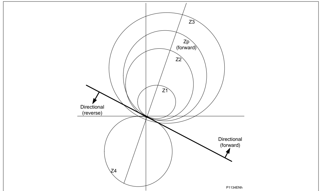
Figure 18 - Phase fault Mho characteristics (Distance option only)
