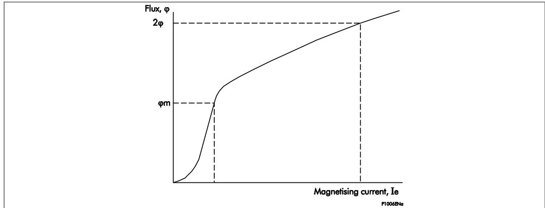
Figure 7 - Transformer magnetizing characteristic
