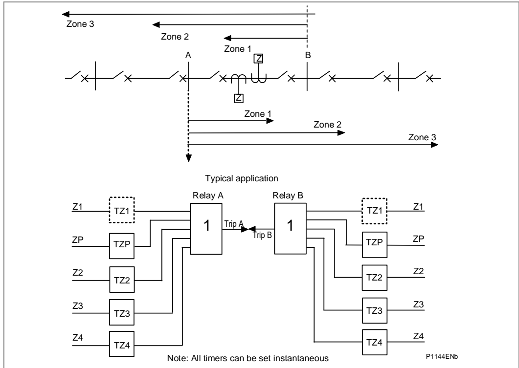
Figure 12 - Basic time stepped distance scheme
