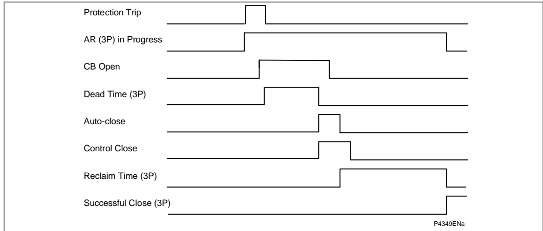
Figure 136 - Auto-reclose timing diagram – single breaker, single fault
