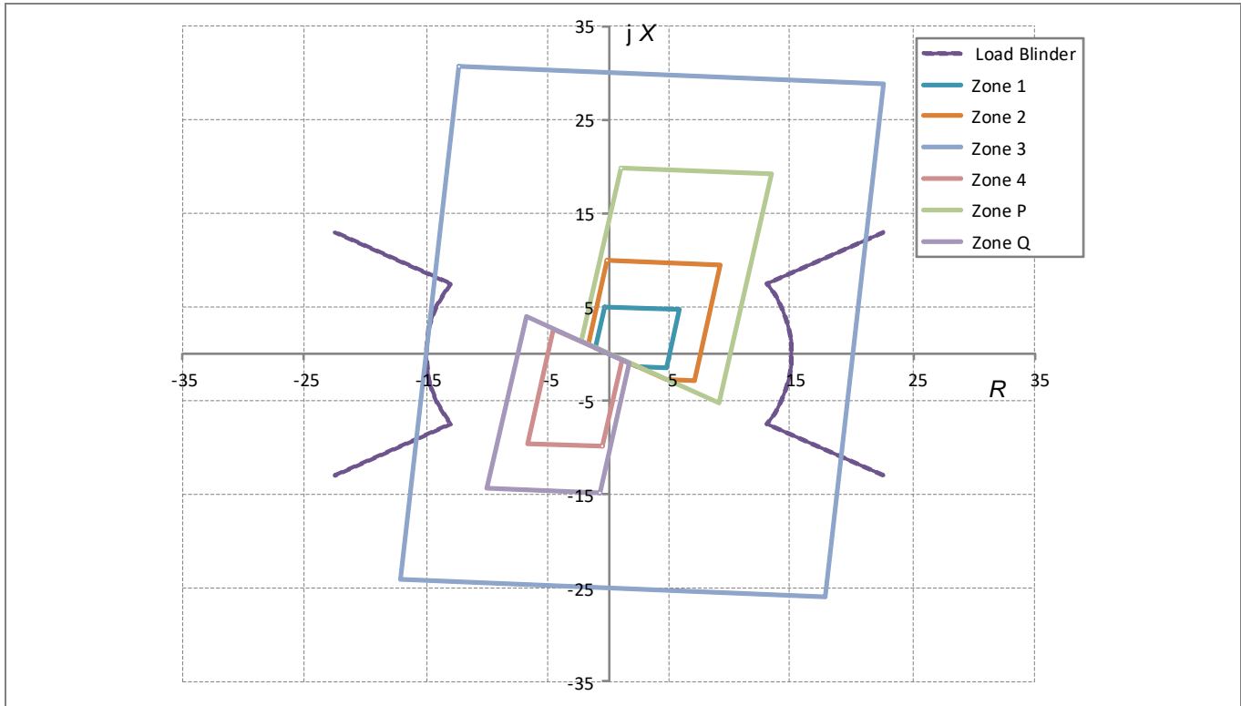
Figure 8 - Zone reach setting with load blinders and underimpedance starting for application example
