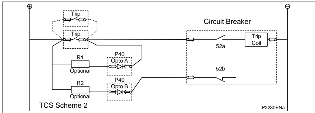
Figure 33 - TCS scheme 2a
