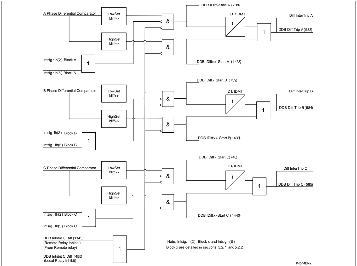
Figure 11 - Highset element logic
