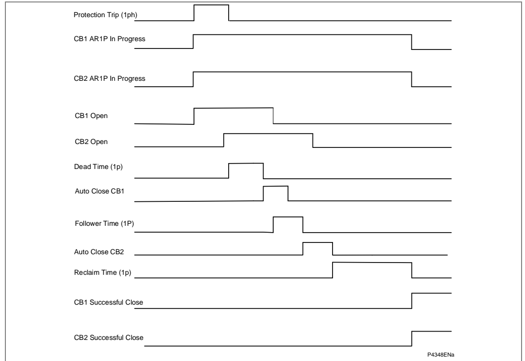
Figure 138 - Auto-reclose timing diagram leader/follower (1ph)
