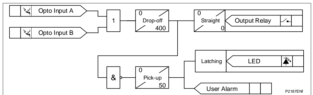
Figure 36 - PSL for TCS schemes 2b
