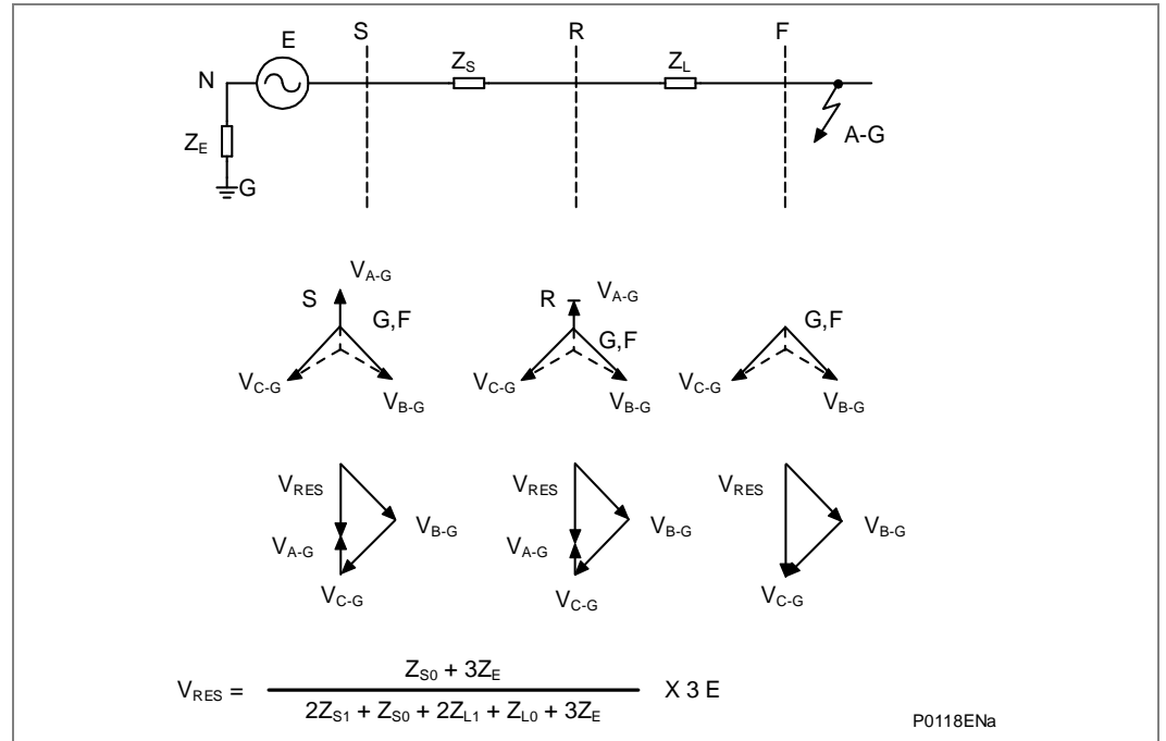
Figure 23 - Residual voltage, resistance earthed system
