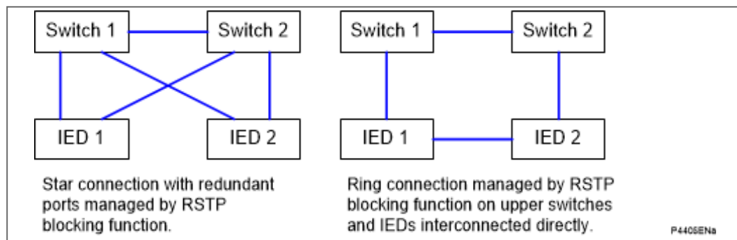
Figure 1 - Px4x attached to a redundant Ethernet star or ring circuit
