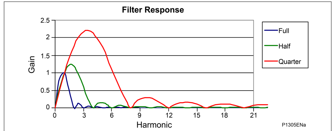
Figure 10 - Frequency response (for P44y, P54x and P445) diagram
