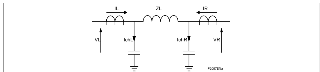
Figure 6 - Capacitive charging current
