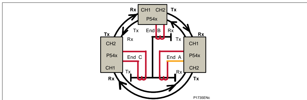
Figure 97 - Triangulated InterMiCOM64 application
