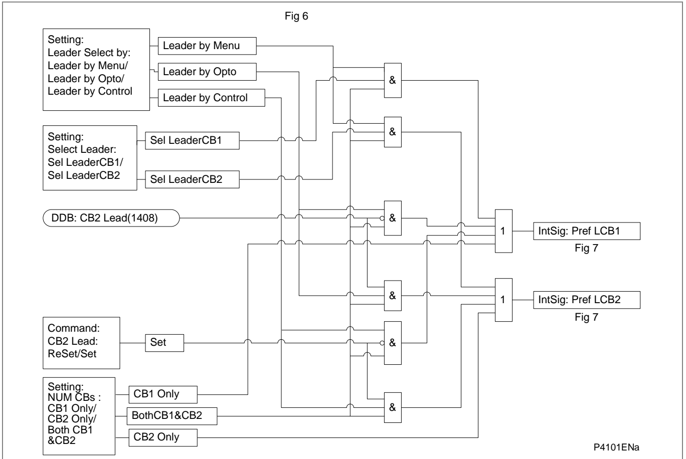
Figure AR-6 - Lead & follower circuit breaker selection
