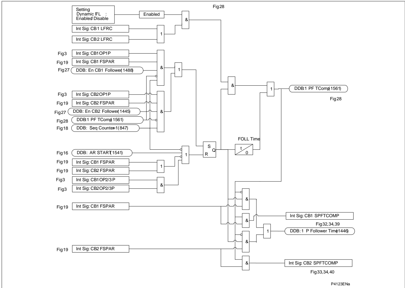
Figure AR-29 - Single phase follower time
