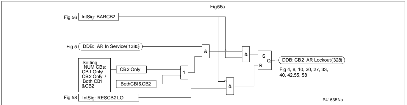
Figure AR-57 - Auto-reclose lockout – CB2
