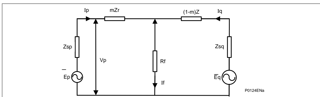
Figure 105 - Two-machine equivalent circuit
