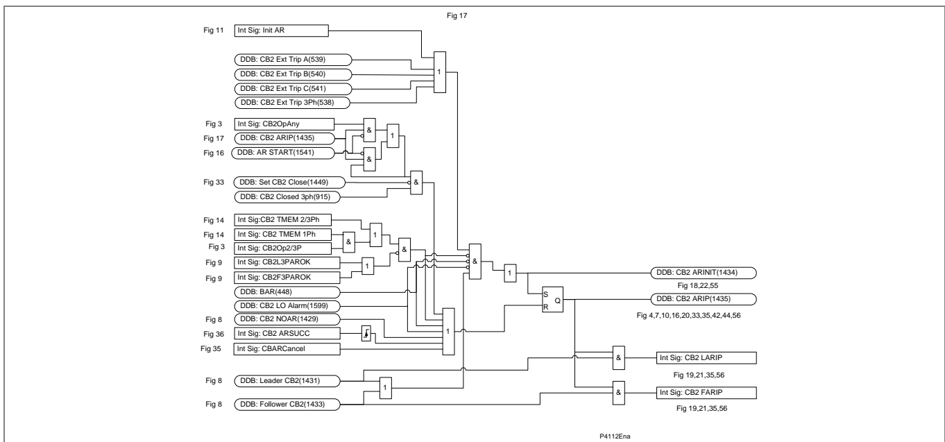
Figure AR-18 - CB2 Auto-reclose in progress
