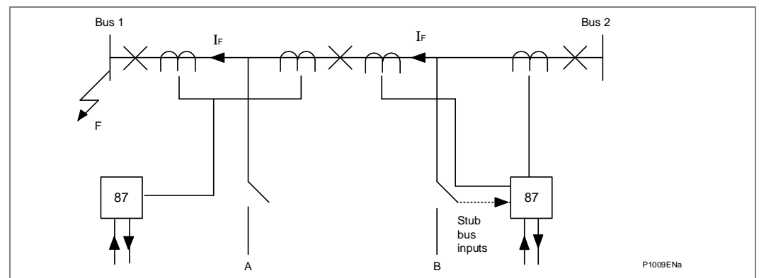
Figure 7 - Breaker and a half switched substation
