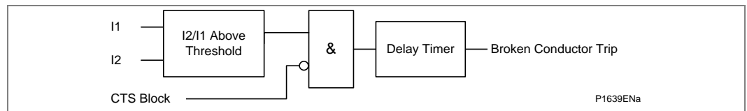
Figure 74 - Broken conductor logic
