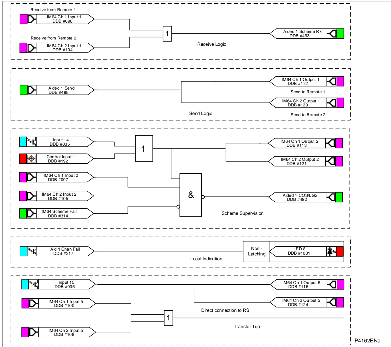
Figure 38 - InterMiCOM 64 mapping in a three ended application
