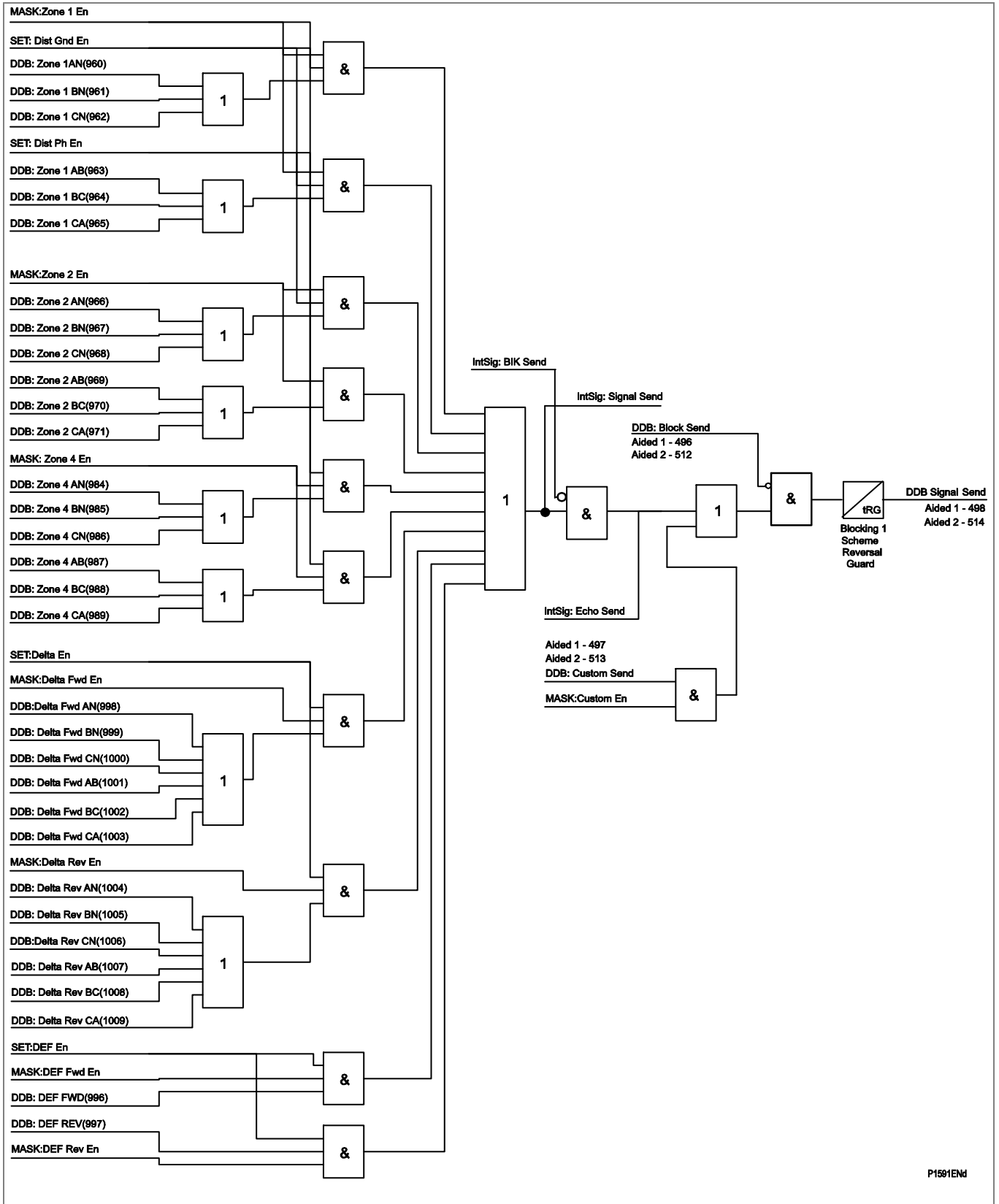
Figure 37 - Send logic (Distance option only)
