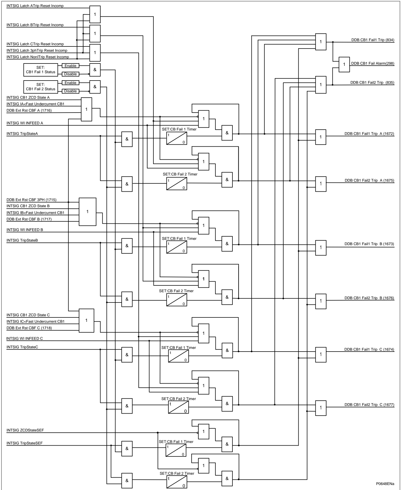
Figure 73 - CB Failure CB1 logic part 2
