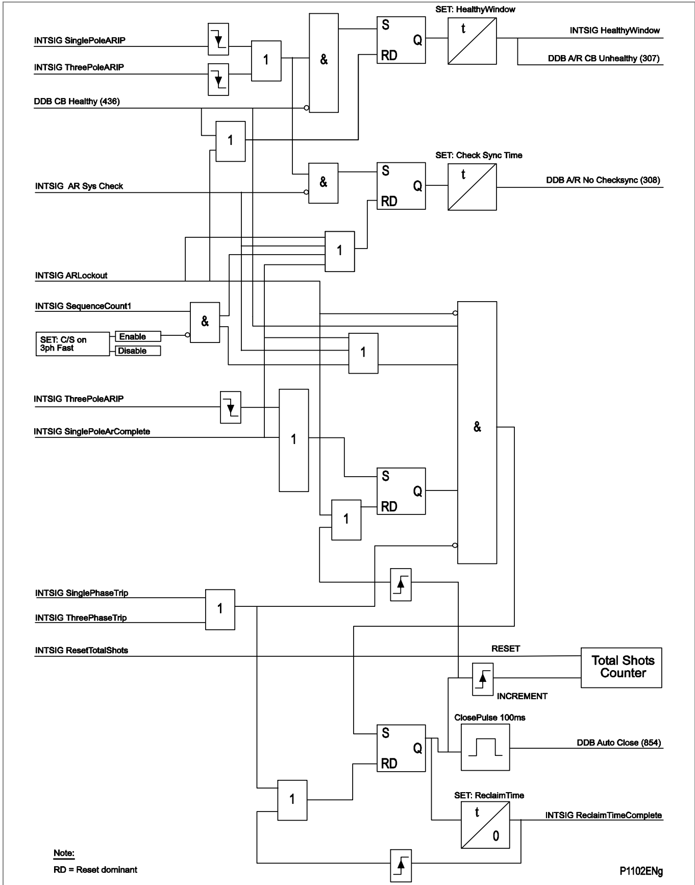
Figure 115 - Auto-reclose close
