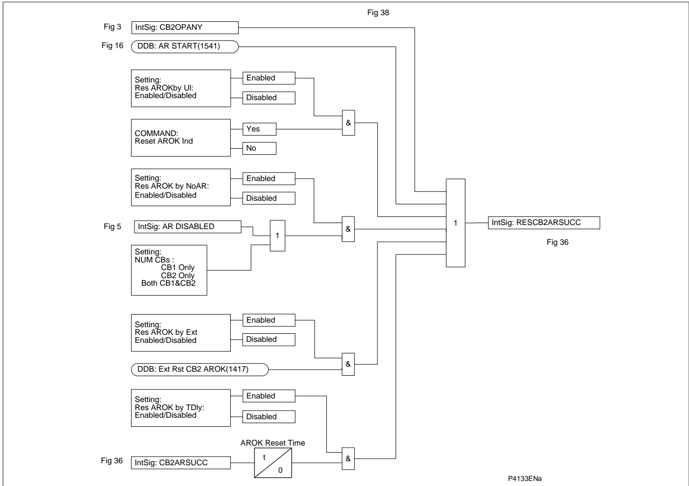
Figure AR-37 - Reset CB2 successful AR indication
