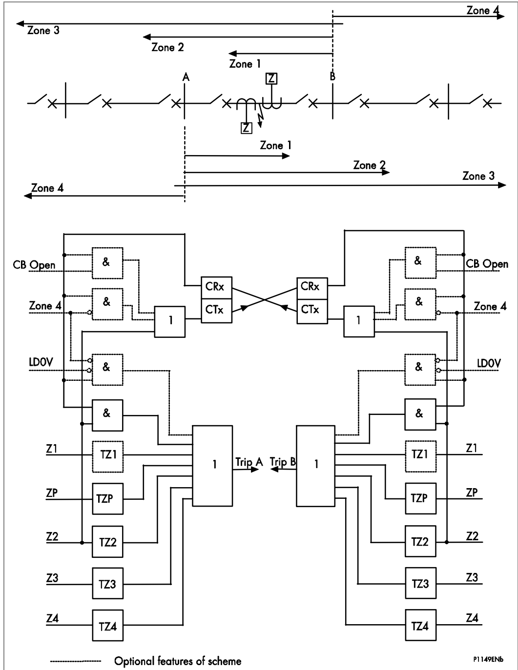
Figure 42 - Permissive overreach transfer trip scheme (POR) (Distance option only)
