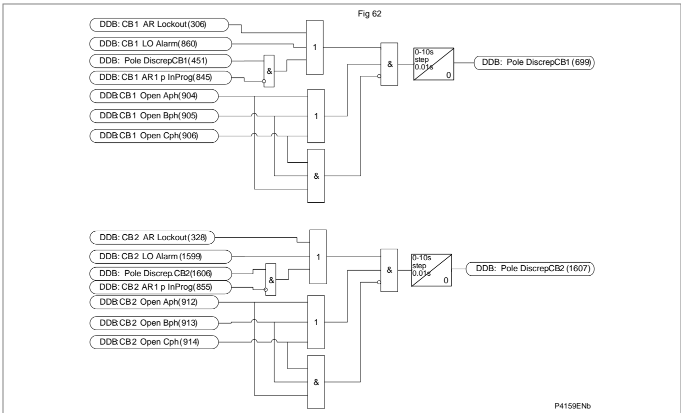
Figure AR-64 - Pole discrepancy (for P546 only)
