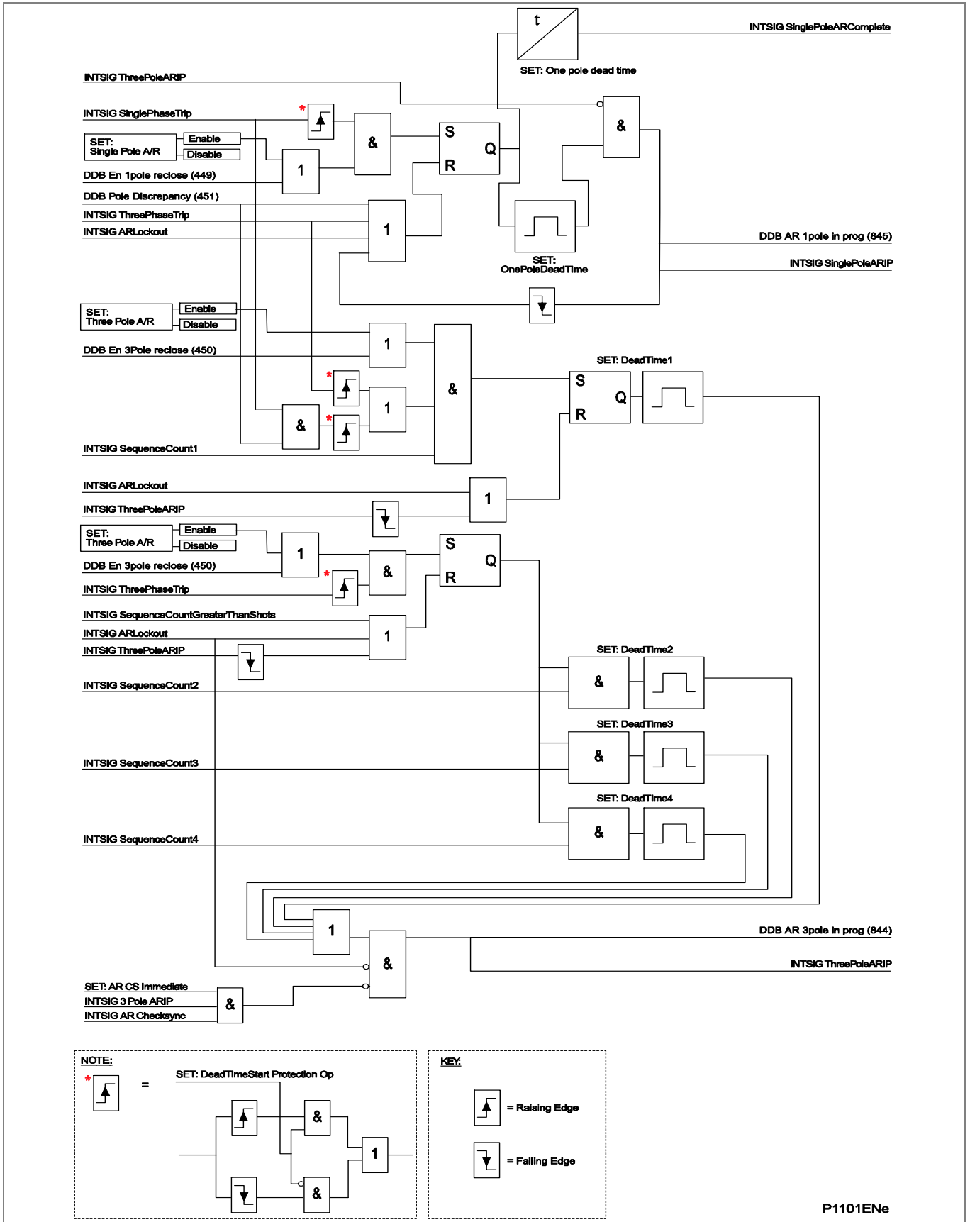
Figure 114 - Auto-reclose cycles (P543/P545)
