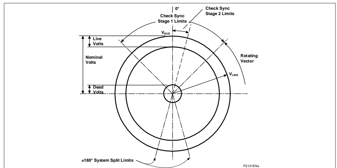
Figure 140 - Synchro check functionality (P544/P546)
