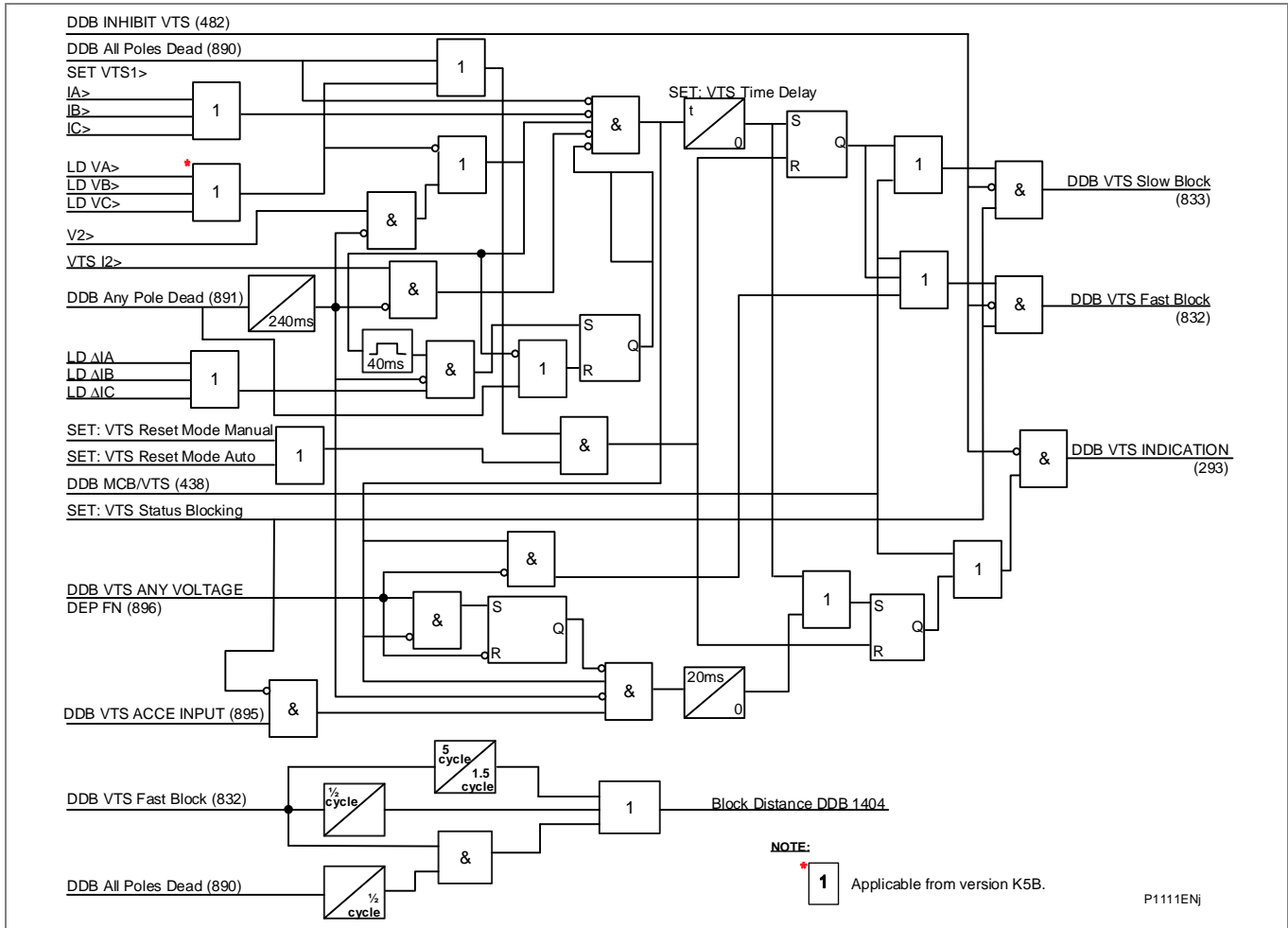
Figure 101 - VTS logic
