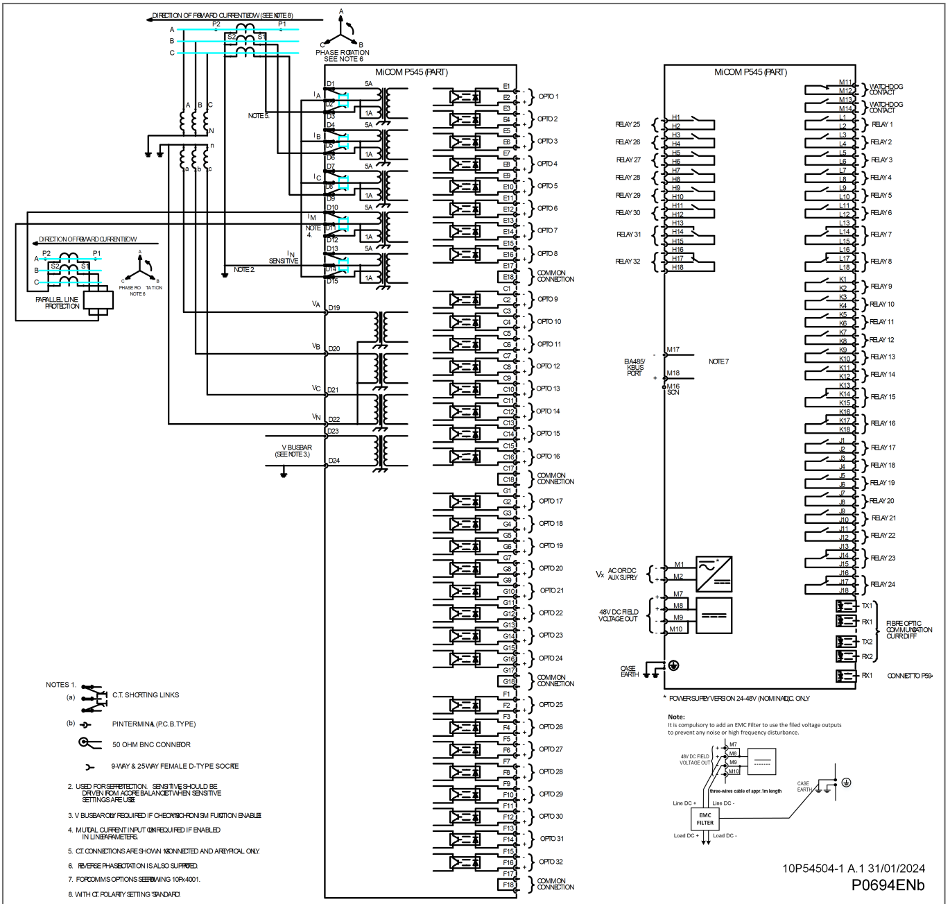
Figure 18 - P545 - 32 optos, 32 relays, Distance, 1 or 3 Pole Tripping, Auto-Reclose and Chk Sync Sheet 1
