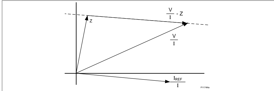
Figure 25 - Reactance line - top line of quadrilateral (Distance option only)
