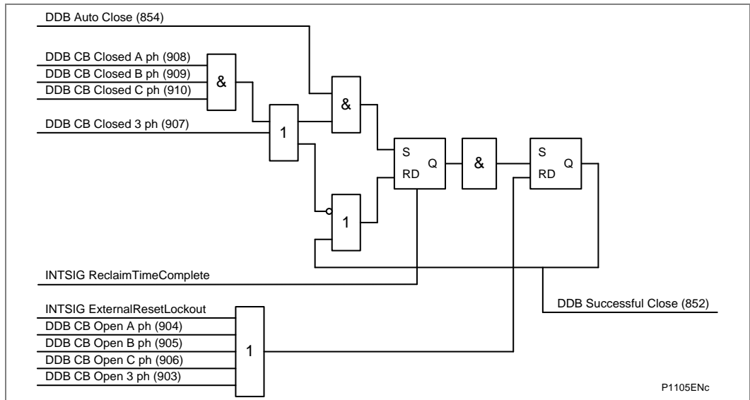
Figure 118 - Auto-reclose close notify (P543/P545)
