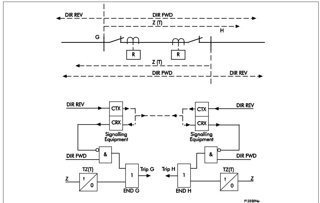
Figure 53 - Delta directional comparison BLOCKING scheme
