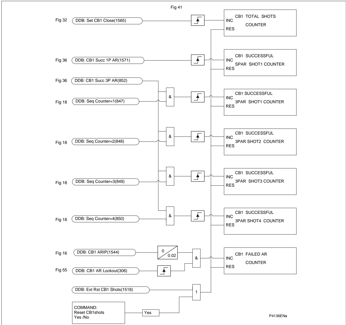
Figure AR-40 - AR shots counters
