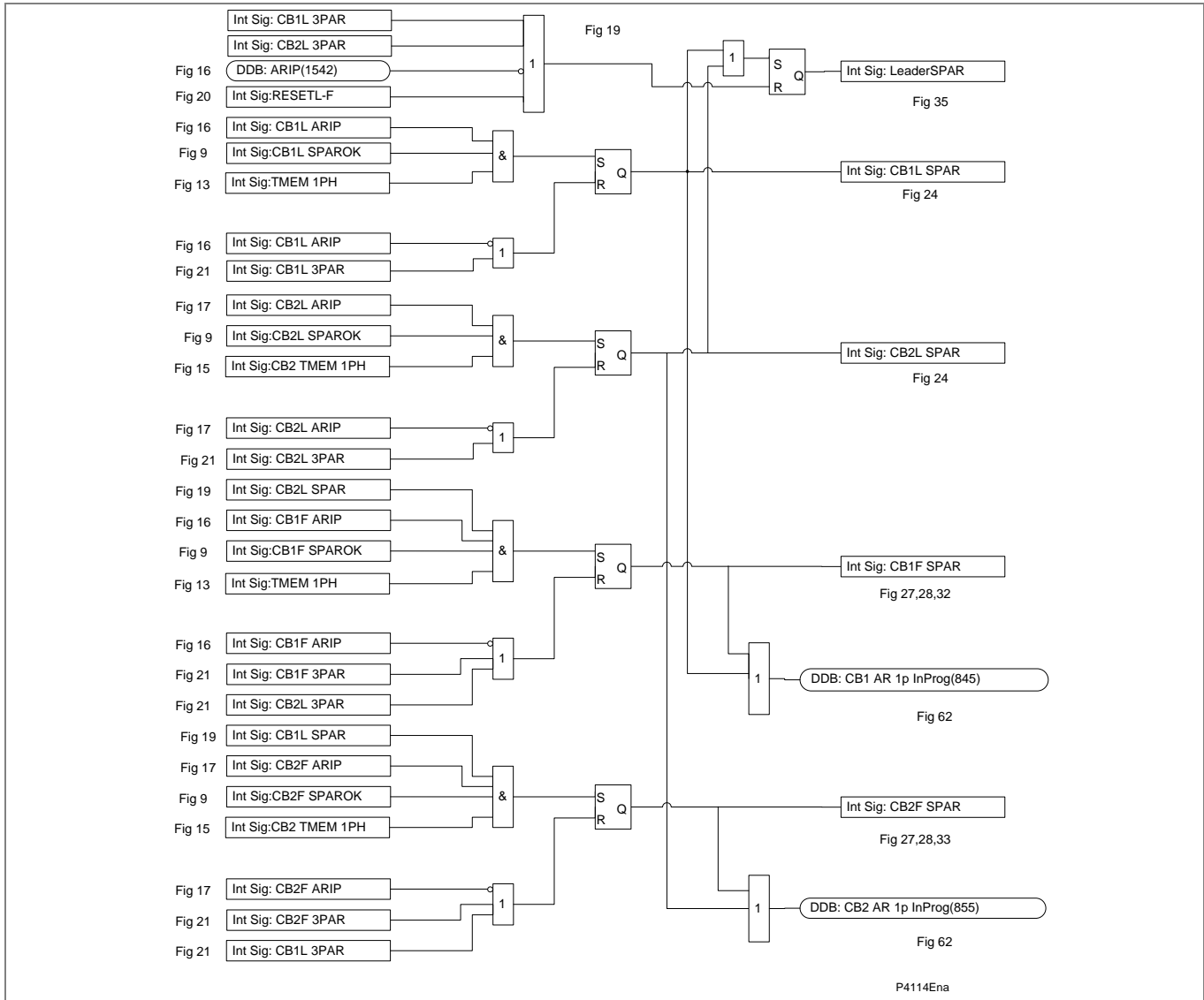
Figure AR-20 - Single phase AR cycle selection
