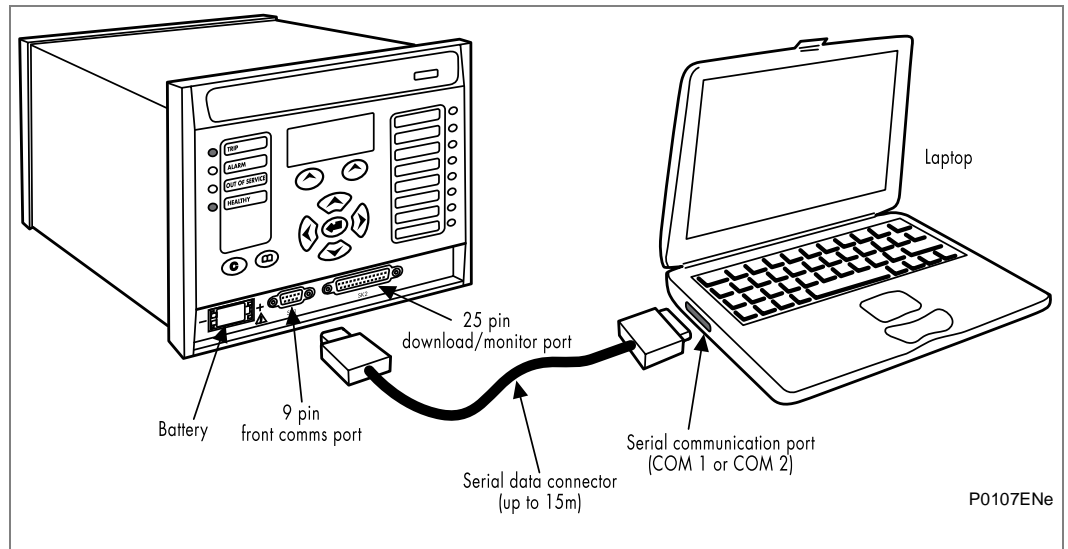
Figure 8 - Front port connection
