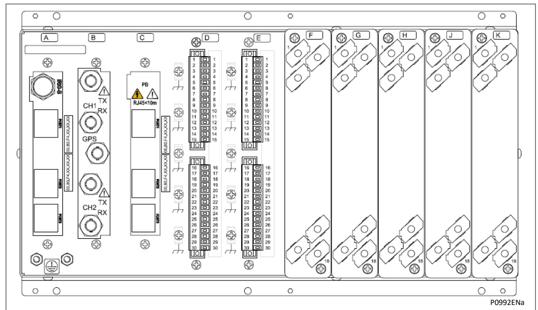
Figure 3 - Rear view of the process bus device
