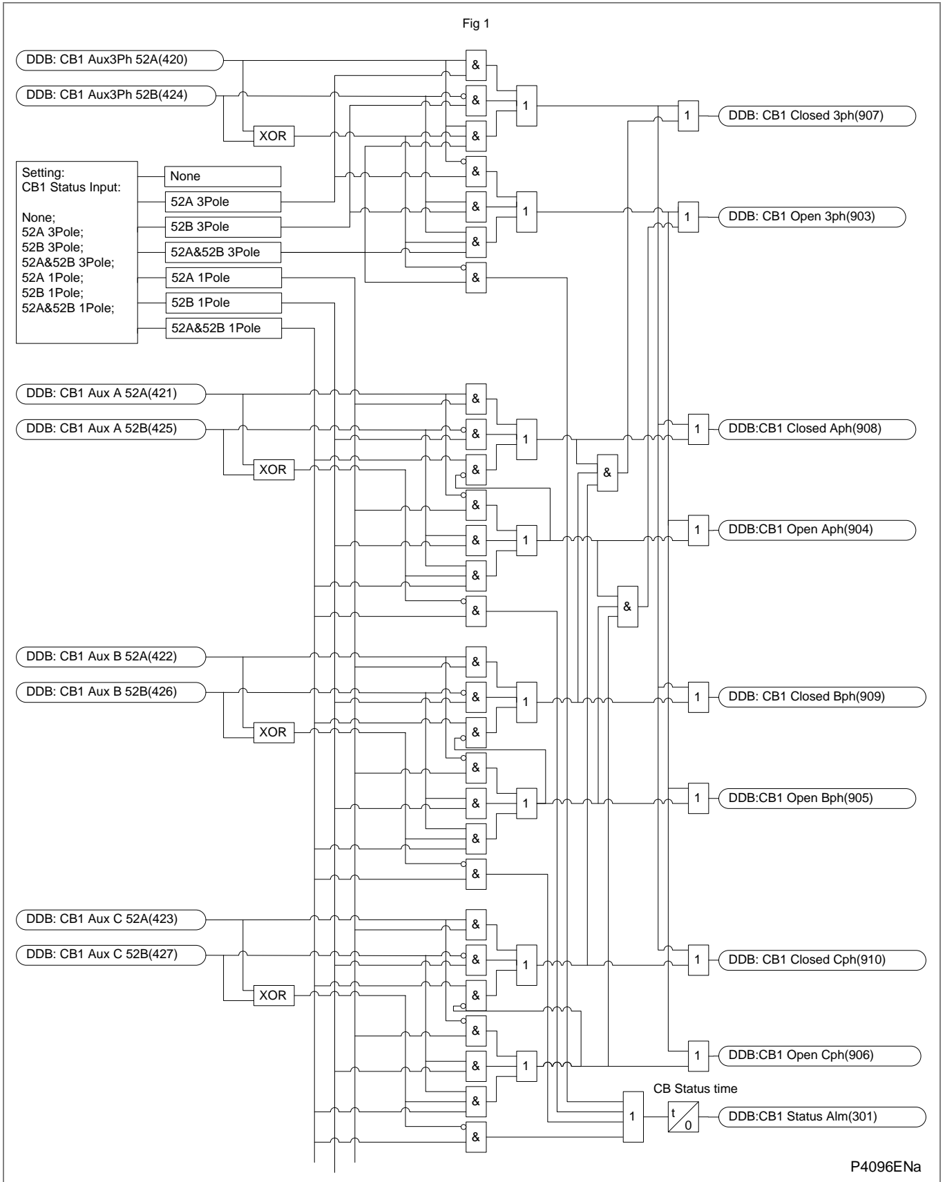
Figure AR-1 - Circuit breaker 1 - state monitor
