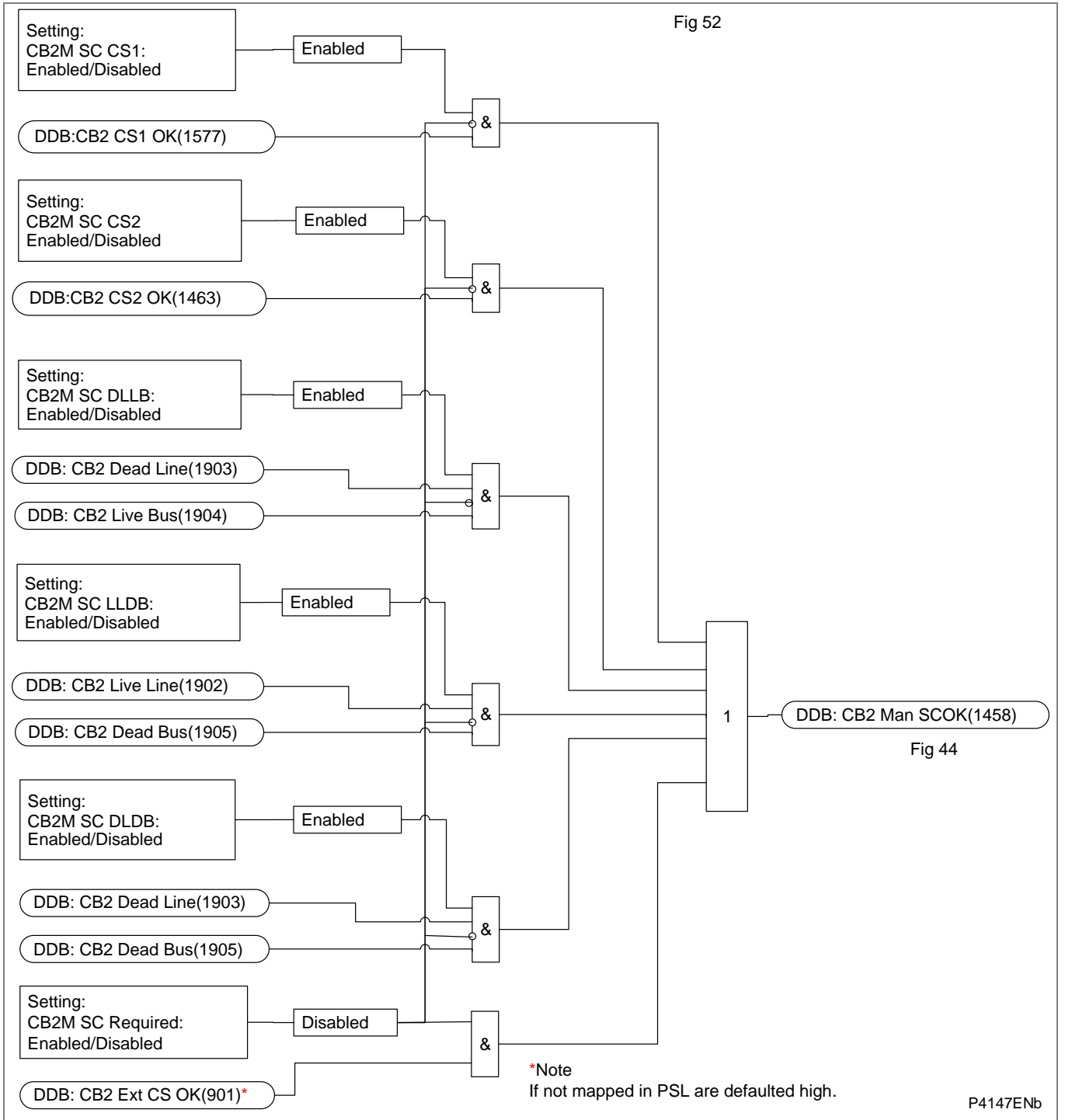
Figure AR-49 - CB2 man. close system check
