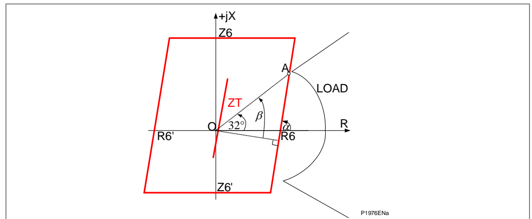
Figure 15 - R_{6\max} determination
