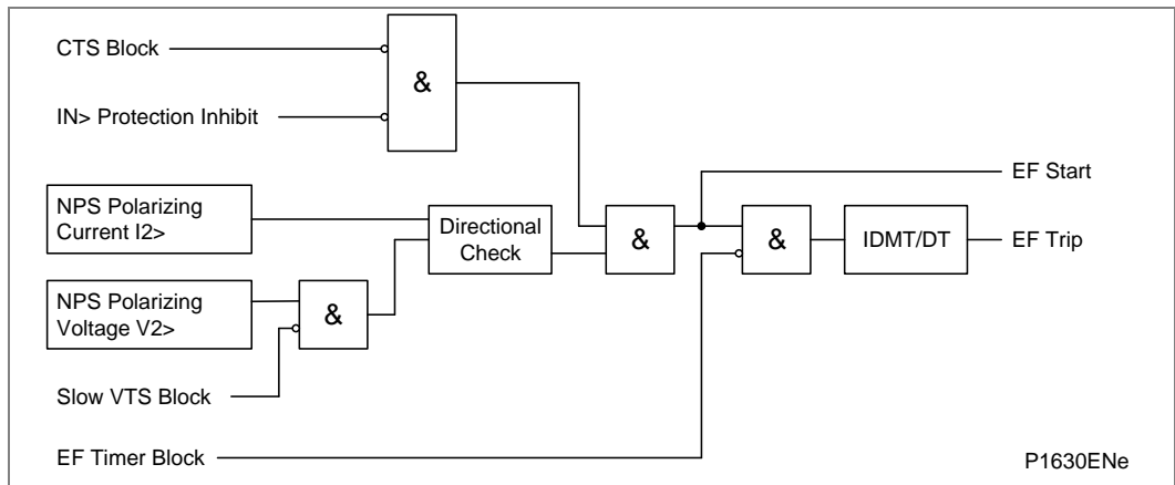
Figure 64 - Directional EF with negative sequence polarization (single stage)
