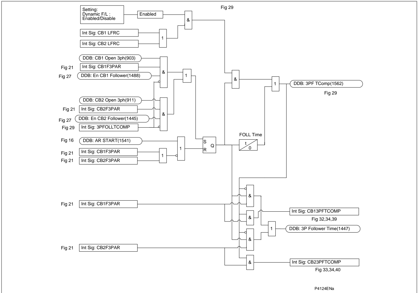
Figure AR-30 - Three phase follower time
