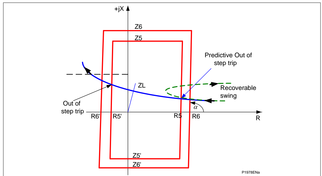
Figure 31 - Out-of-step detection characteristic (Distance option only)
