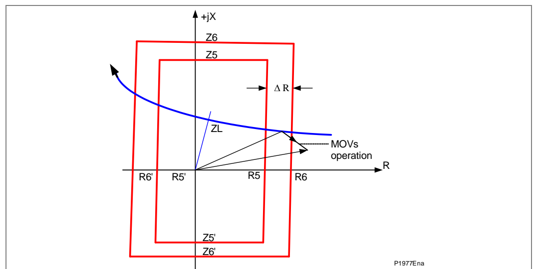
Figure 16 - Example of timer reset due to MOVs operation
