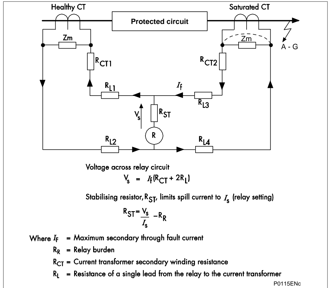
Figure 61 - High impedance principle
