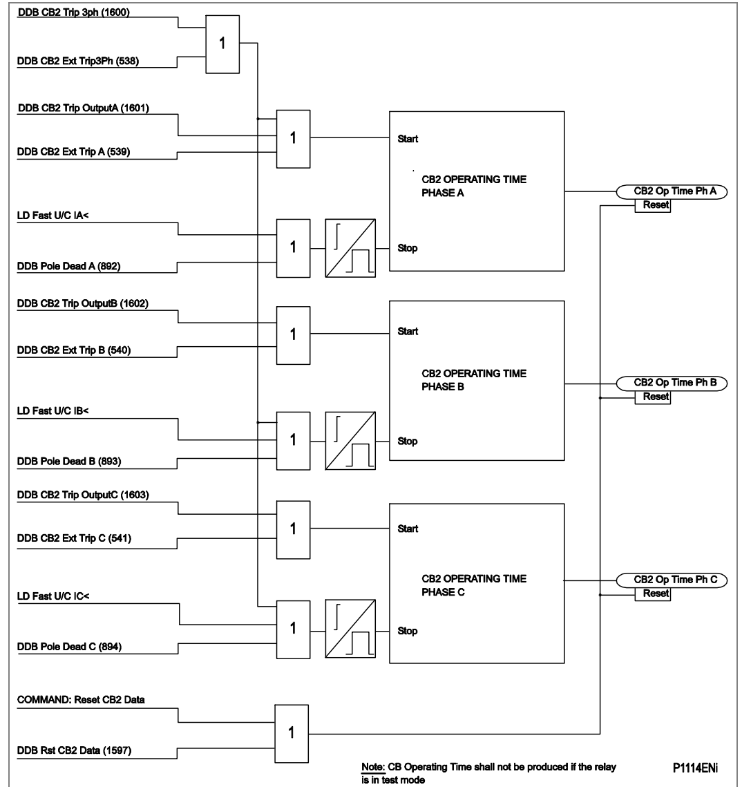
Figure 131 - CB2 condition monitoring – operation time
