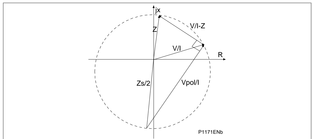
Figure 22 - Expansion of zone 1 for the default polarizing setting V pol =1 (Distance option only)
