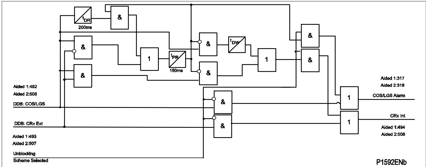
Figure 38 - Receive logic (Distance option only)
