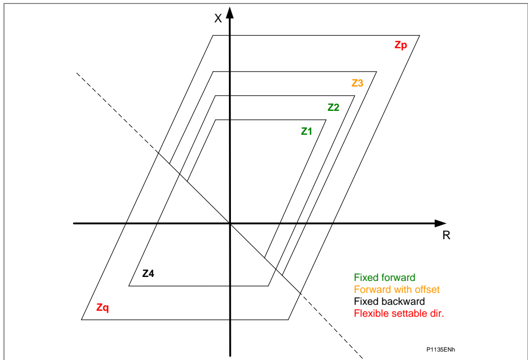
Figure 19 - Earth fault quadrilateral characteristics (Distance option only)
