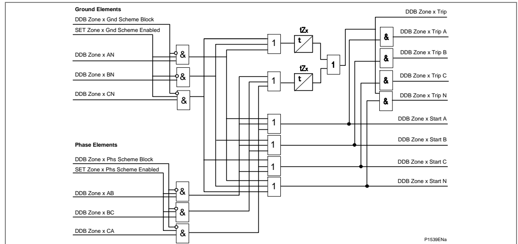
Figure 28 - Basic scheme delayed trip (Distance option only)
