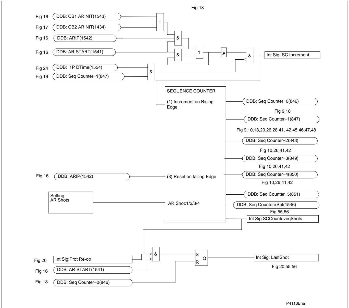
Figure AR-19 - Sequence counter
