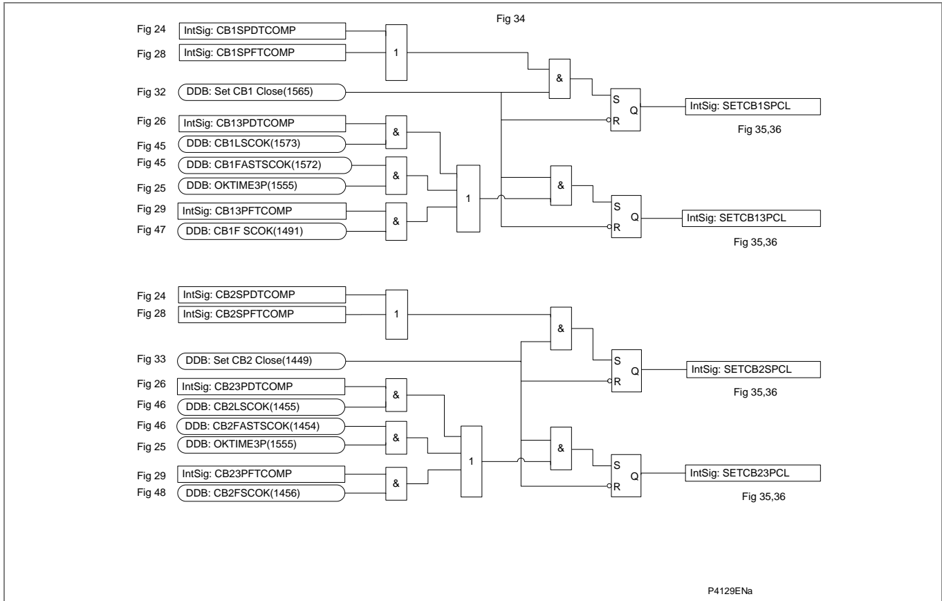
Figure AR-33 - Prepare reclaim initiation
