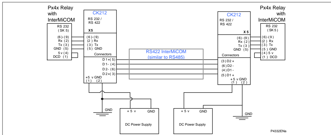
Figure 94 - MODEM InterMiCOM teleprotection via a RS422 protocol
