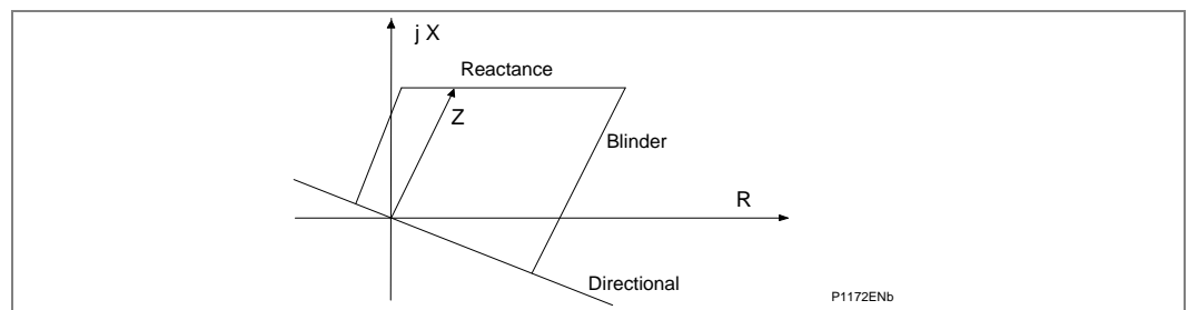
Figure 23 - Quadrilateral characteristics (directional line shown simplified) (Distance option only)
