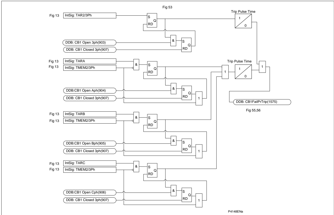
Figure AR-50 - CB1 trip time monitor
