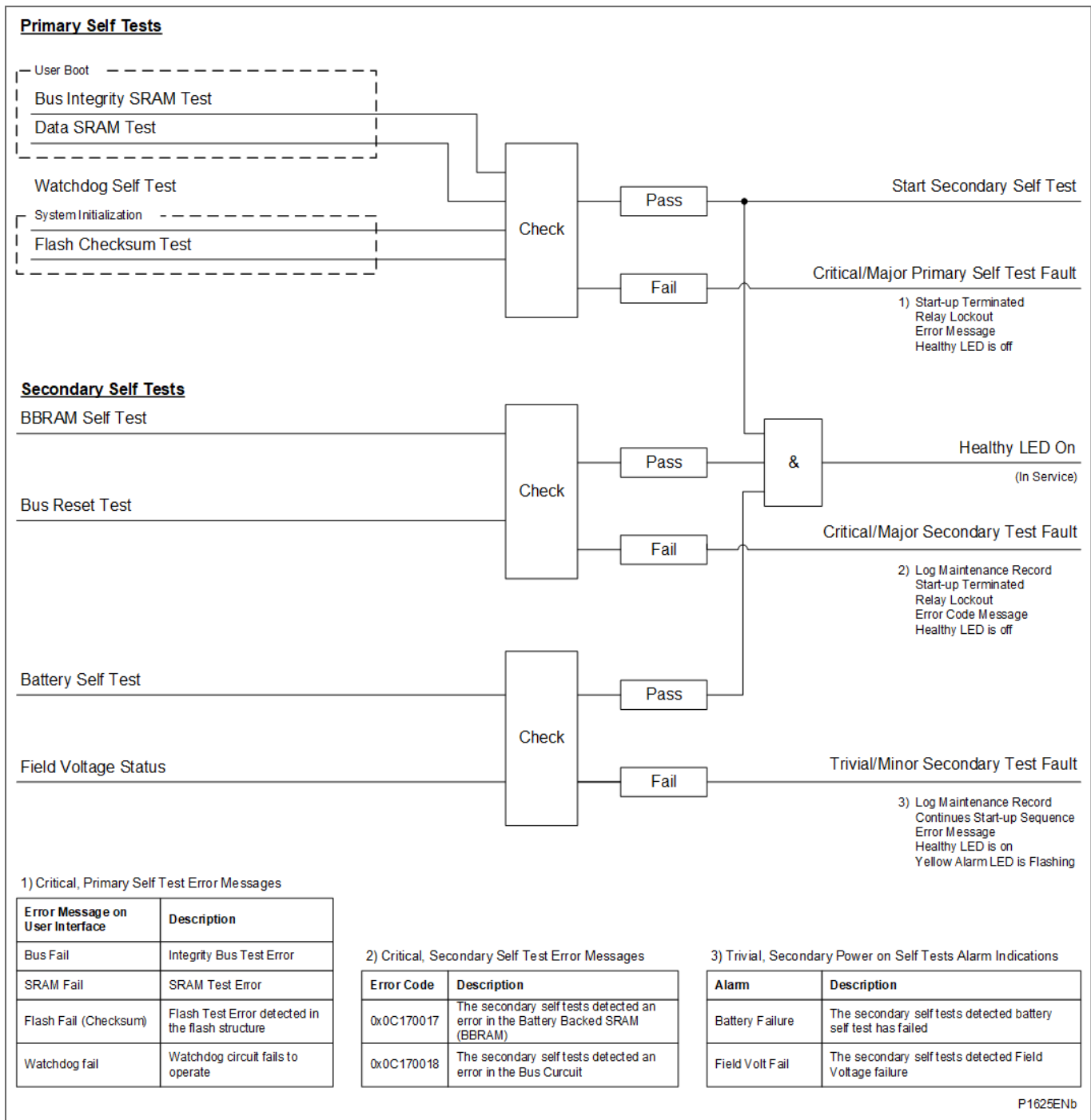
Figure 15 - Start-up self-testing logic diagram
