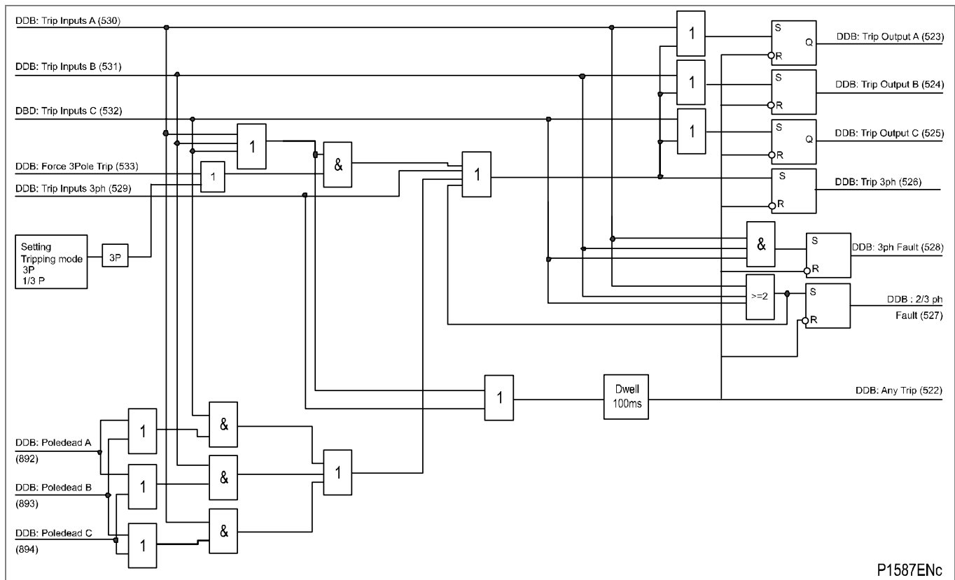
Figure 15 - Trip conversion scheme logic
