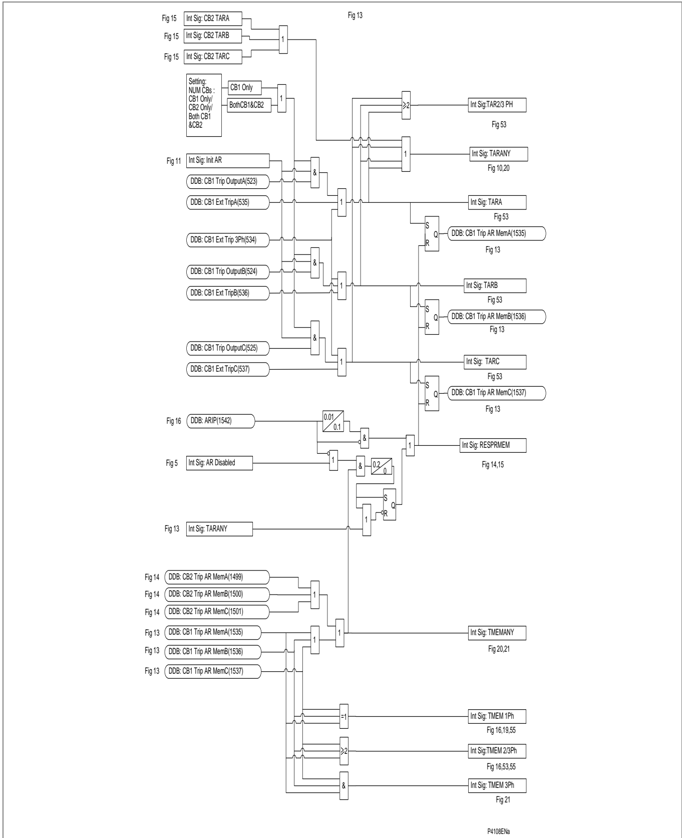
Figure AR-14 - CB1 1pole / 3-pole trip + AR initiation
