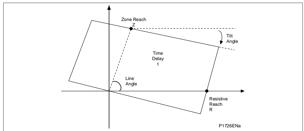
Figure 10 - Settings required to apply a quadrilateral zone (Distance option only)
