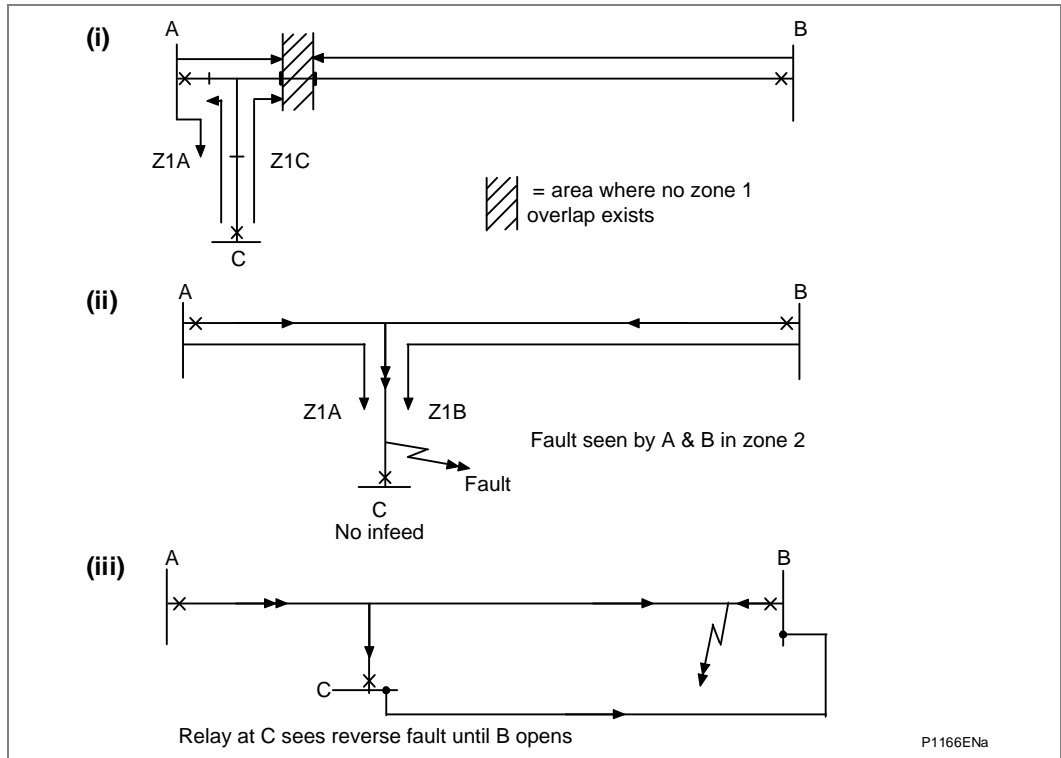
Figure 30 - Teed feeder applications
