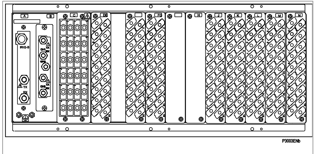
Figure 3 - Rear terminal blocks on size 80TE case
