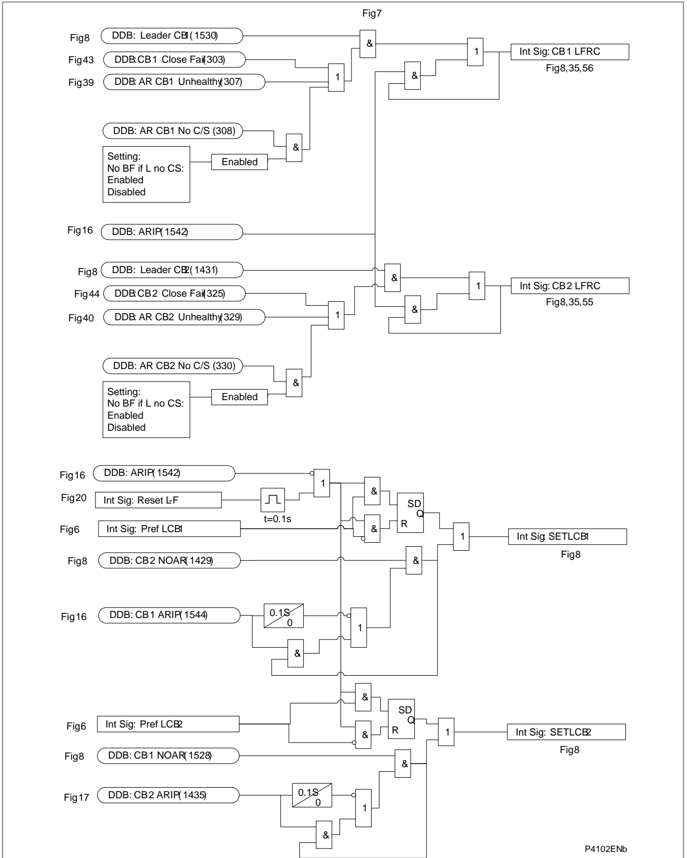
Figure AR-8 - Leader/follower logic – 1 (for Software Versions H1 and later)
