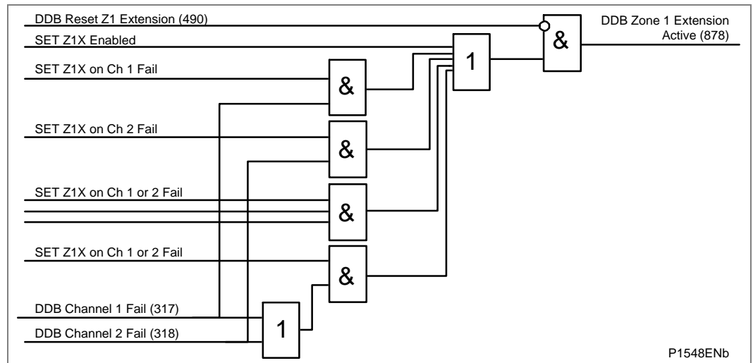
Figure 55 - Zone 1 extension
