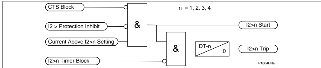
Figure 65 - Negative sequence overcurrent non-directional operation
