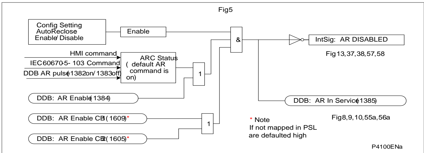
Figure AR-5 - Auto-reclose enable
