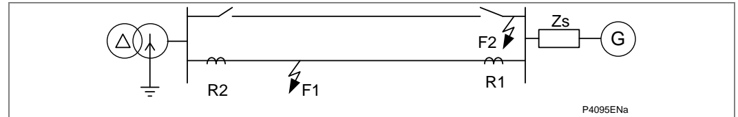
Figure 78 - Weak infeed configuration on stub-fed radial circuit (parallel line is out of service)
