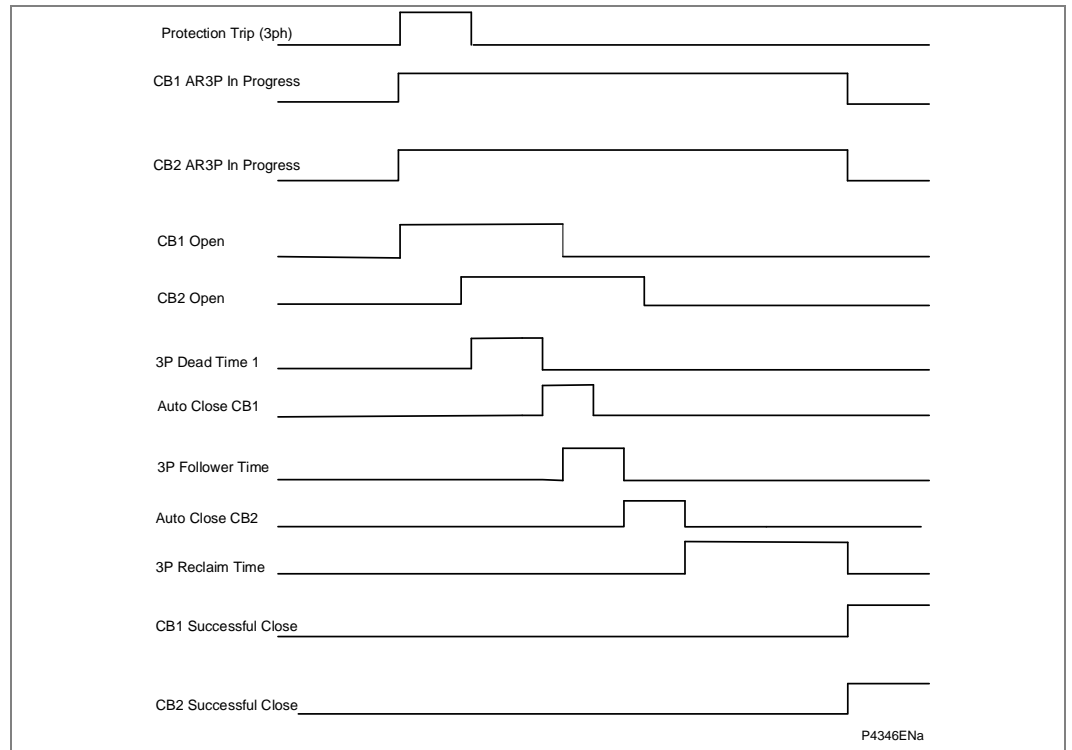
Figure 139 - Auto-reclose timing diagram leader/follower (3ph)
