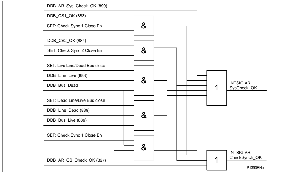
Figure 120 - Auto-reclose/check sync interface (P543/P545)
