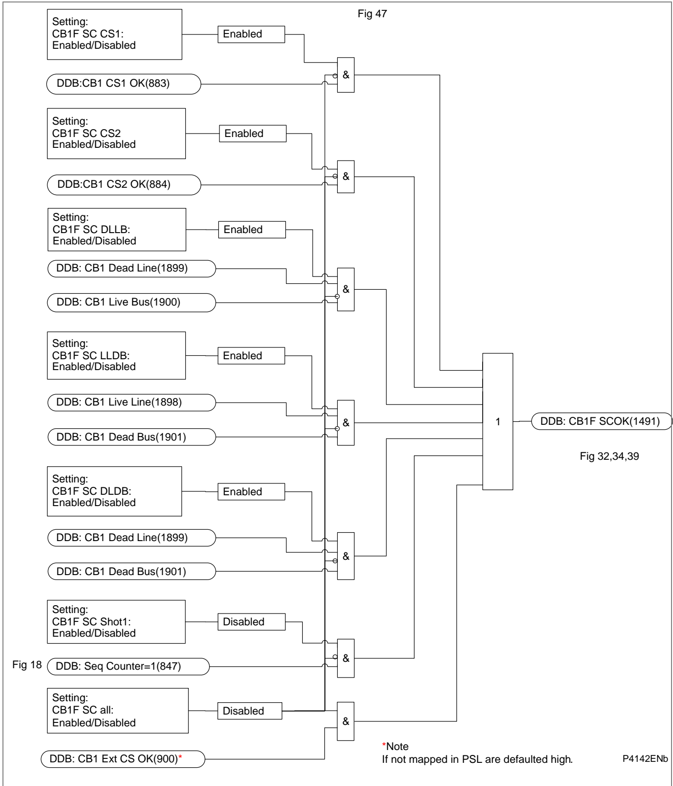
Figure AR-46 - CB1 follow 3PAR system check
