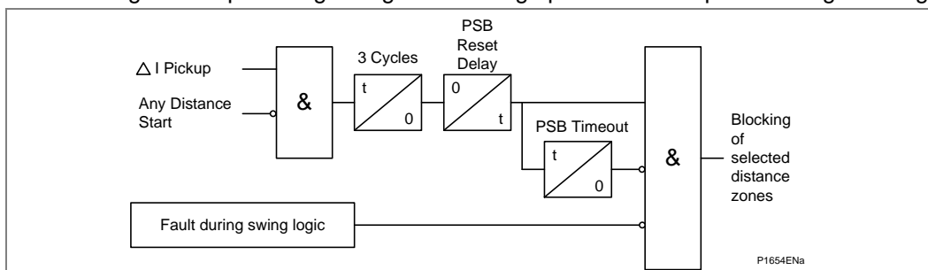
Figure 30 - Power swing blocking (Distance option only)
