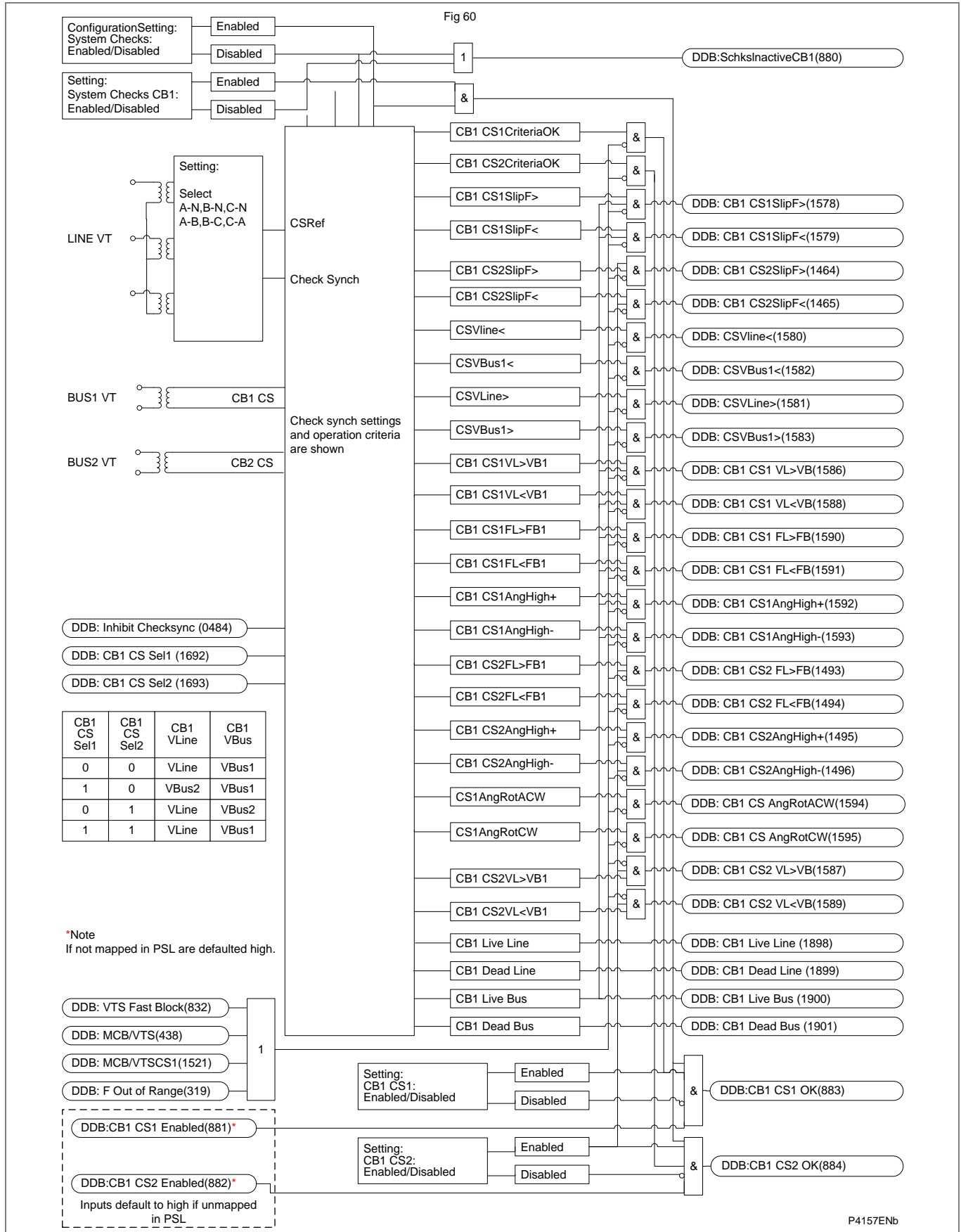
Figure AR-61 - CB1 synch check signals
