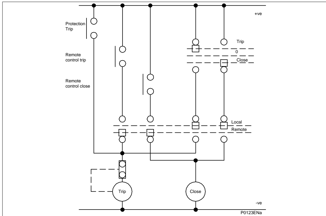
Figure 124 - Remote control of circuit breaker (P543/P545)
