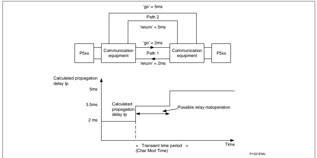
Figure 86 - Switched communication network
