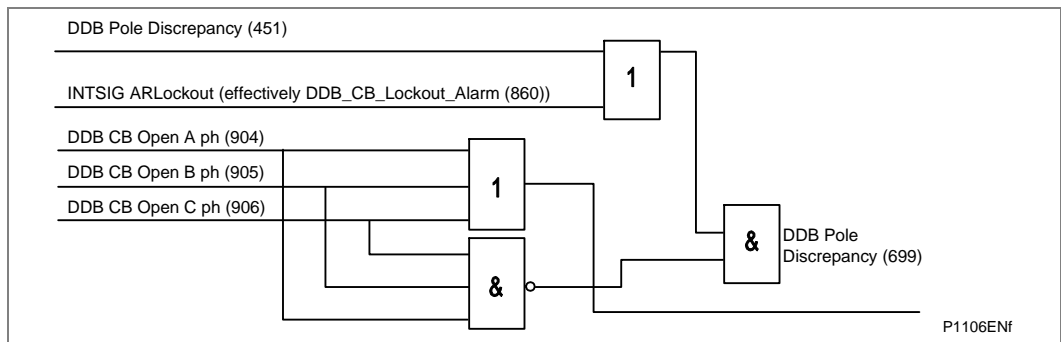
Figure 119 - Ddb pole discrepancy trip (P543/P545)
