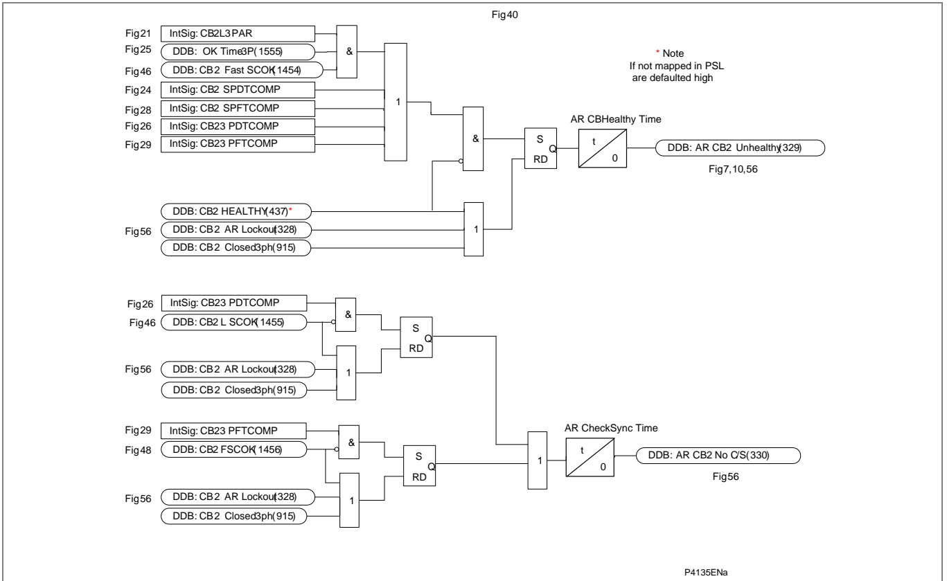
Figure AR-39 - CB2 healthy & system check timers
