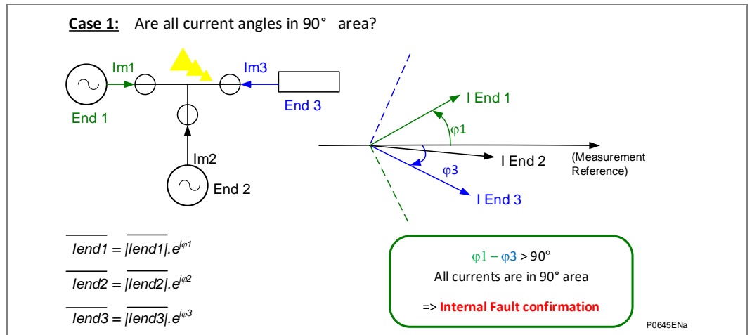
Figure 1 - Differential 3-terminal scheme - internal fault
