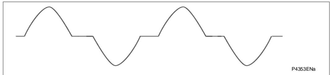
Figure 6 - Typical overflux current waveform
