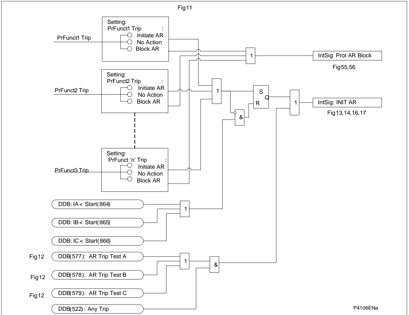
Figure AR-12 - Auto-reclose initiation
