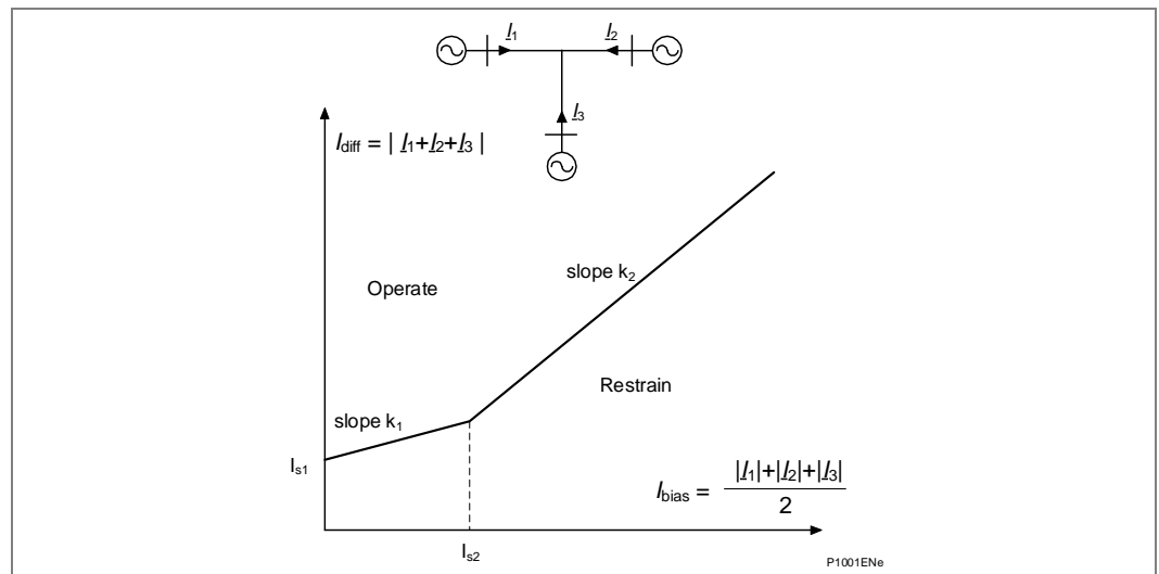
Figure 1 - Relay bias characteristic
