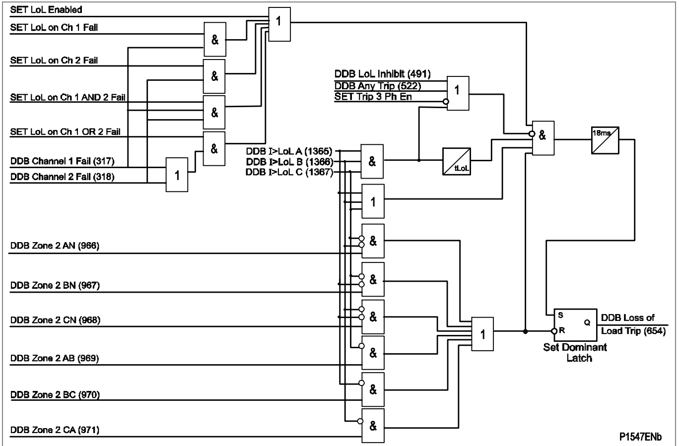
Figure 57 - Loss of load (Distance option only)
