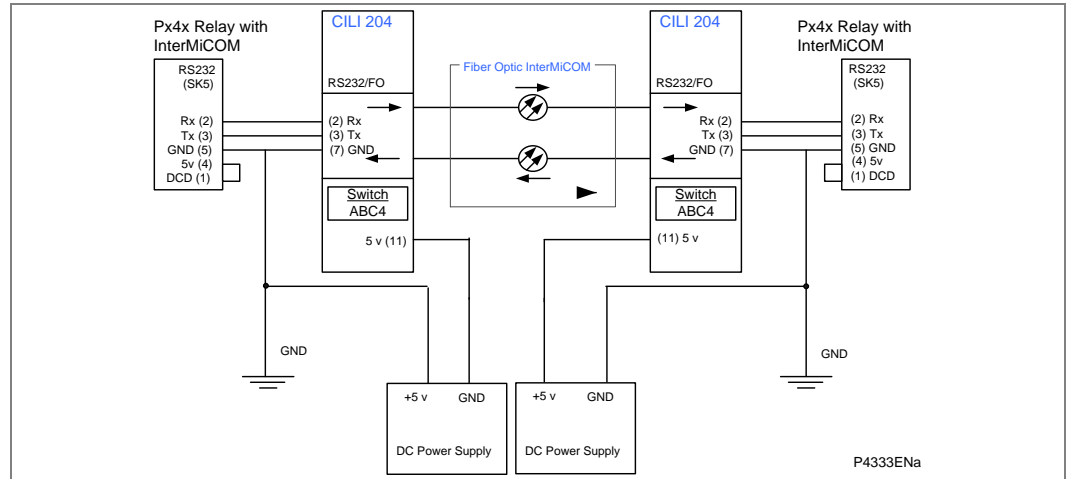
Figure 95 - MODEM InterMiCOM teleprotection via fiber optic
