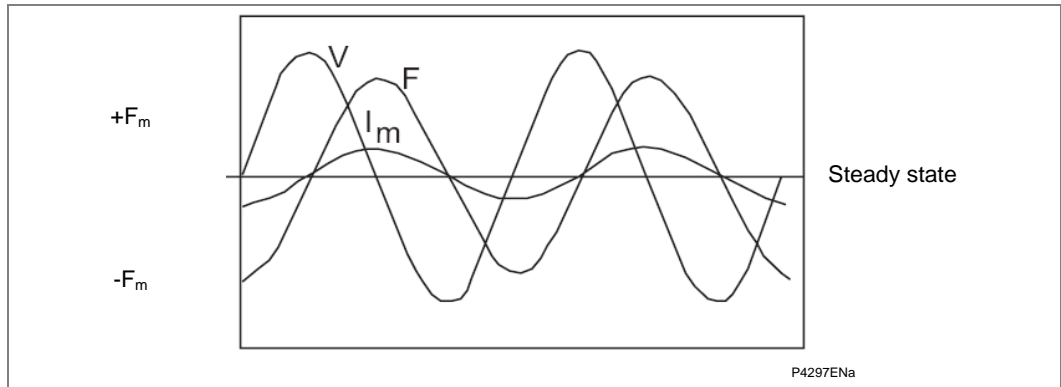
Figure 3 - Steady state magnetizing inrush current
