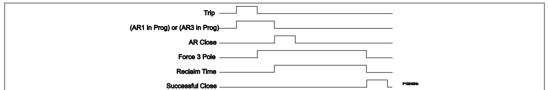
Figure 107 - Auto-reclose timing diagram - single fault
