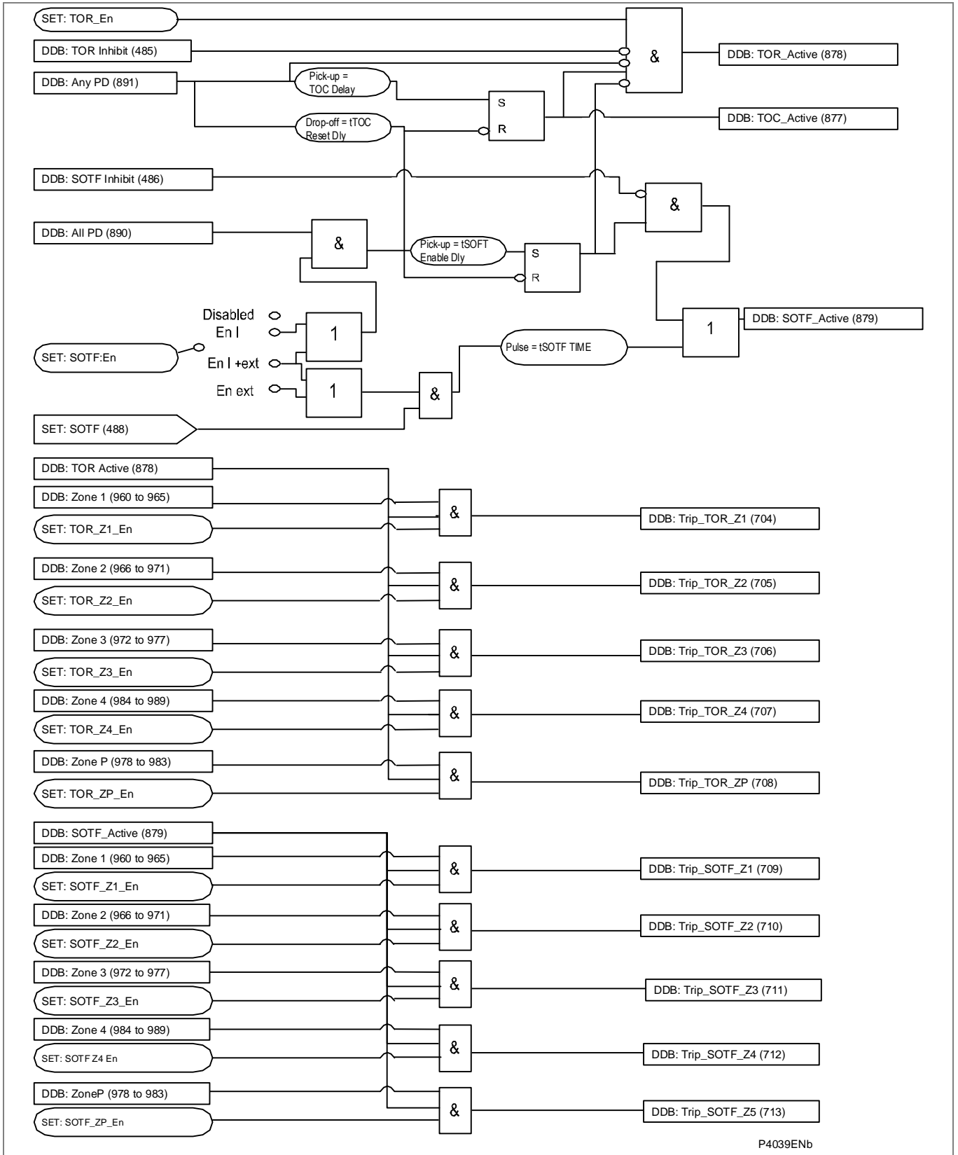
Figure 33 - Trip on close (Distance option only)
