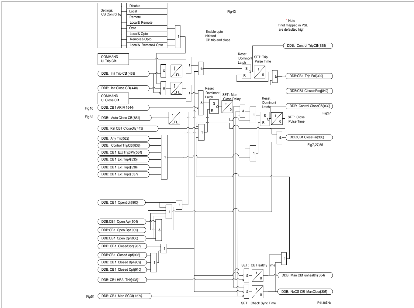
Figure AR-42 - CB1 circuit breaker control
