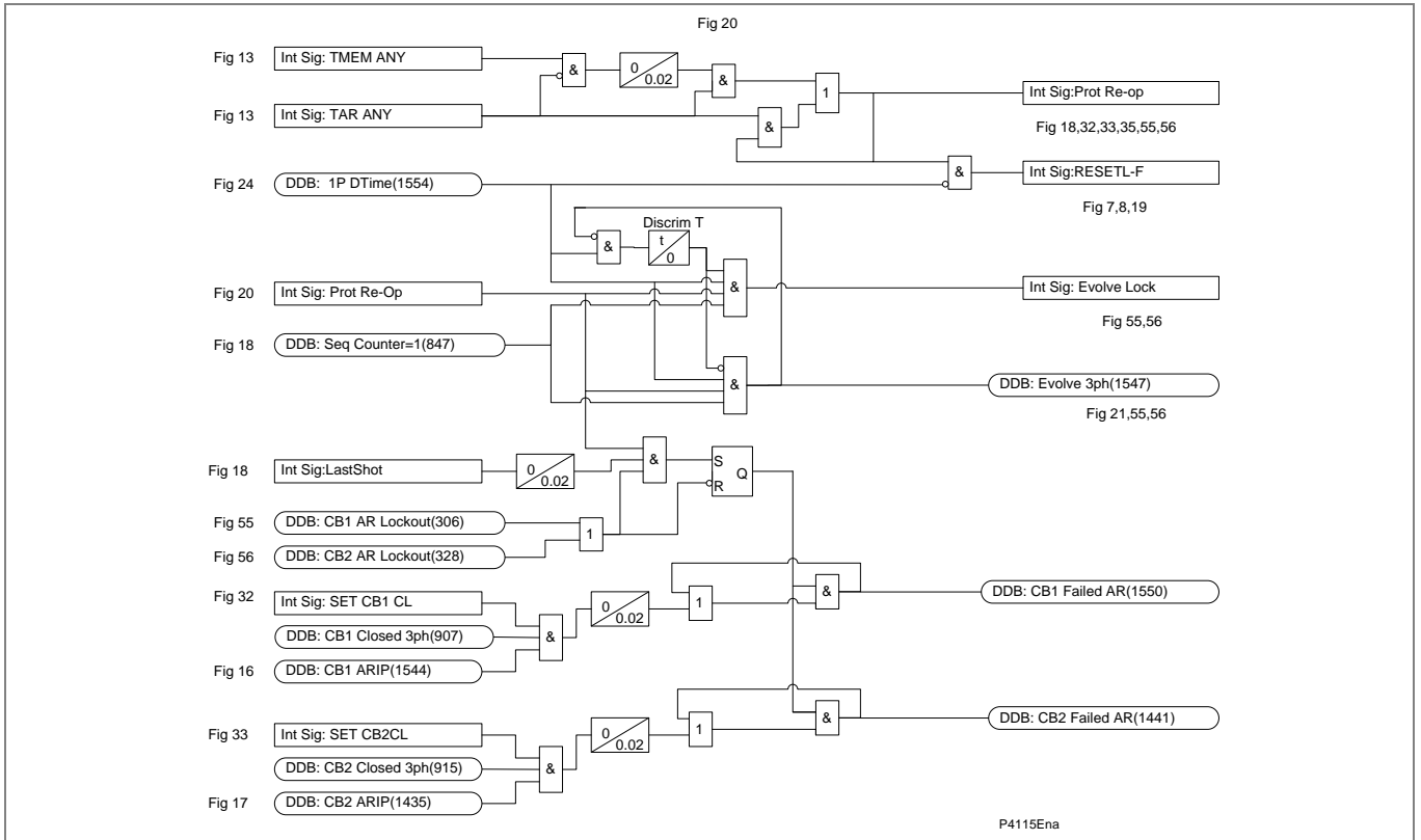
Figure AR-21 - Protection re-operation + evolving fault + persistent fault
