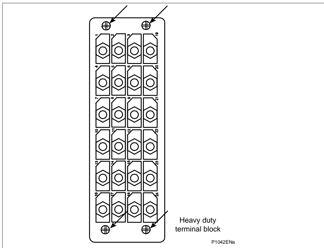
Figure 4 - Location of securing screws for heavy duty terminal blocks
