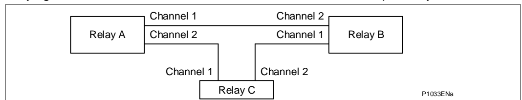
Figure 89 - 3-terminal system connection
