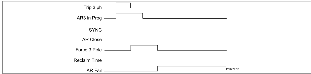
Figure 110 - Auto-reclose timing diagram - lockout for no checksynch
