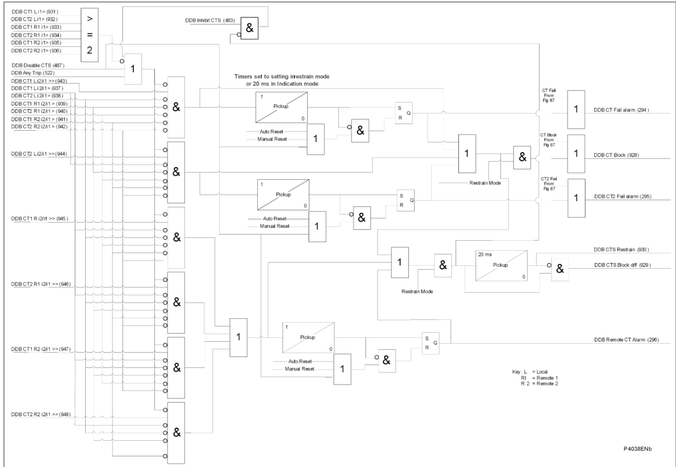
Figure 102 - Differential CTS
