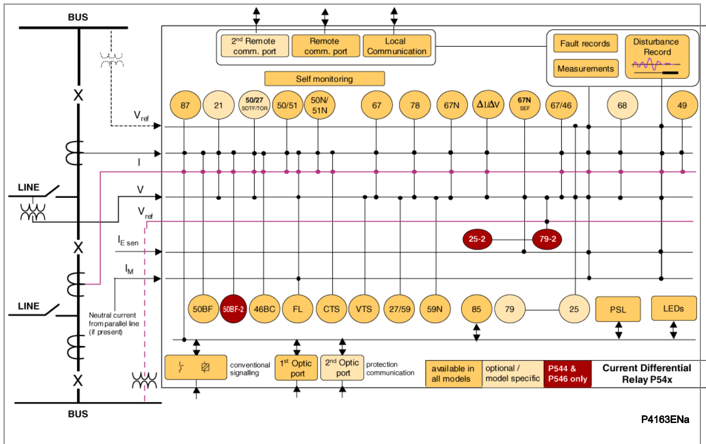
Figure 2 - Functional diagram
