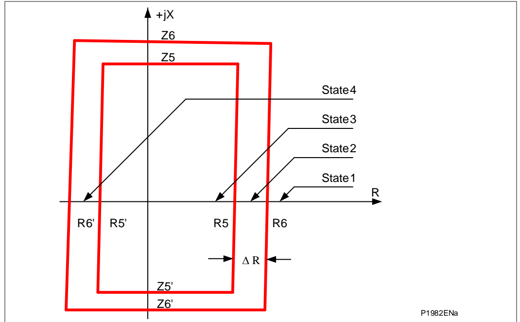
Figure 6 - Four state impedances
