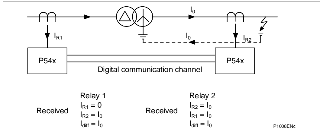
Figure 12 - Need for zero-sequence current filtering
