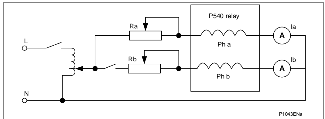
Figure 5 - Connection for bias characteristic testing
