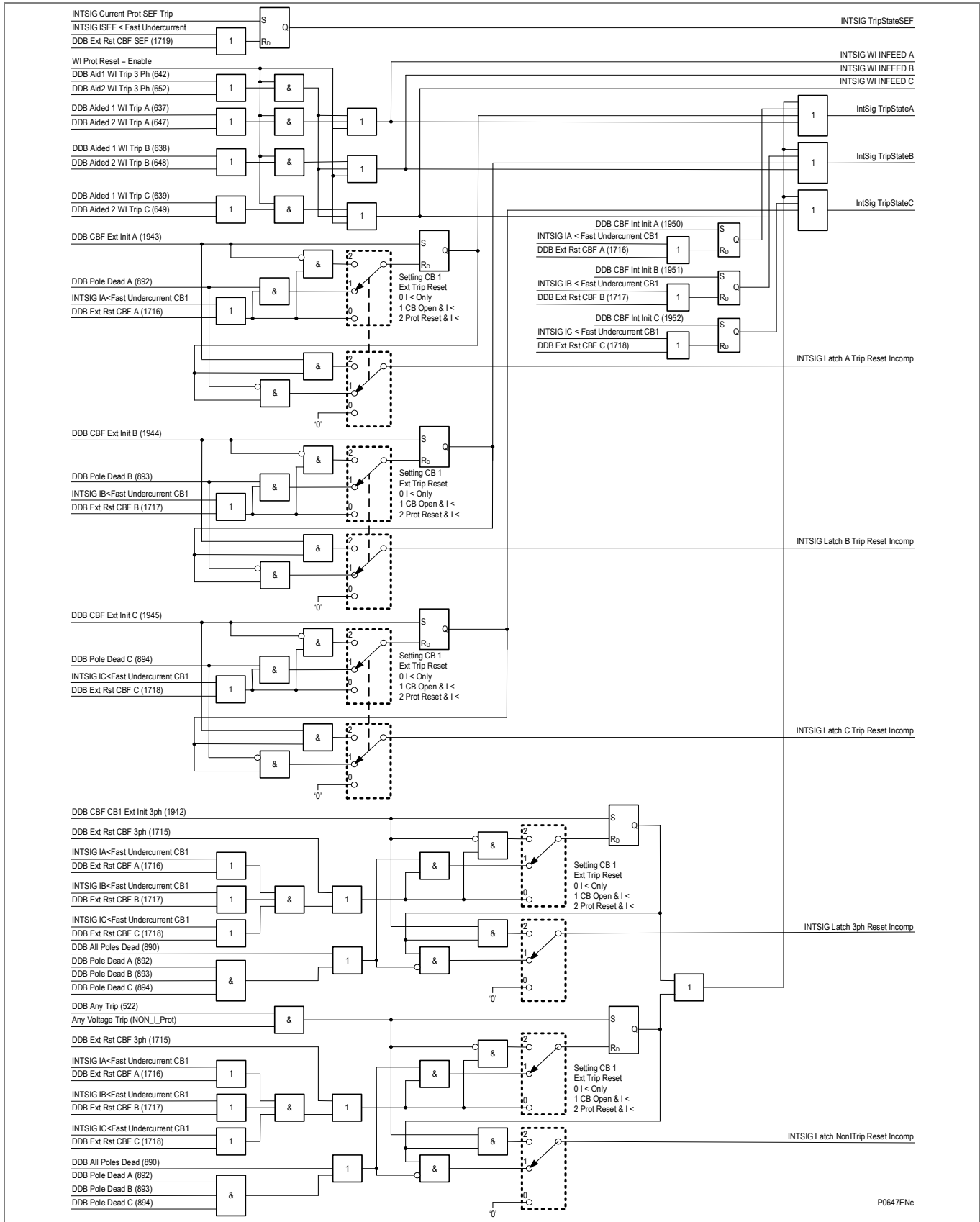
Figure 72 - CB Failure CB1 logic part 1
