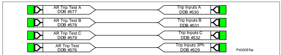
Figure 1 - Auto-reclose default PSL - P543 & P545 SW ver 44 and 54
