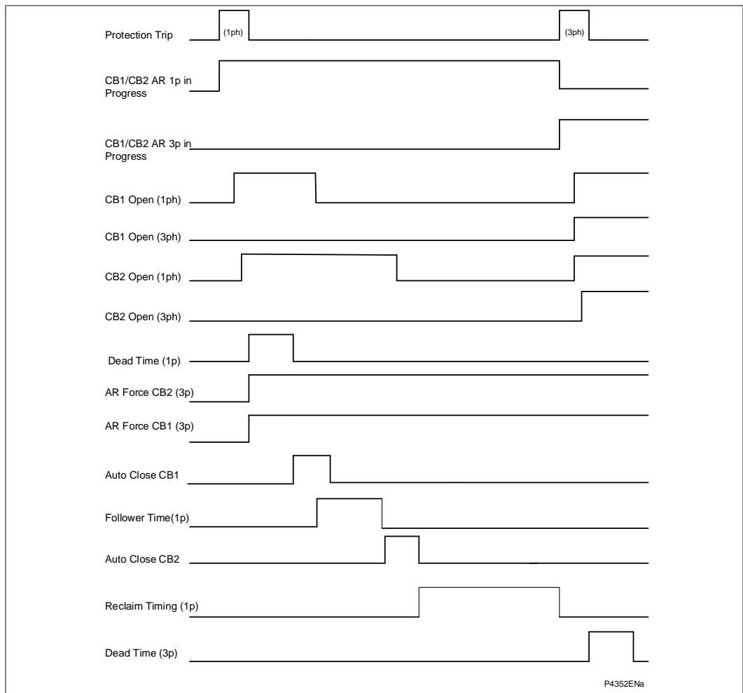
Figure 137 - Auto-reclose timing diagram – repeated fault inception
