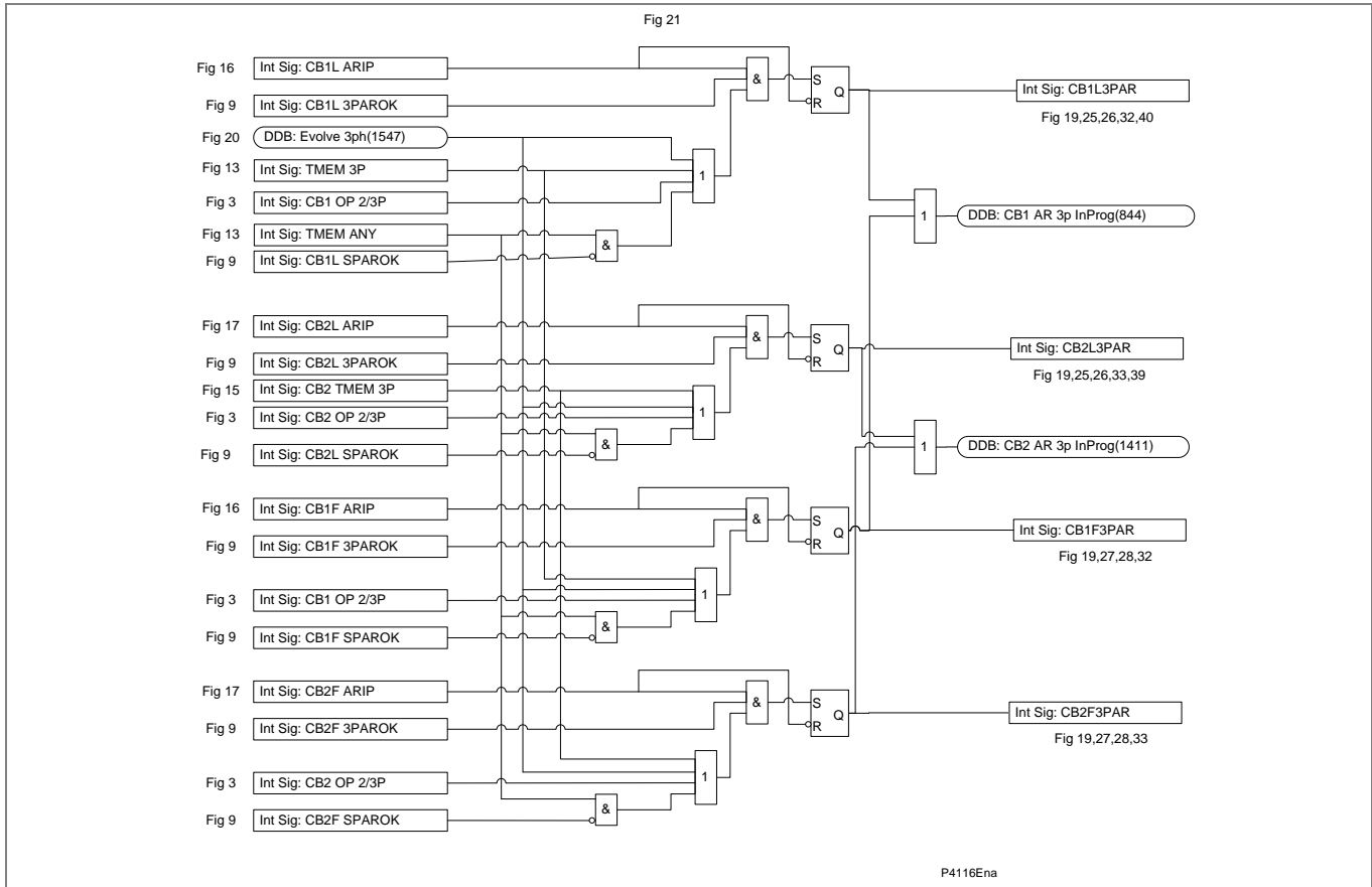
Figure AR-22 - Three phase AR cycle selection
