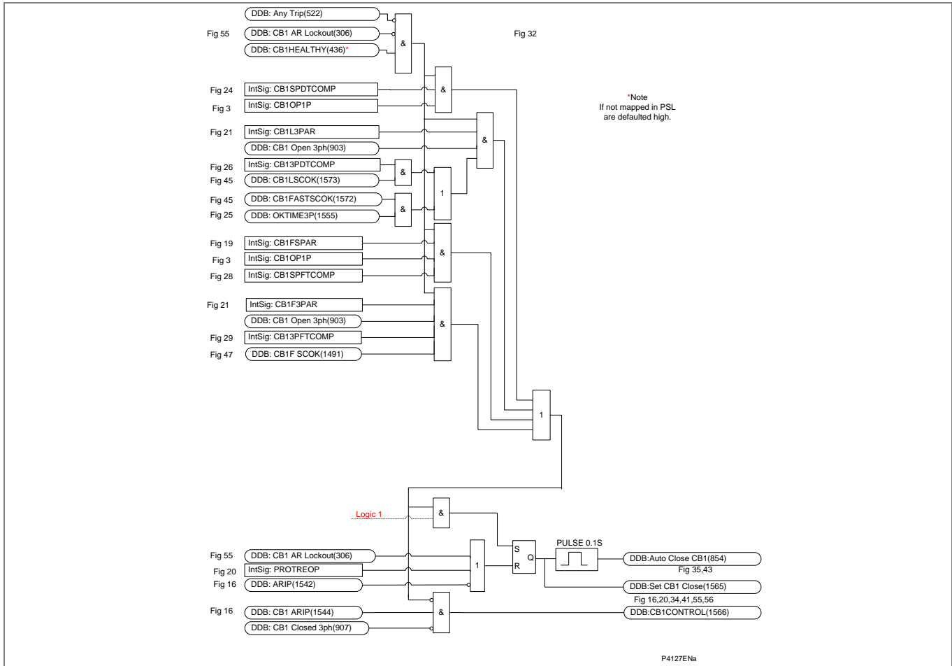
Figure AR-31 - CB Auto close
