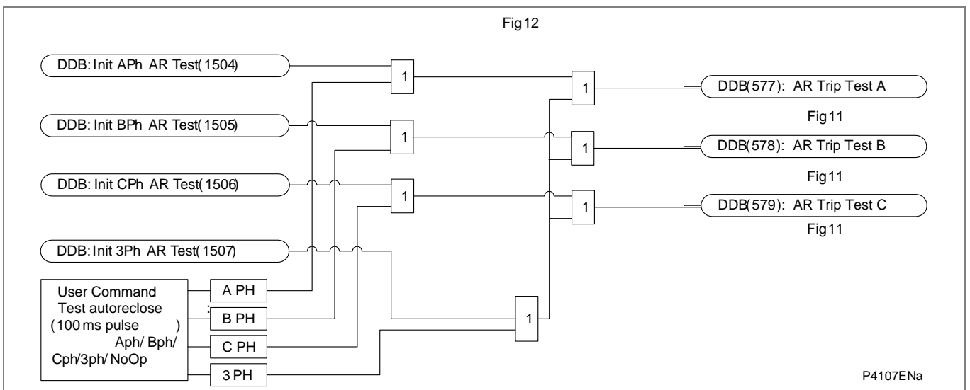
Figure AR-13 - Test trip & AR initiation
