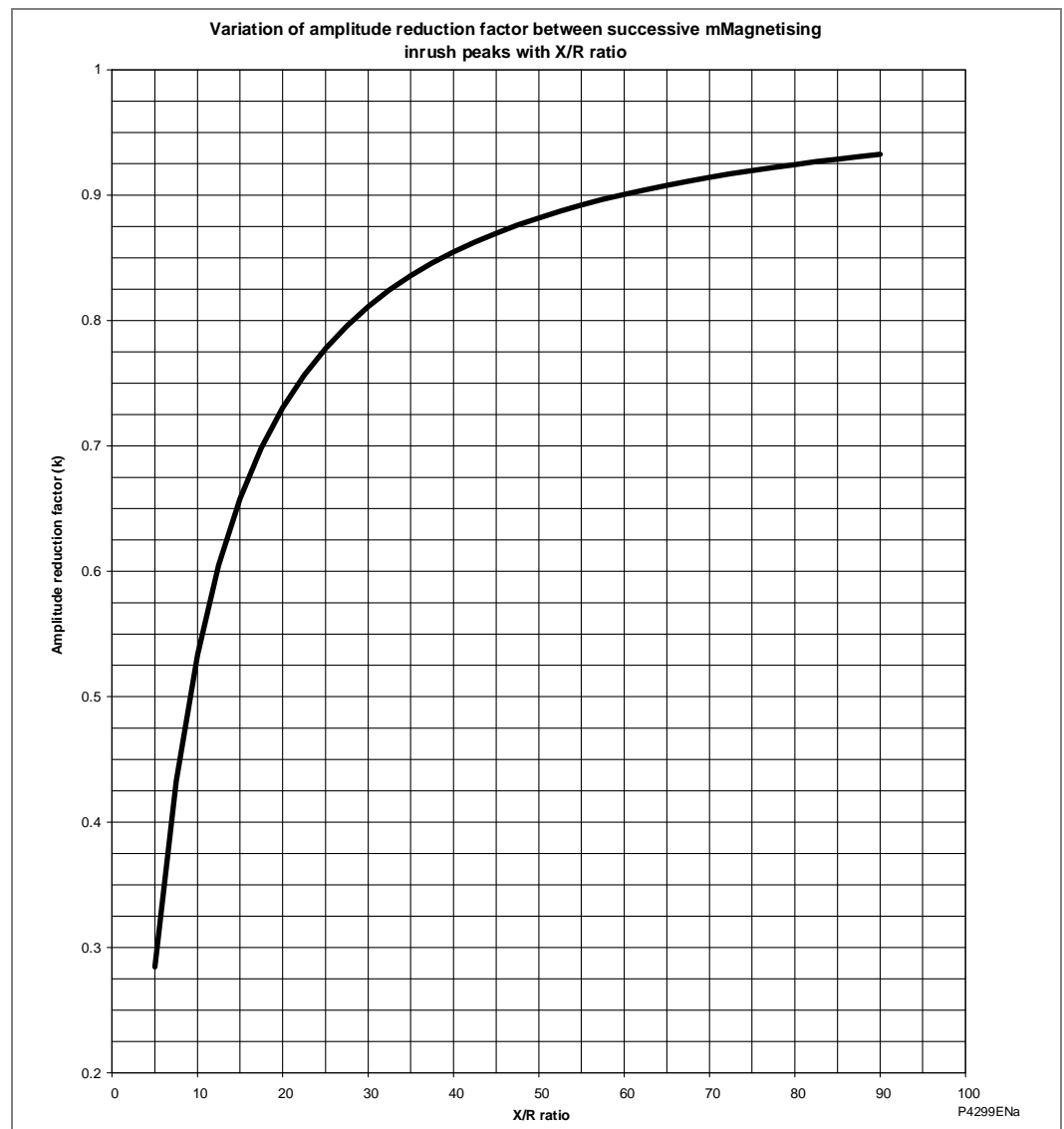
Figure 5 - Variation of amplitude reduction factor
