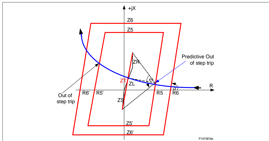
Figure 14 - Setting determination for the positive sequence resistive component R5
