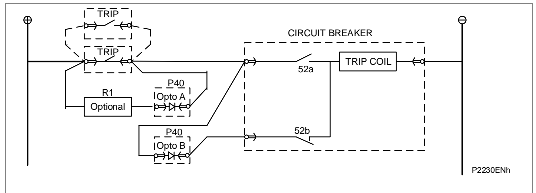
Figure 35 - TCS scheme 2b
