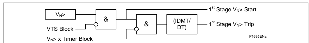
Figure 69 - Residual overvoltage logic (single stage)
