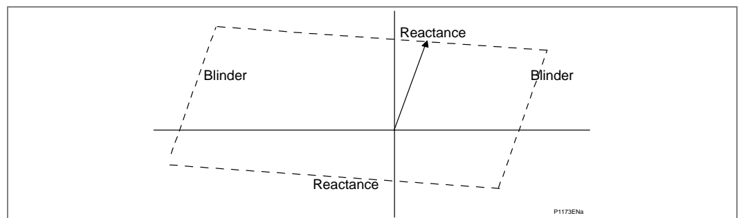
Figure 24 - Offset quadrilateral for zone 3 (Distance option only)
