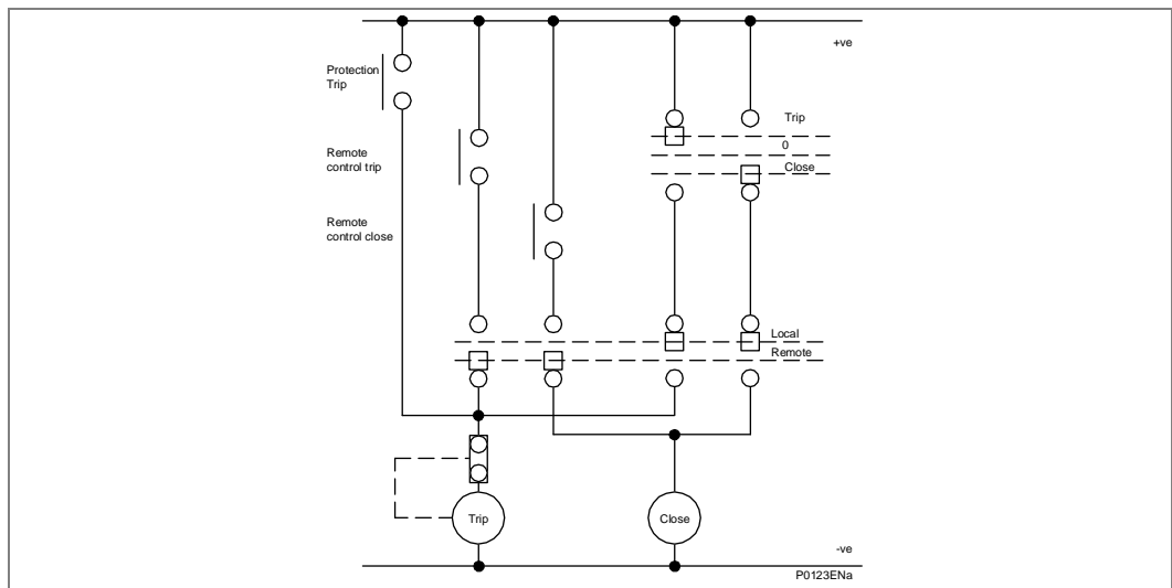
Figure 134 - Remote control of circuit breaker
