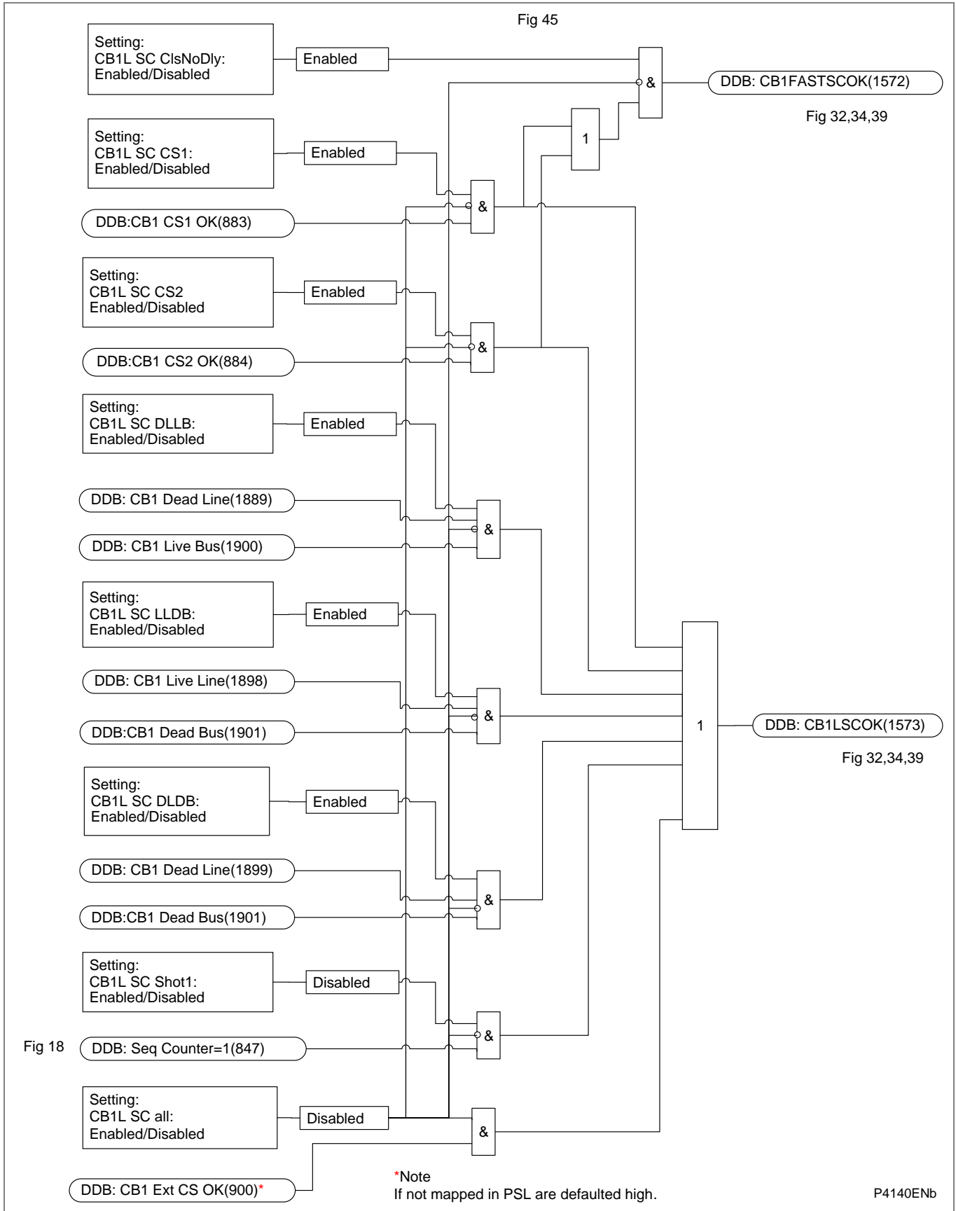
Figure AR-44 - CB1 lead 3PAR system check
