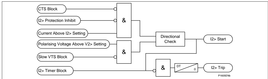
Figure 66 - Directionalizing the negative phase sequence overcurrent element
