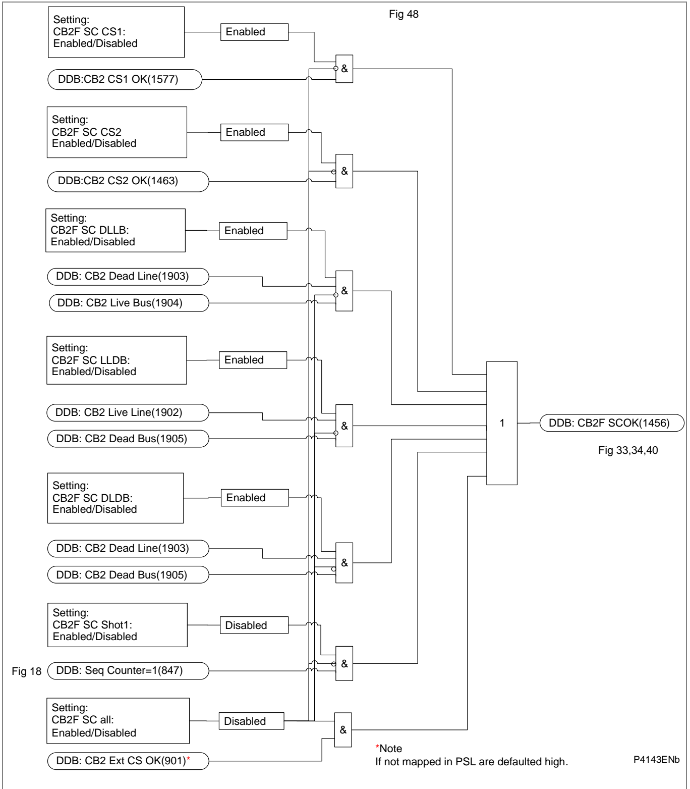
Figure AR-47 - CB2 follow 3PAR system check
