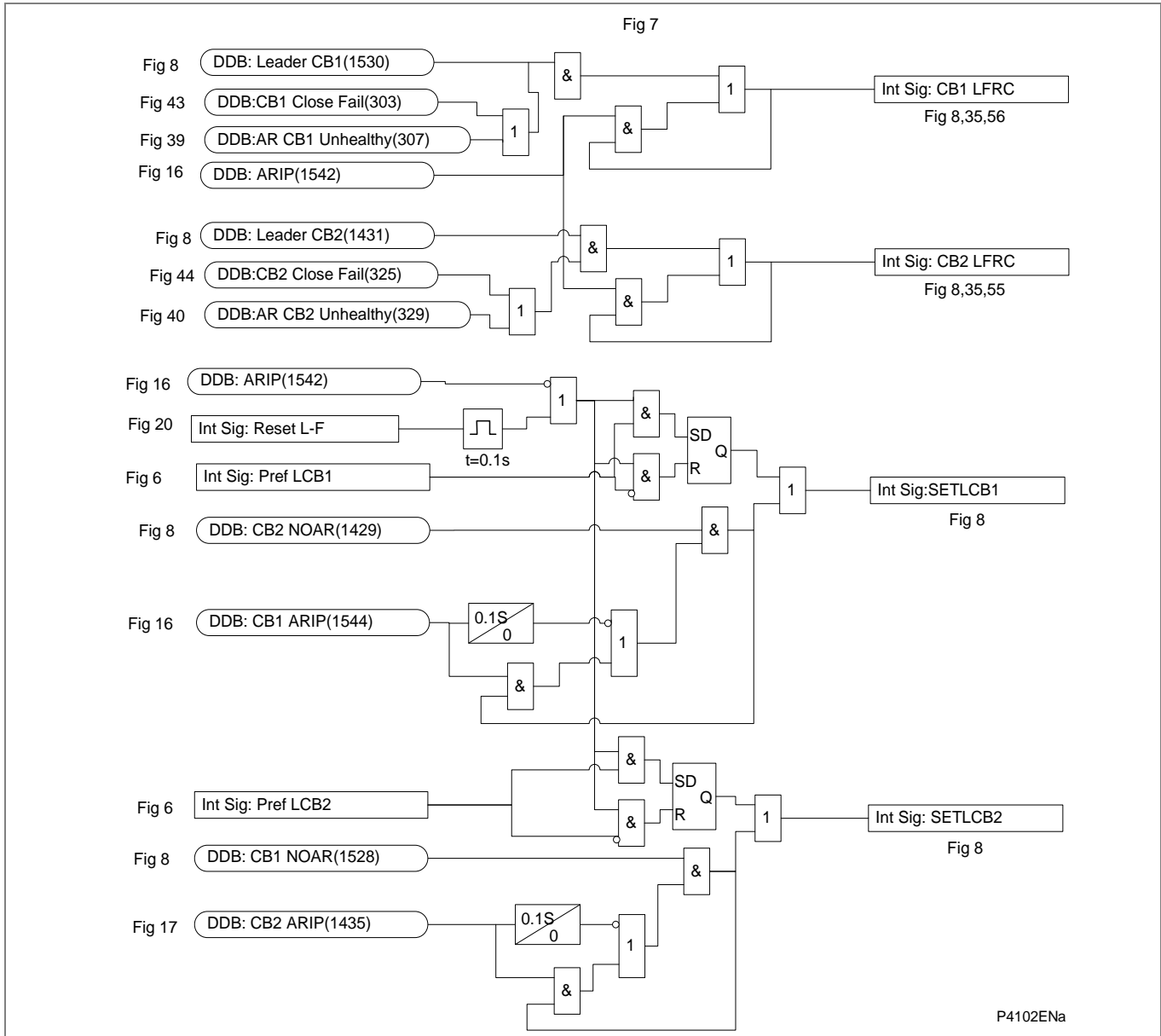
Figure AR-7 - Leader/follower logic – 1 (for Software Versions BEFORE H1)
