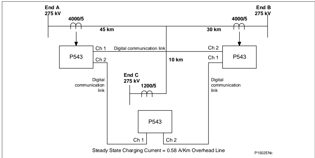
Figure 26 - Typical teed feeder application
