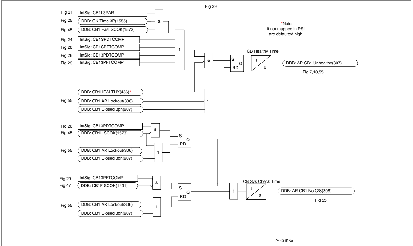
Figure AR-38 - CB healthy & system check timers
