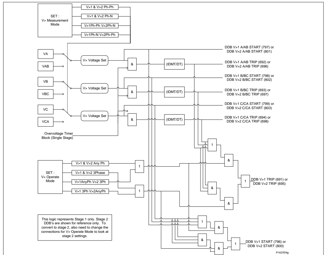
Figure 67 - Undervoltage - single and three-phase tripping mode (single stage)
