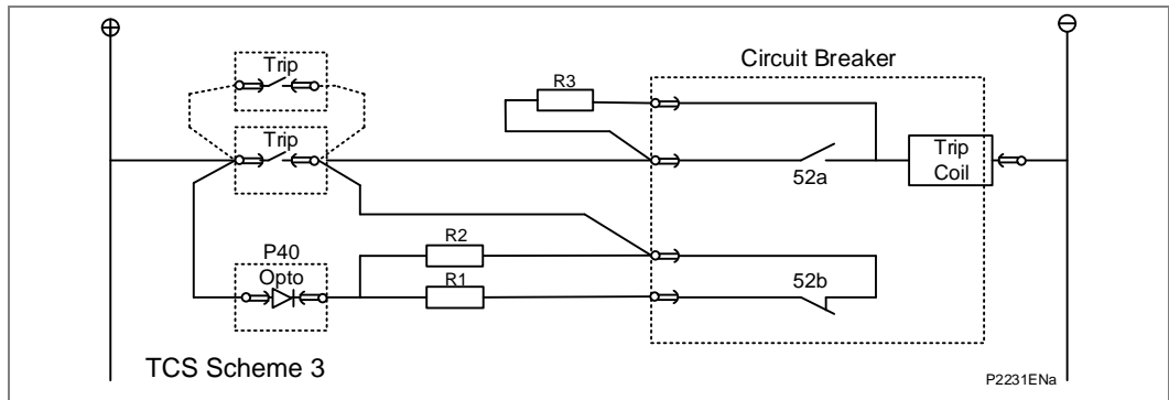
Figure 37 - TCS scheme 3
