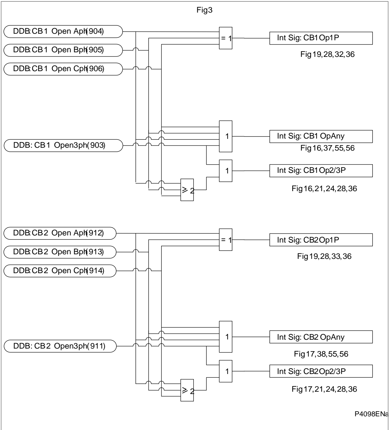
Figure AR-3 - CB1 & CB2 Open 1P, 2P, 2/3P, Any
