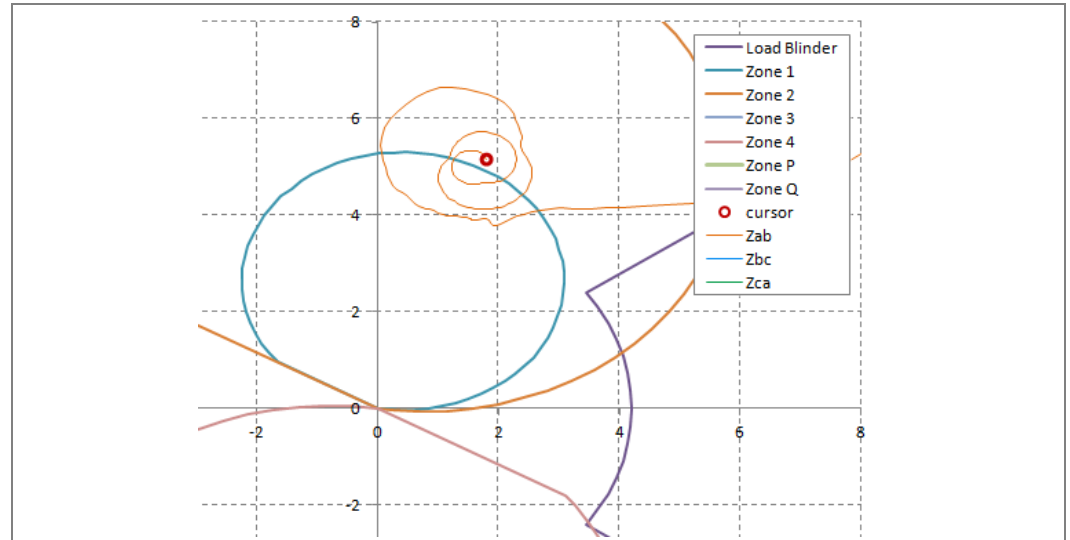
Figure 19 - Apparent impedance with sub-synchronous oscillations effecting zone 1 operation (simulated data)
