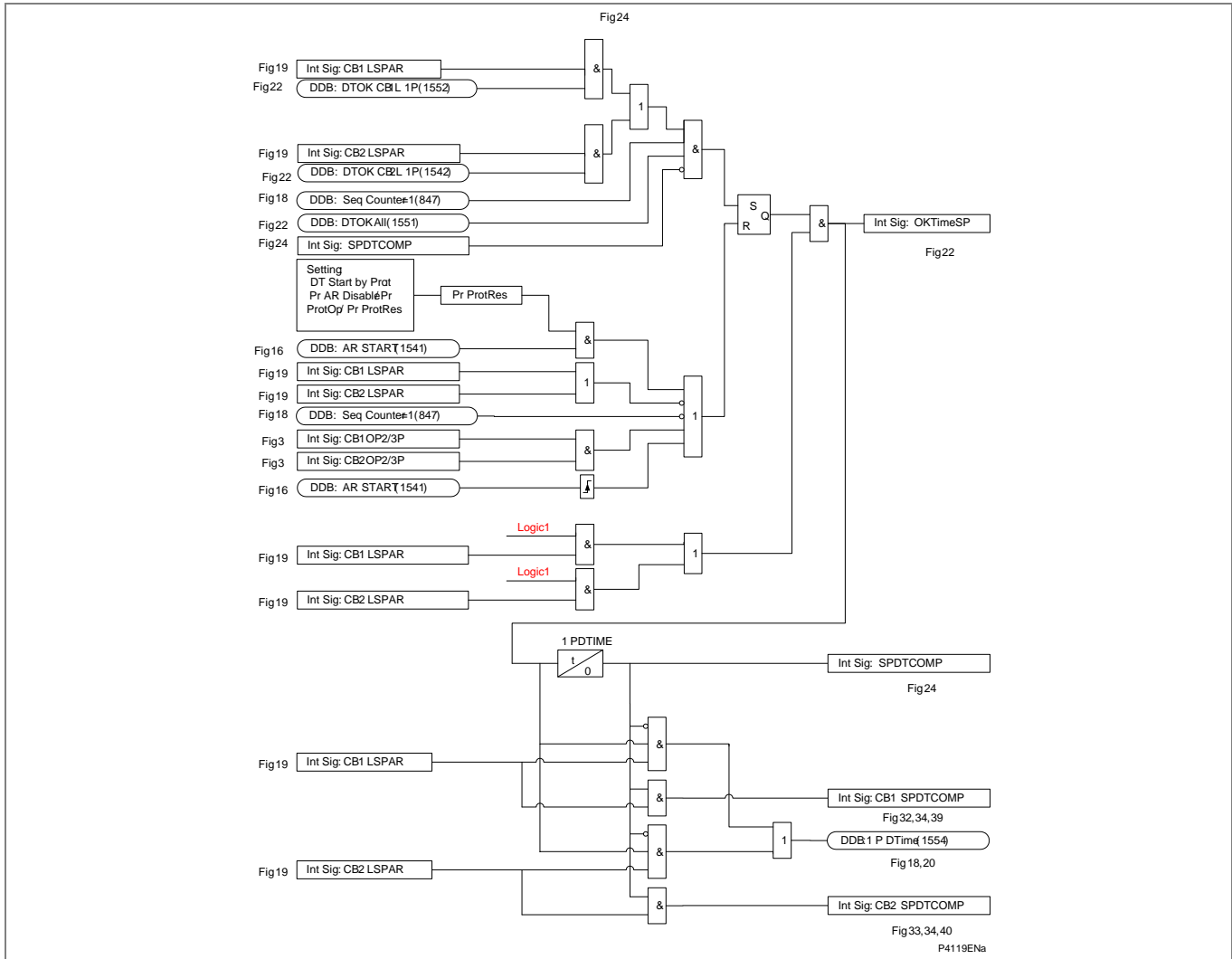
Figure AR-24 - Single phase AR lead CB dead time
