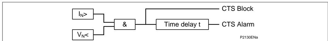
Figure 103 - Voltage dependant CTS principle scheme
