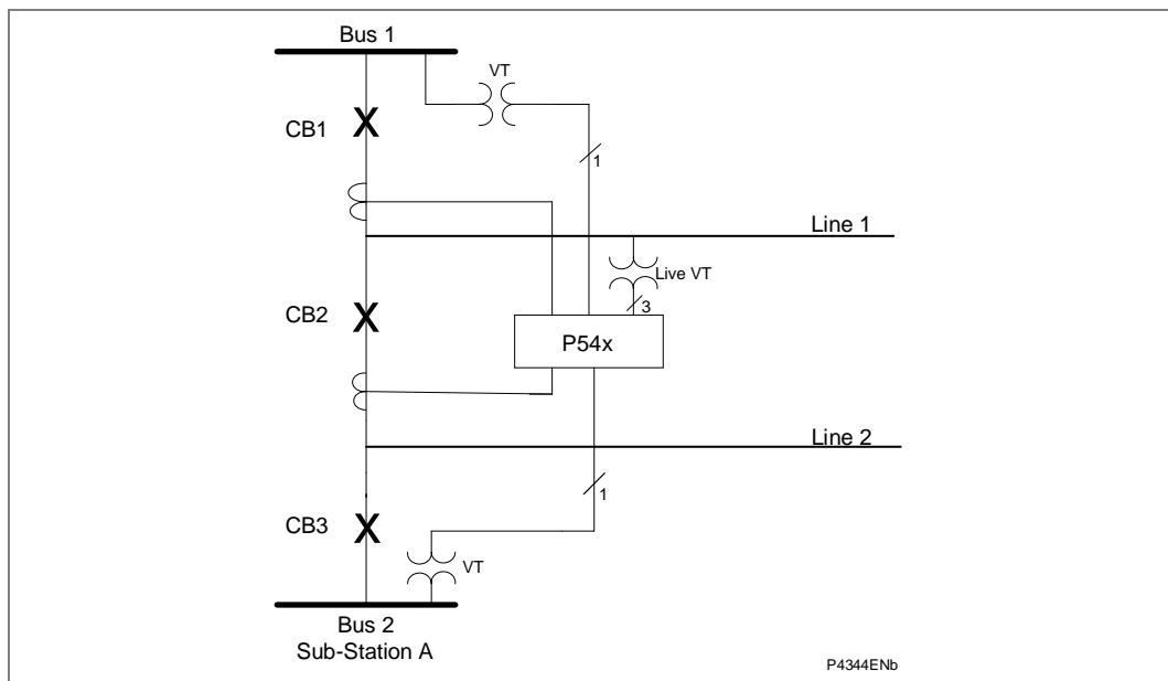
Figure 39 - Two circuit breaker auto-reclose application
