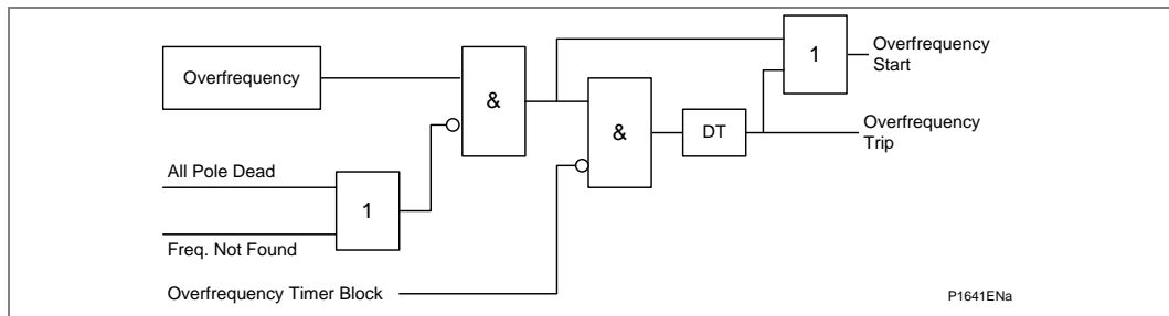
Figure 76 - Overfrequency logic (single stage)
