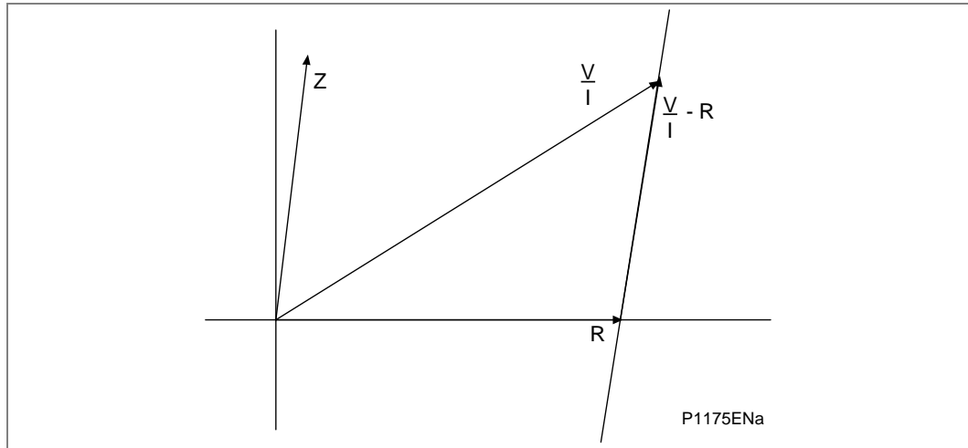
Figure 26 - Resistive reach line (load blinder) (Distance option only)
