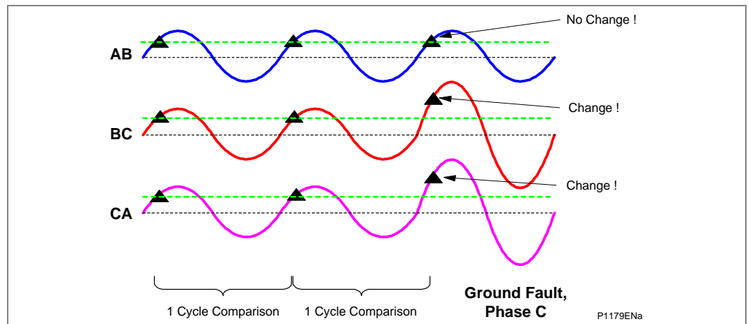
Figure 21 - Phase to phase currents showing change for CN fault
