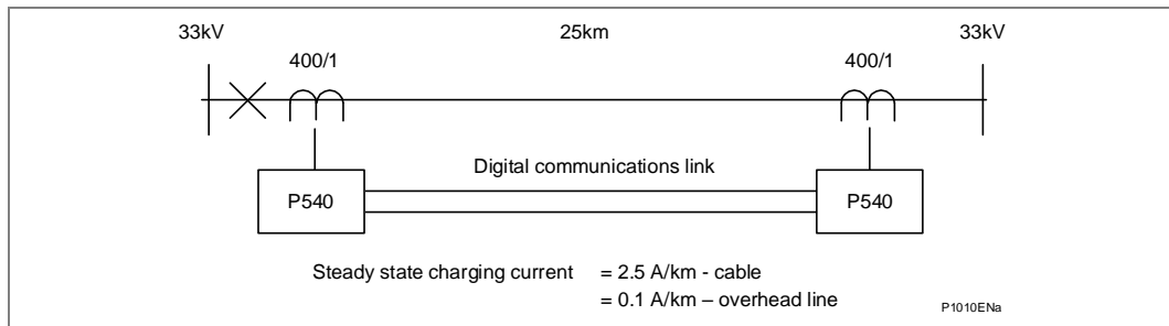
Figure 24 - Typical plain feeder circuit
