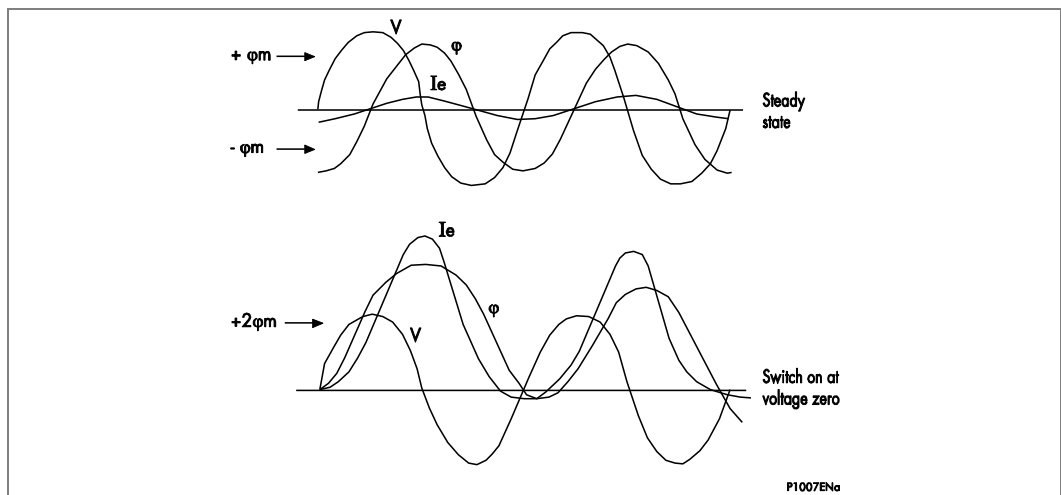
Figure 8 - Magnetizing inrush waveforms
