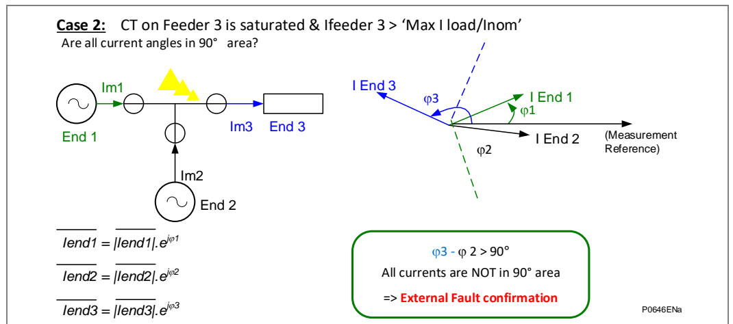
Figure 2 - Differential 3-terminal scheme - external fault
