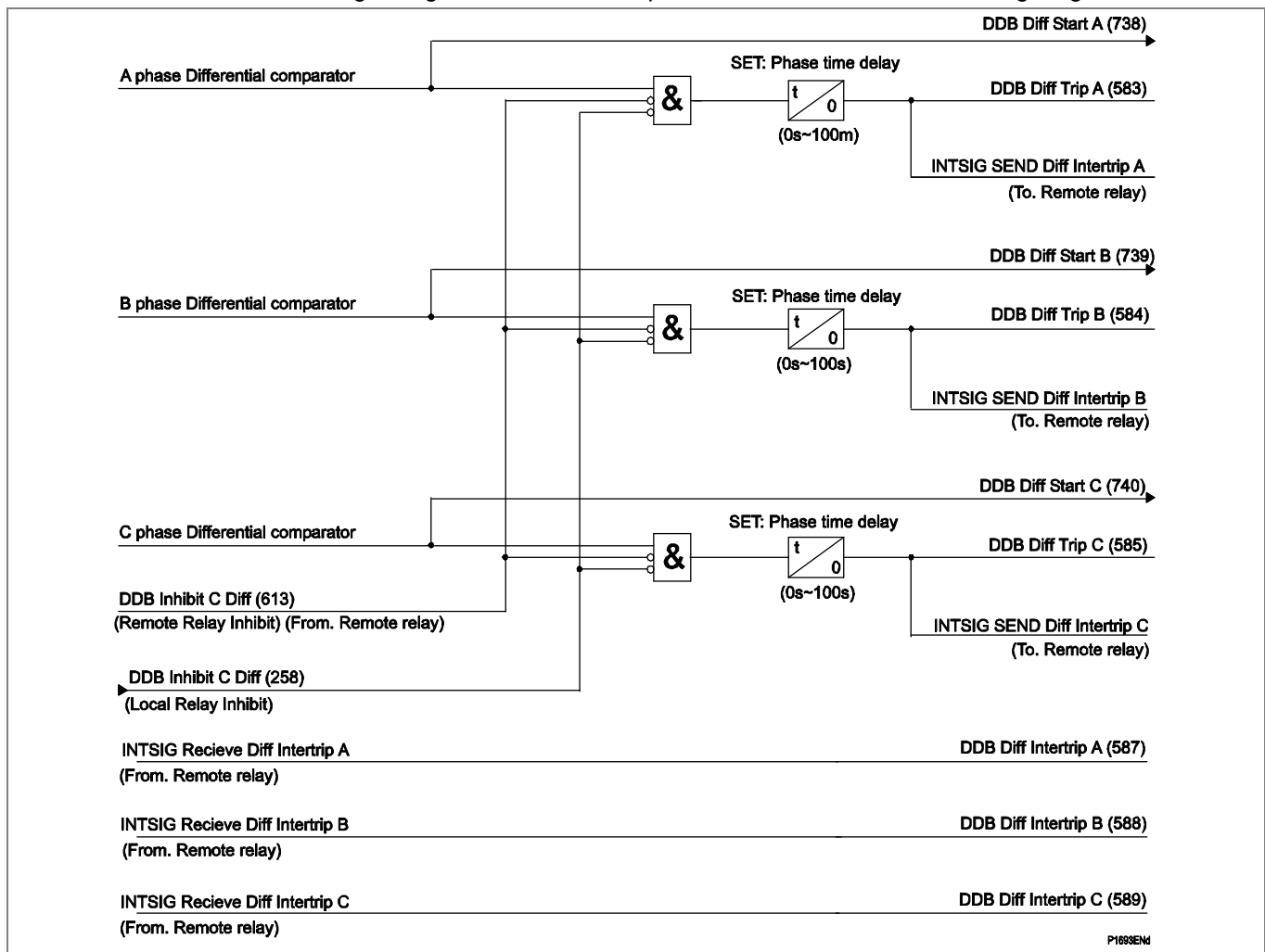
Figure 2 - Differential logic diagram
