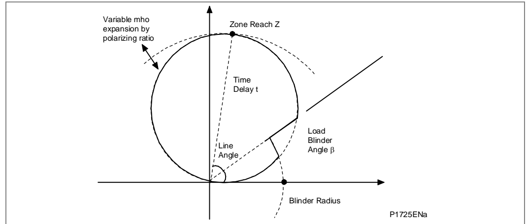
Figure 9 - Settings required to apply a Mho zone (Distance option only)
