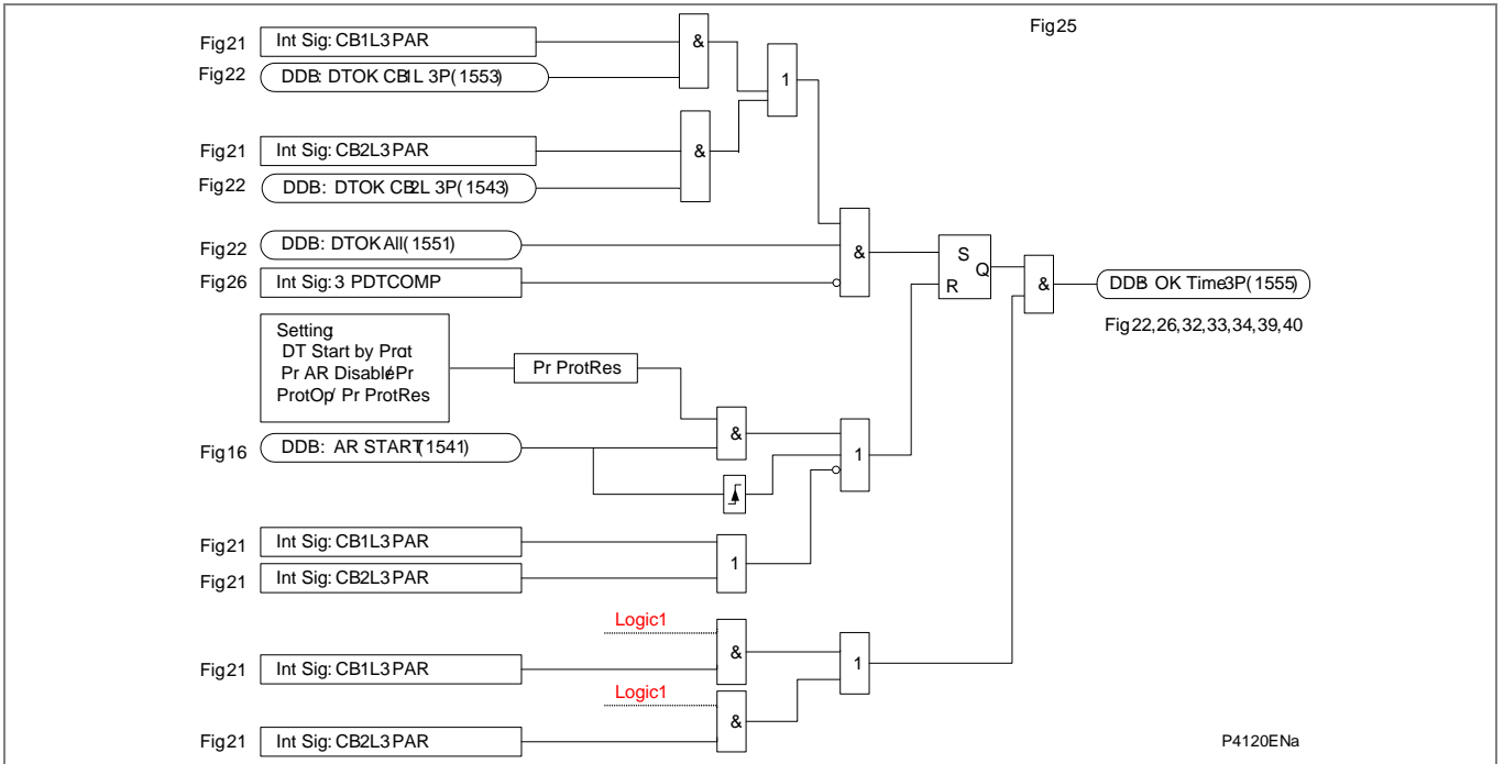
Figure AR-25 - Three phase AR lead CB dead time enable
