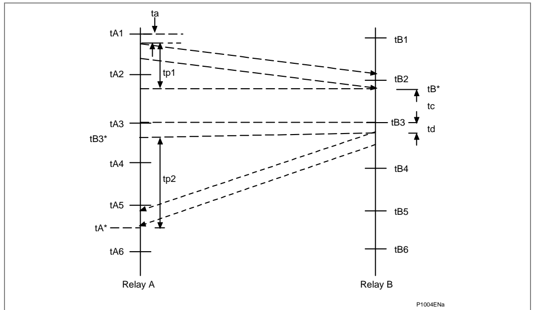
Figure 5 - Data transmission
