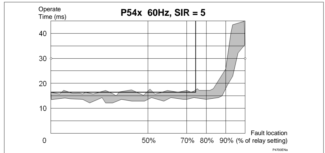
Figure 2 - Operating Time vs Reach % at 60 Hz
