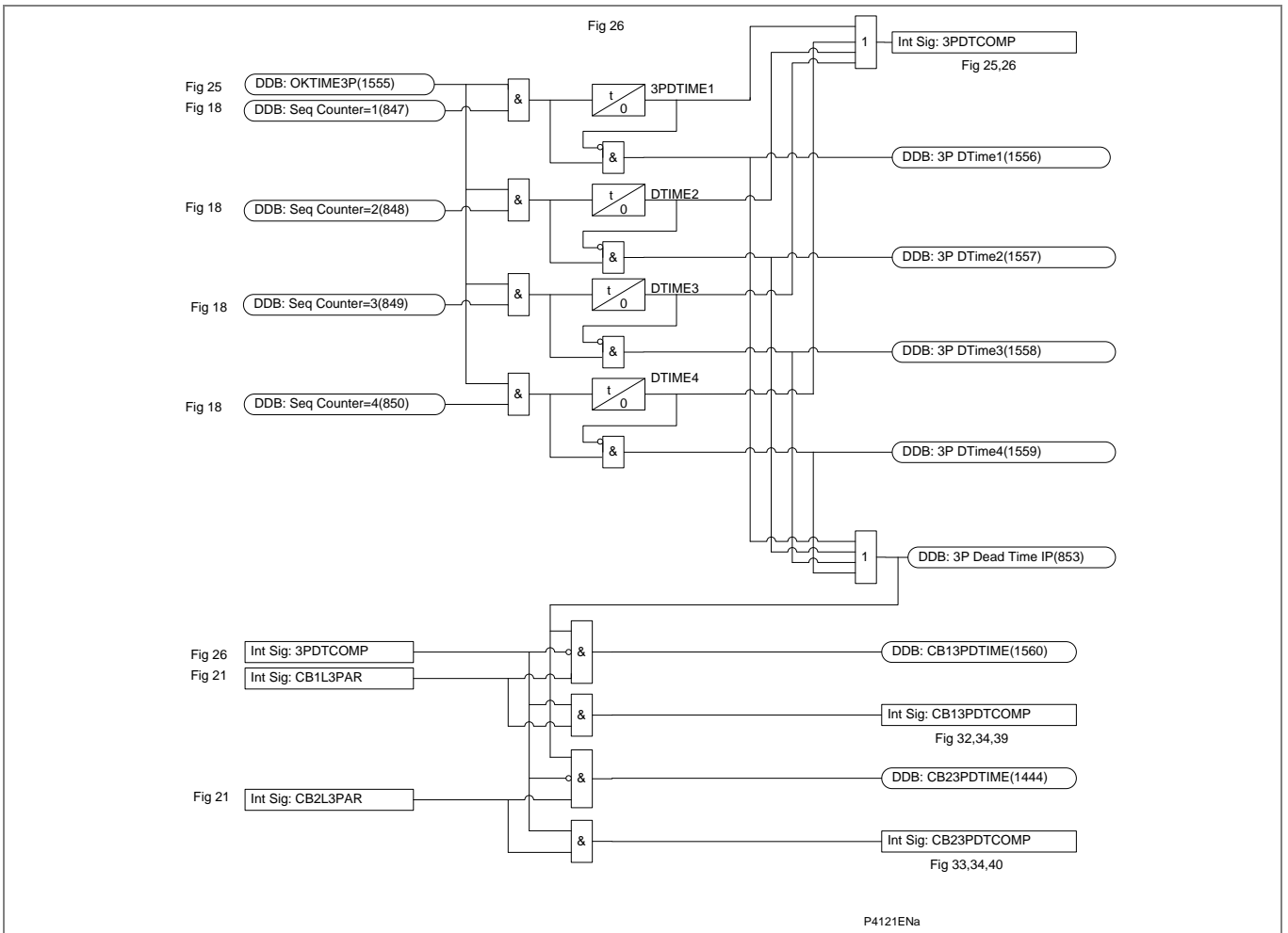
Figure AR-26 - Three phase AR lead CB dead time
