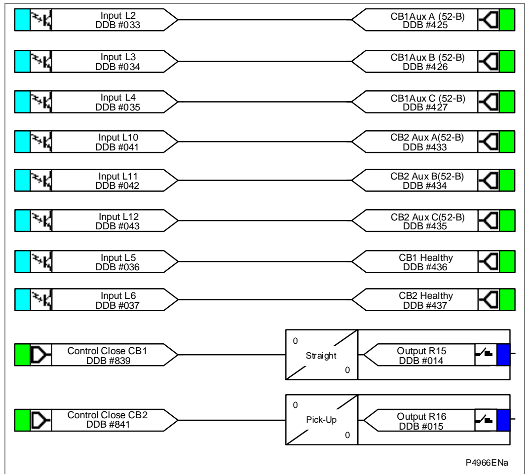
Figure 40 - PSL mapping of some of the opto inputs and relay outputs
