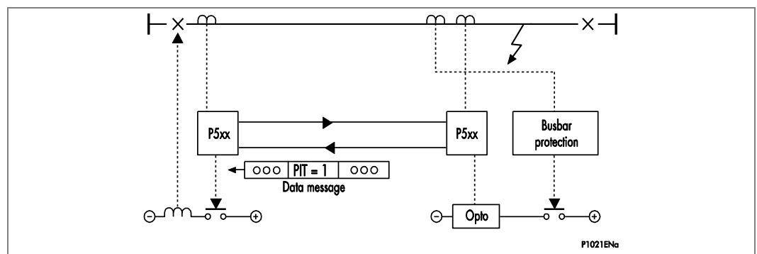
Figure 98 - Permissive intertrip
