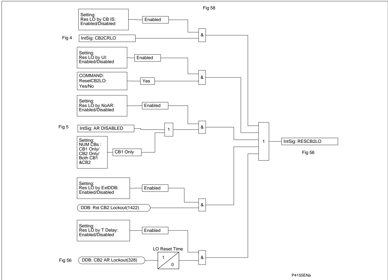
Figure AR-59 - Reset CB2 lockout
