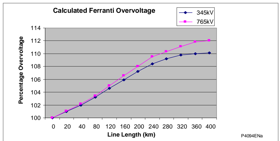
Figure 21 - Calculated Ferranti voltage rise on 345 kV and 765 kV lines
