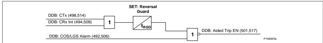
Figure 47 - Blocking 2 (Distance option only)
