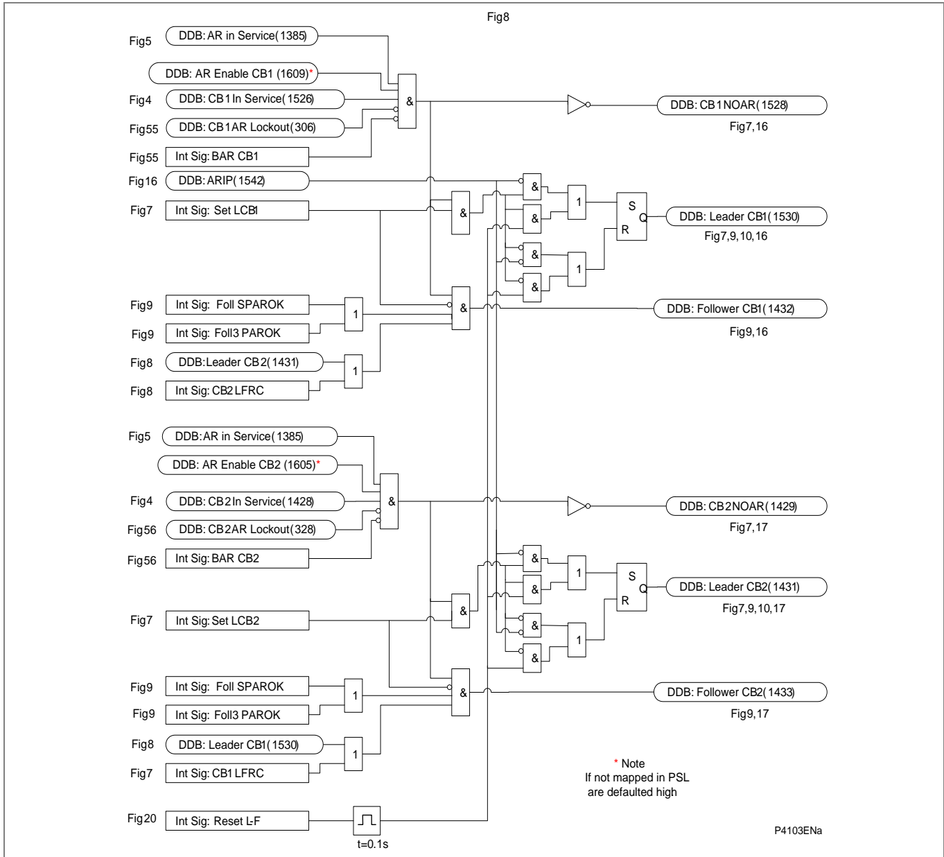
Figure AR-9 - Leader/follower logic – 2
