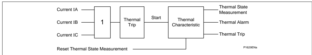
Figure 59 - Thermal overload protection logic diagram
