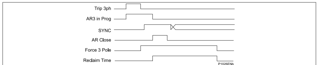
Figure 109 - Auto-reclose timing diagram - fault with system synchronism
