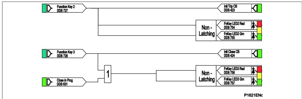
Figure 135 - Circuit breaker control via function keys default PSL
