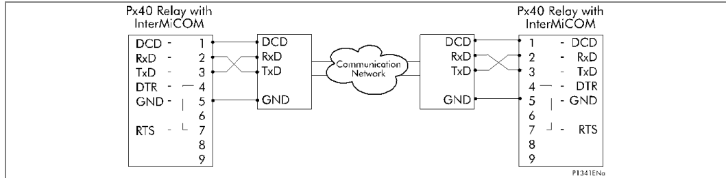
Figure 93 - InterMiCOM teleprotection via a MODEM link
