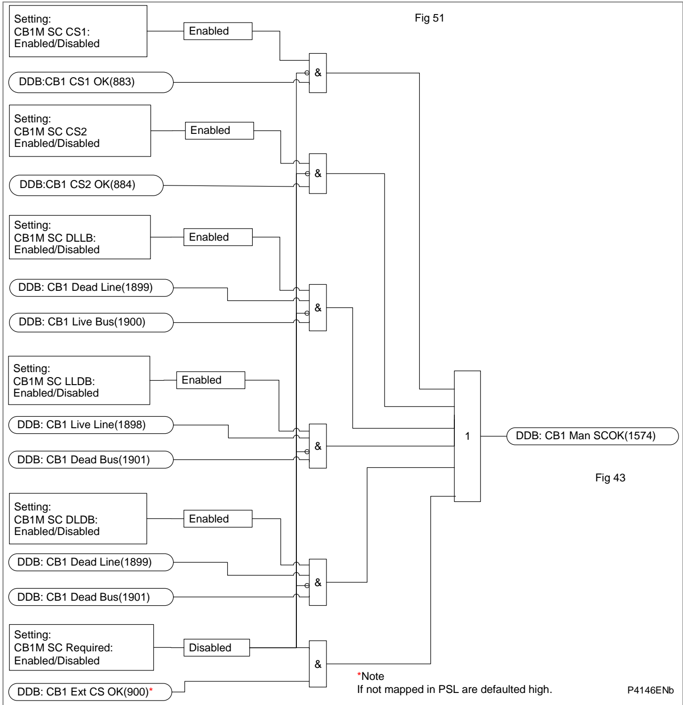
Figure AR-48 - CB1 man. close system check
