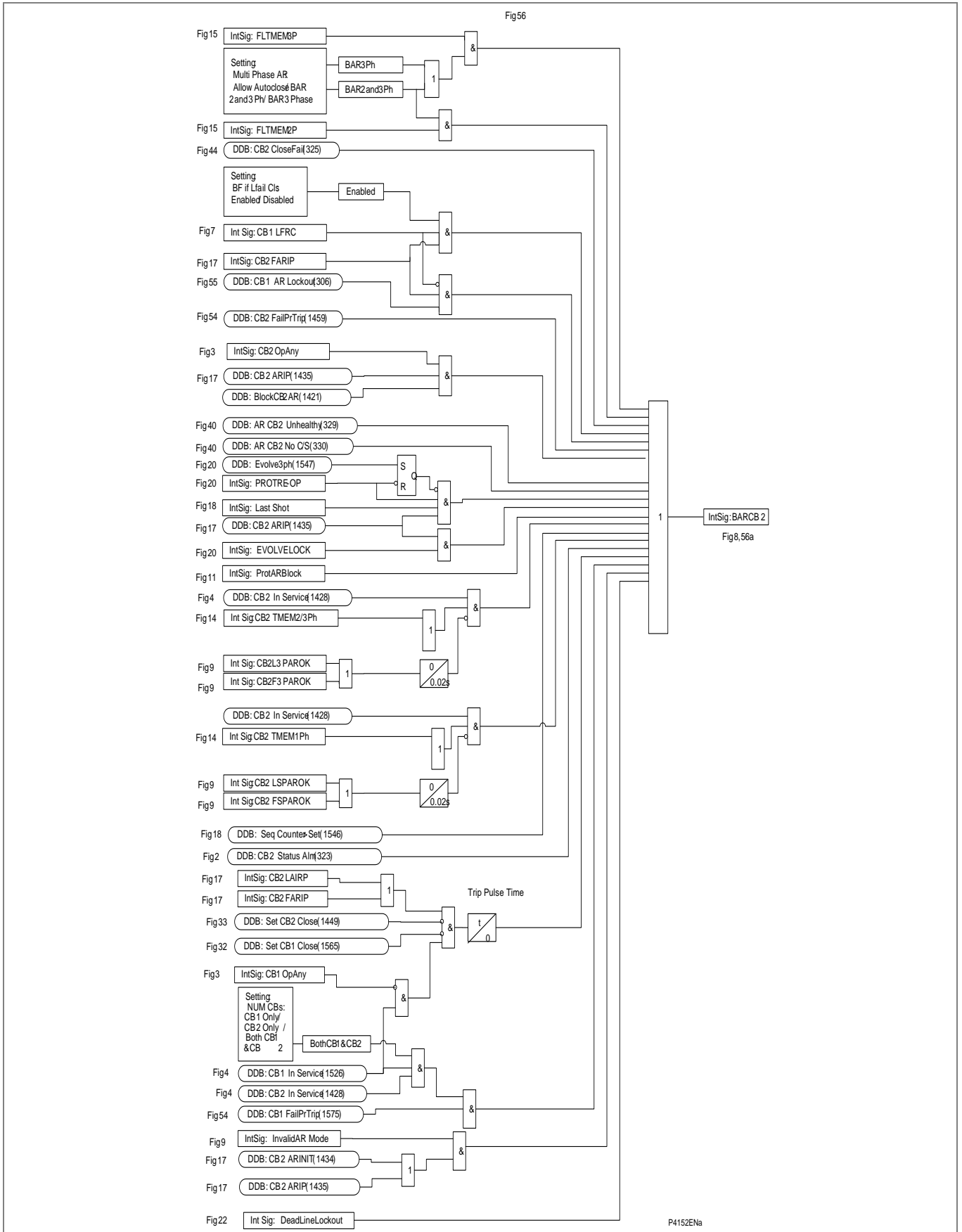
Figure AR-55 - Auto-reclose lockout – CB2 (for Software Versions BEFORE H1)
