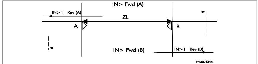
Figure 50 - DEF blocking scheme (Distance option only)
