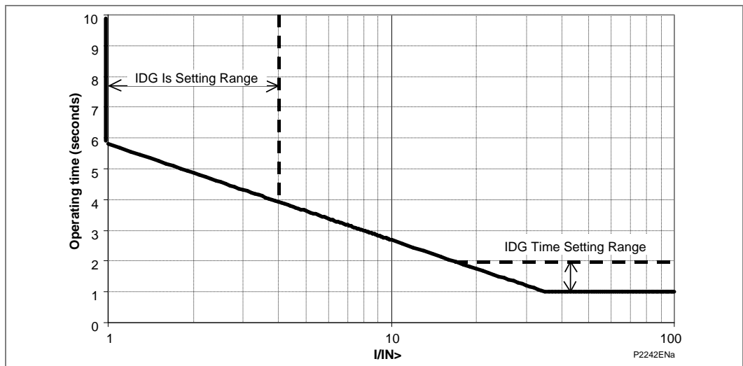
Figure 60 - IDG characteristic
