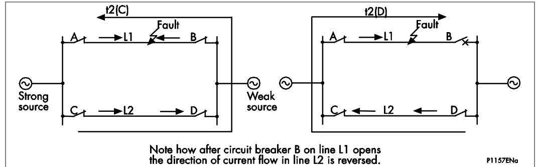
Figure 45 - Example of fault current reverse of direction
