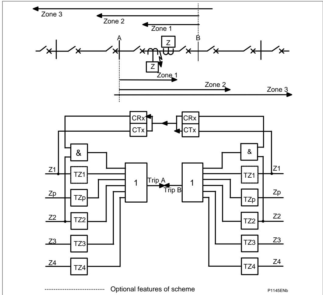
Figure 40 - Permissive underreach transfer trip scheme (PUR) (Distance option only)
