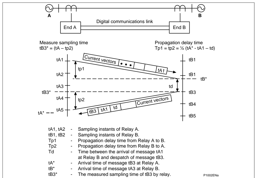
Figure 3 - Propagation delay measurement
