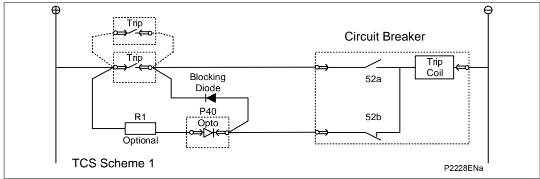
Figure 31 - TCS scheme 1
