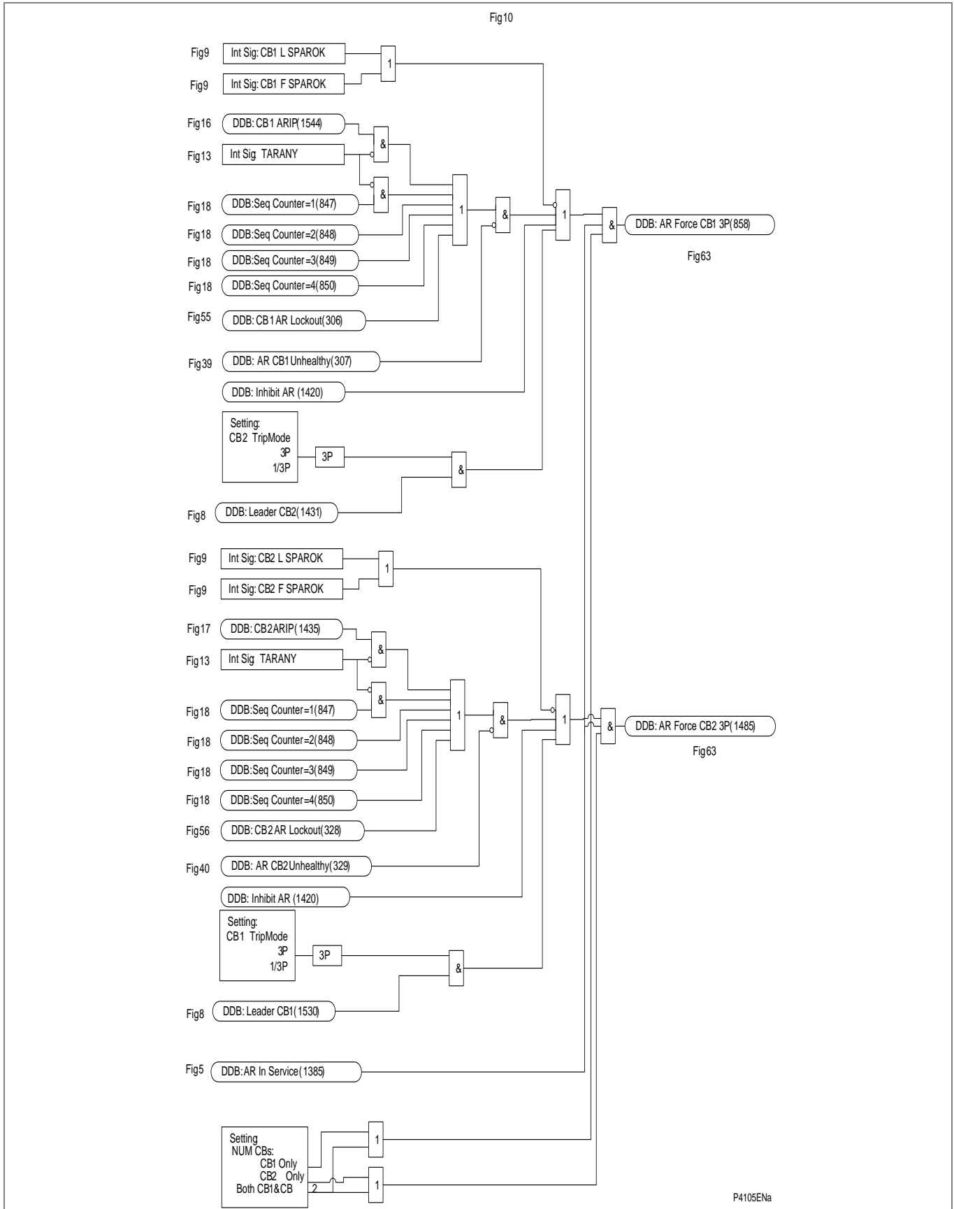
Figure AR-11 - Force three-phase trip
