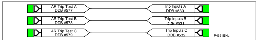
Figure 2 - Auto-reclose default PSL - P544 & P546 SW ver 45 and 55
