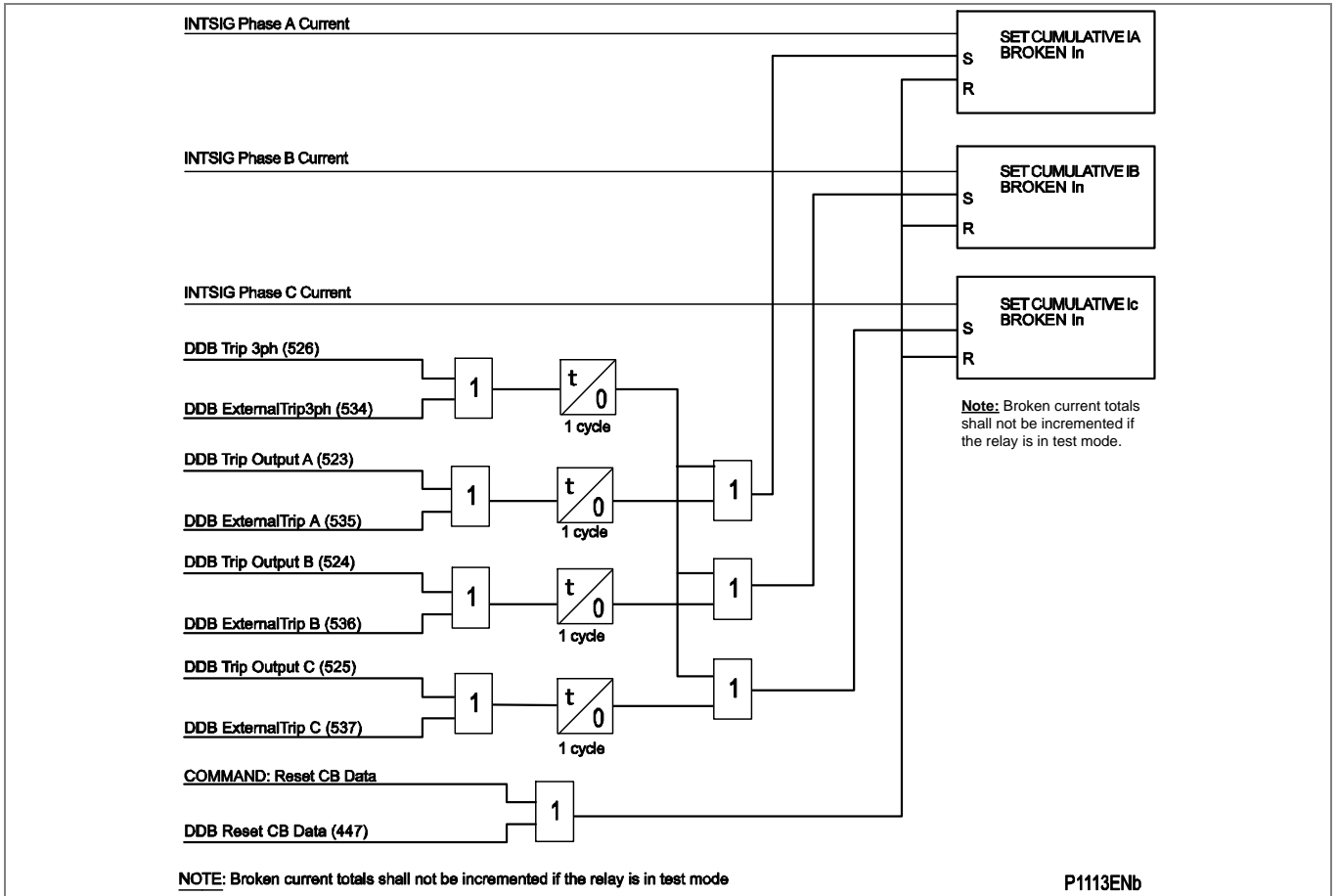
Figure 121 - Circuit breaker condition monitoring - broken current (P543/P545)
