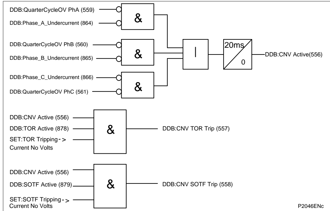
Figure 34 - Trip on close based on CNV level detectors (Distance option only)
