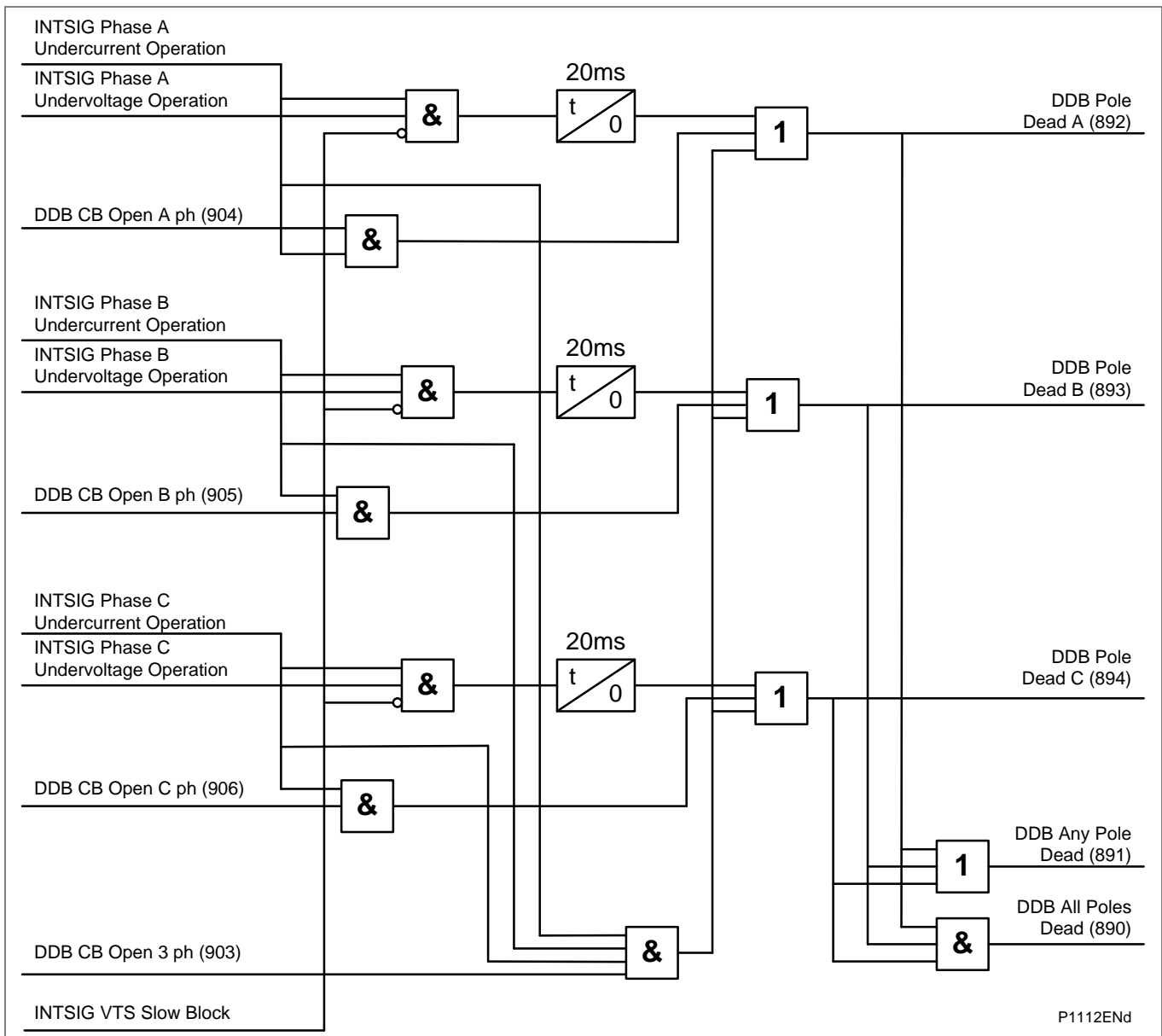
Figure 16 - Pole dead logic for P543/P545
