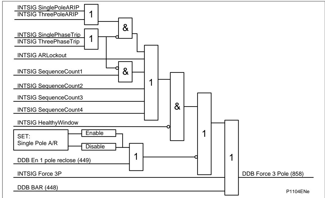
Figure 117 - Auto-reclose force 3-pole trip (P543/P545)
