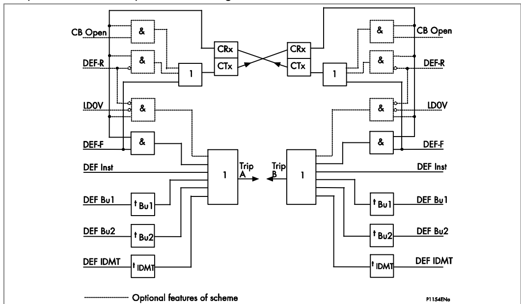
Figure 49 - Aided DEF (ground) permissive scheme logic (Distance option only)
