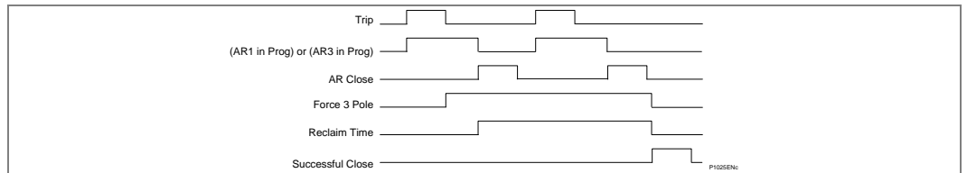
Figure 108 - Auto-reclose timing diagram - repeated fault inception
