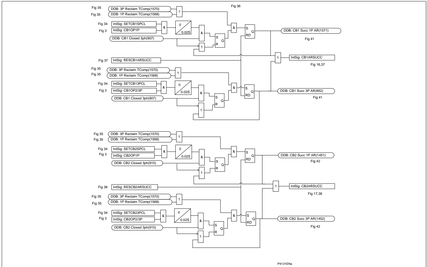
Figure AR-35 - Successful auto-reclose signals
