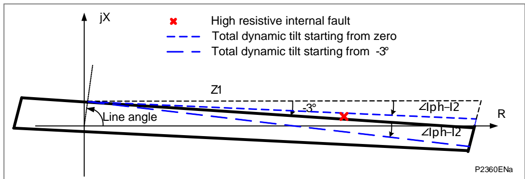
Figure 11 - Example of a high resistive zone 1 fault that falls outside zone 1 characteristic when the starting tilt angle of -3^\circ is set (over-tilting effect)
