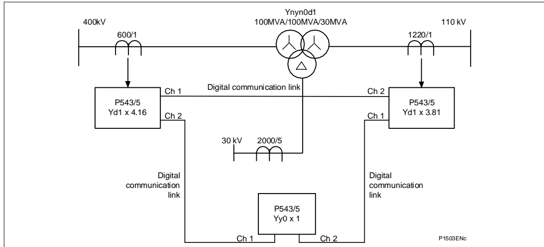
Figure 27 - Three winding transformer in zone application
