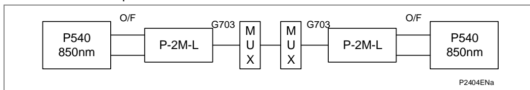
Figure 88 - P54x connection to P-2M-L
