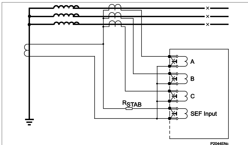
Figure 62 - High impedance REF relay/CT connections
