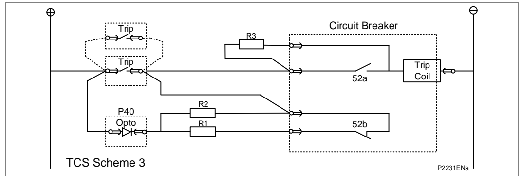
Figure 26 - TCS scheme 3
