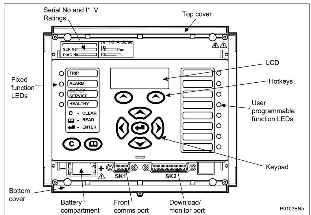
Figure 1 - Relay front view (40TE case for )
