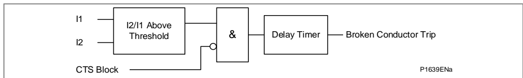
Figure 64 - Broken conductor logic
