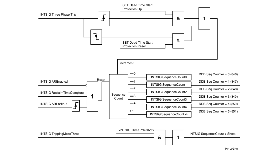
Figure 75 - Auto-reclose inhibit sequence count
