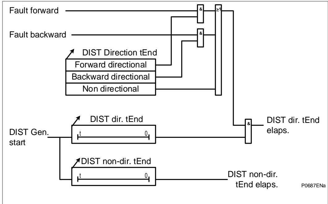
Figure 8 - Distance protection logic
