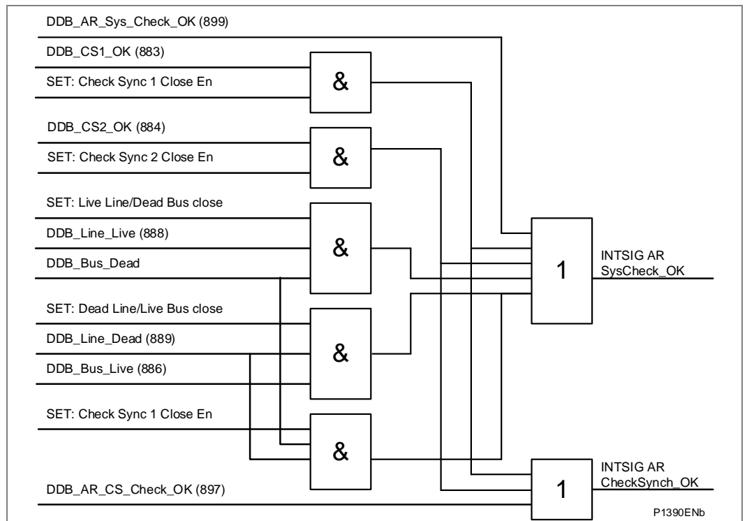
Figure 80 - Auto-reclose/check sync interface
