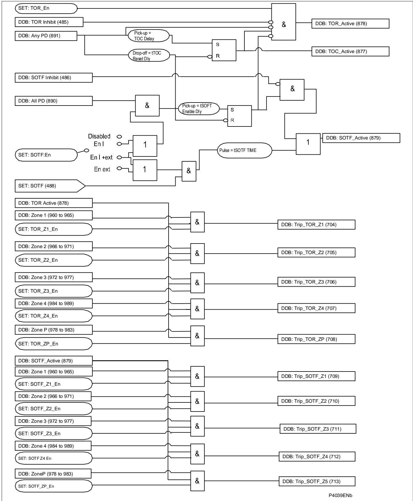
Figure 15 - Trip on close
