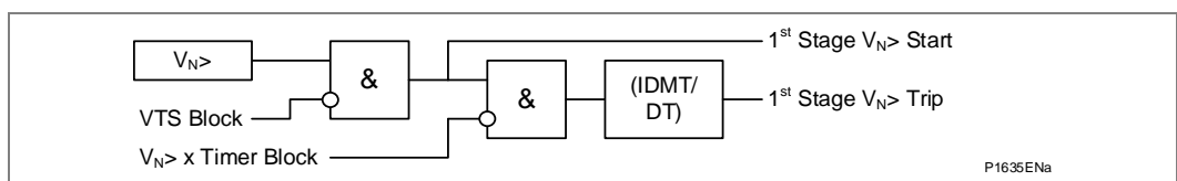
Figure 60 - Residual overvoltage logic (single stage)
