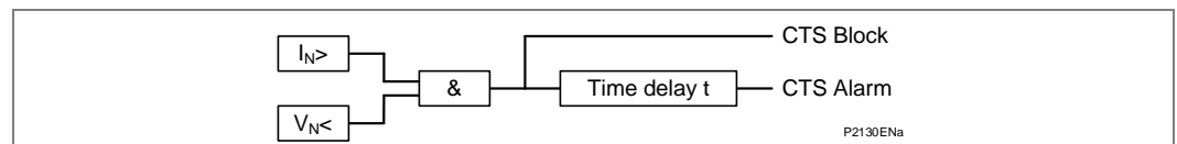
Figure 82 - Voltage dependant CTS
