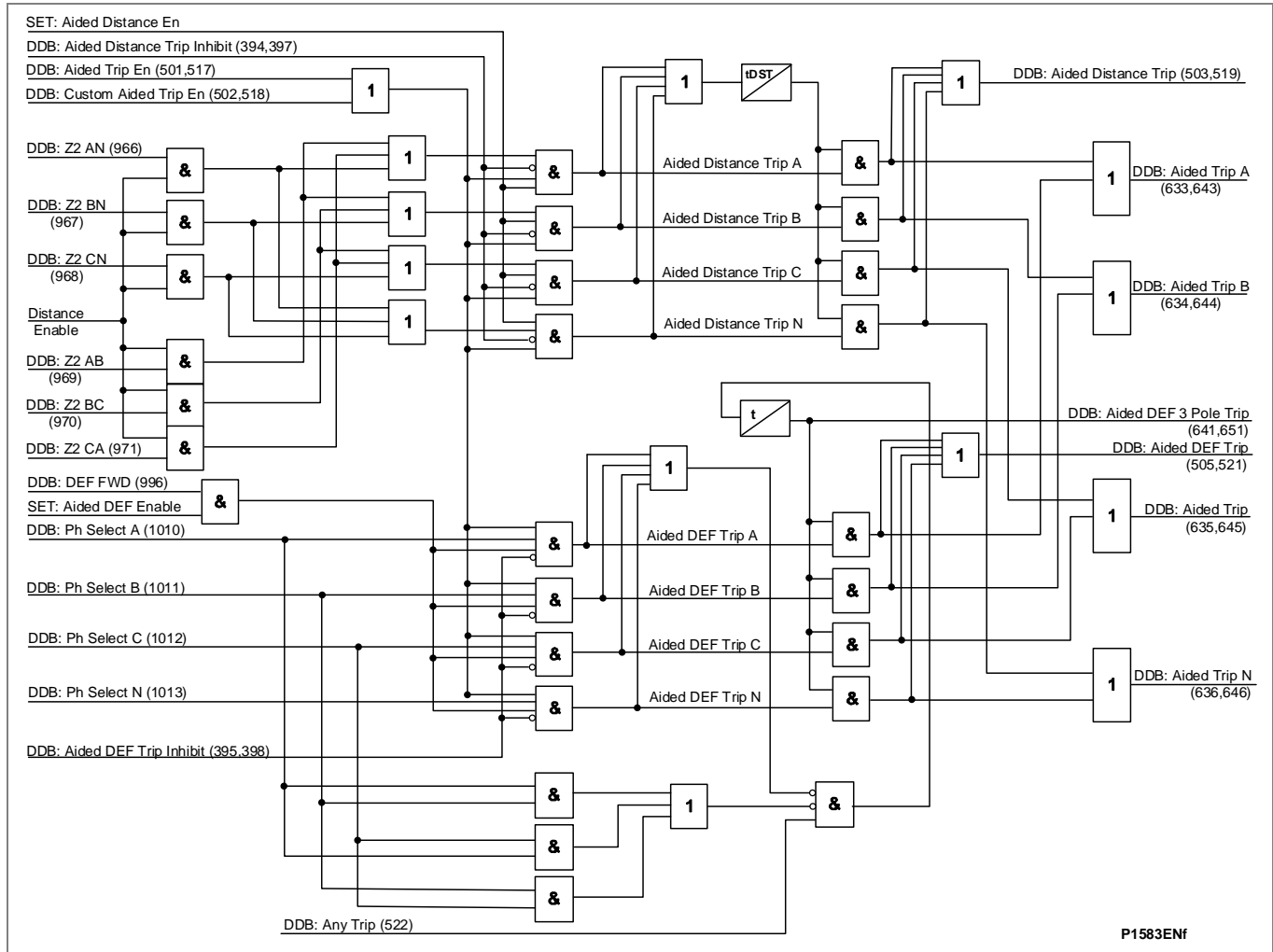
Figure 21 - Aided tripping logic
