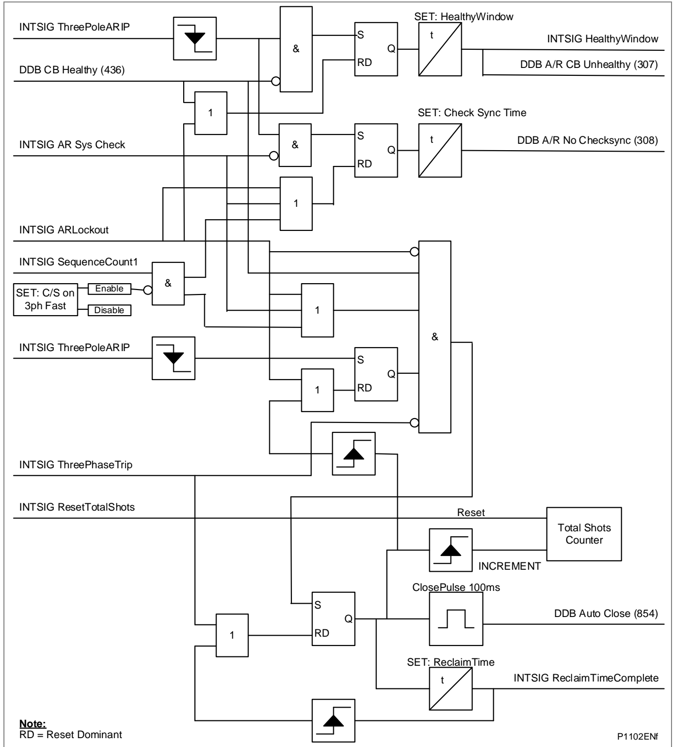
Figure 77 - Auto-reclose close
