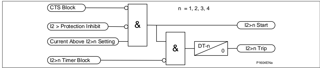
Figure 55 - Negative sequence overcurrent non-directional operation
