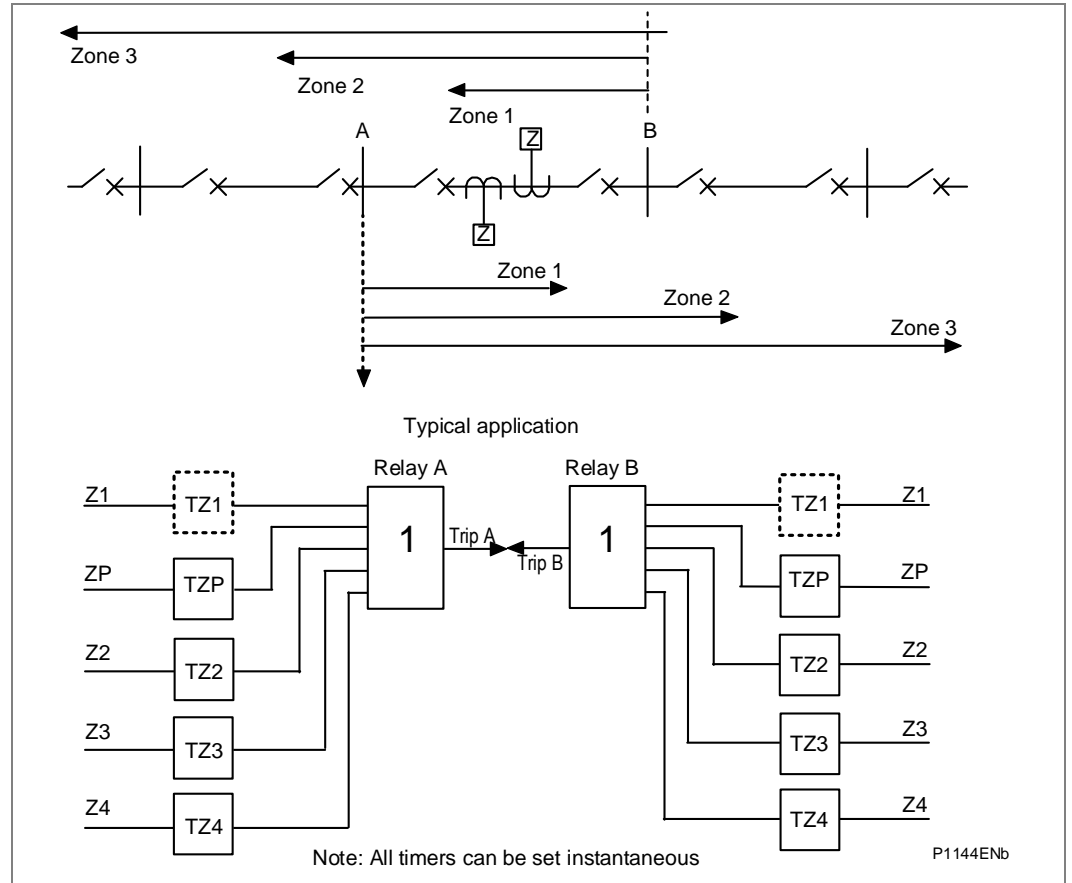
Figure 9 - Basic time stepped distance scheme
