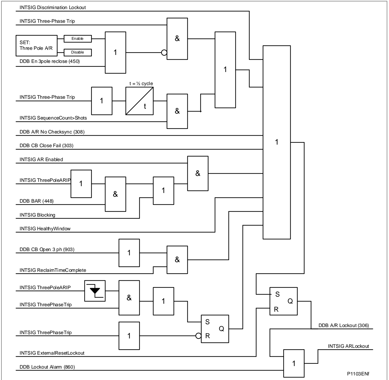
Figure 78 - Auto-reclose lockout logic
