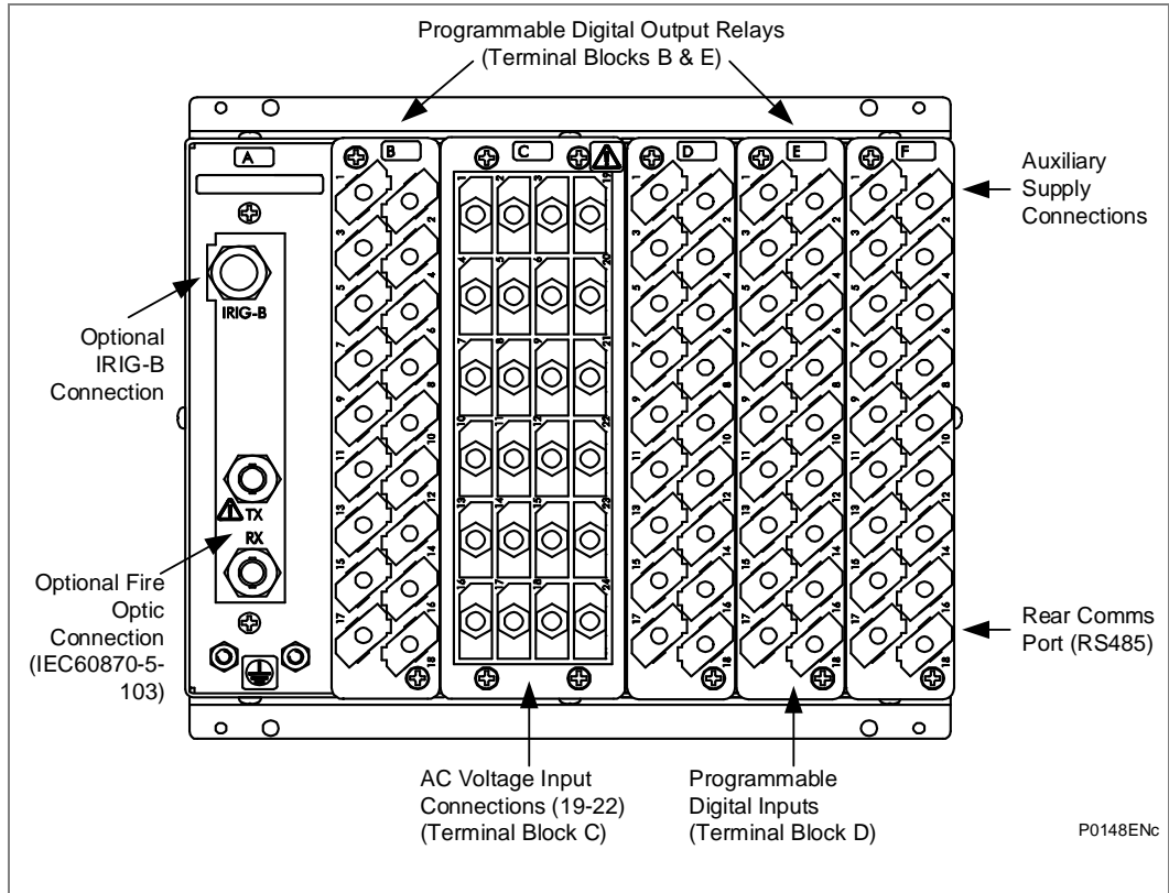
Figure 1 - Rear terminal blocks on size 40TE case
