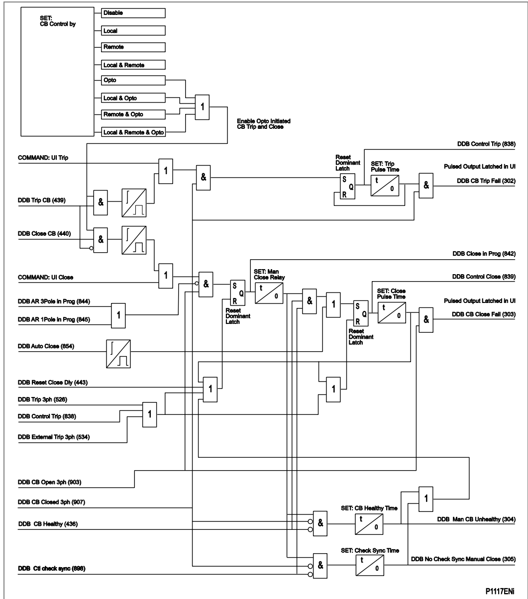
Figure 88 - Circuit breaker control
