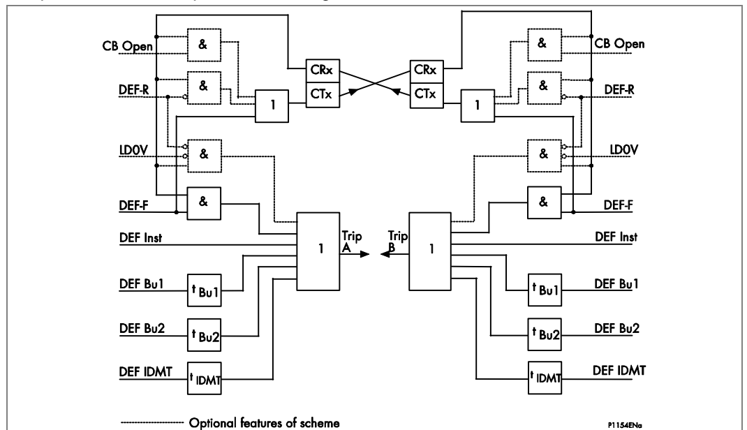
Figure 31 - Aided DEF (ground) permissive scheme logic
