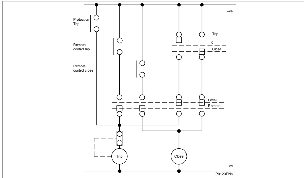
Figure 87 - Remote control of circuit breaker
