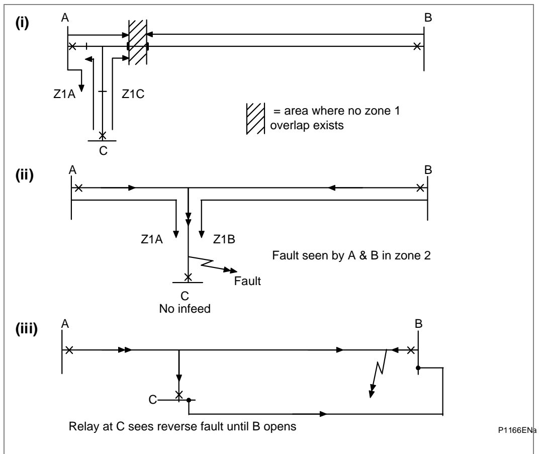
Figure 19 - Teed feeder applications
