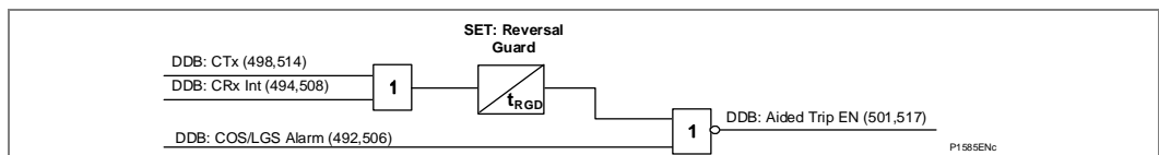
Figure 29 - Blocking 2
