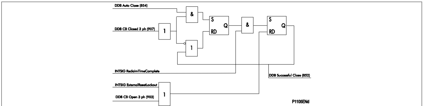
Figure 79 - Auto-reclose close notify
