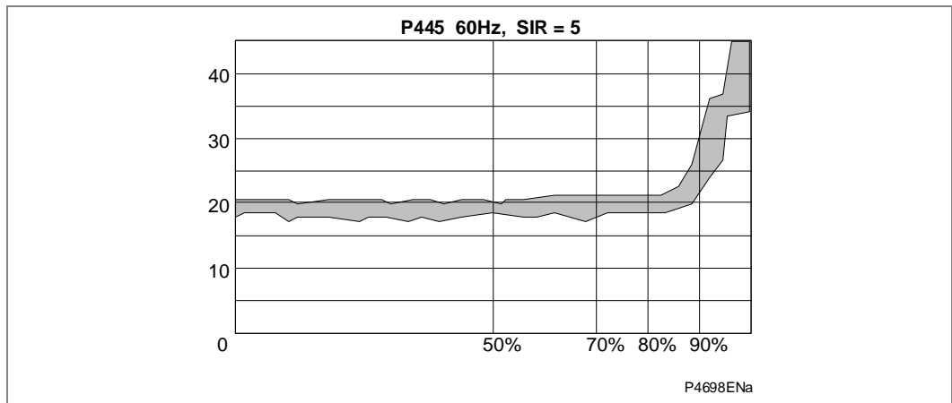
Figure 2 - Operating Time vs Reach % at 60 Hz
