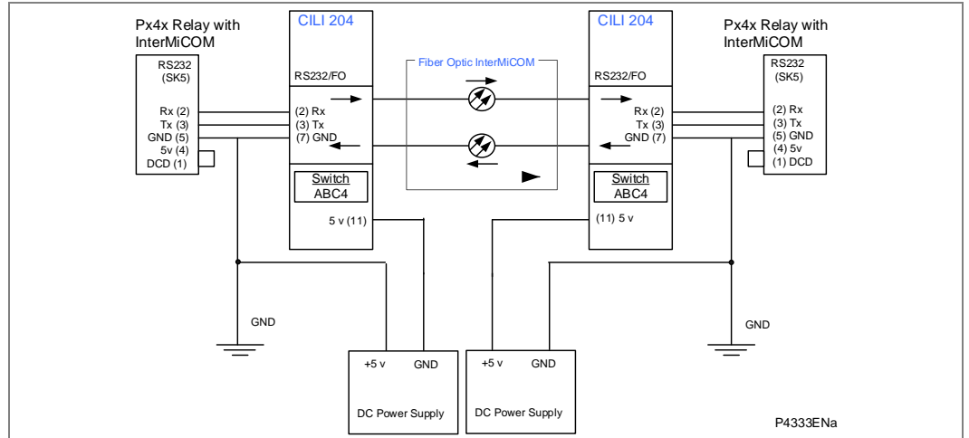
Figure 42 - MODEM InterMiCOM teleprotection via fiber optic
