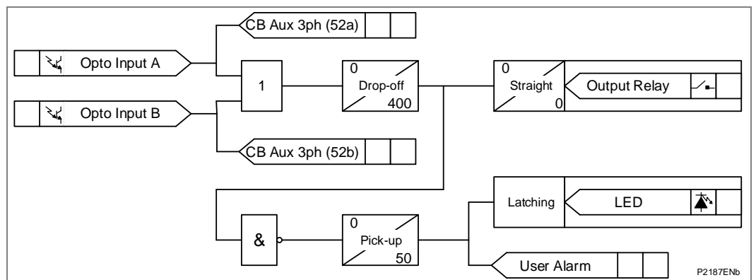
Figure 23 - PSL for TCS schemes 2a
