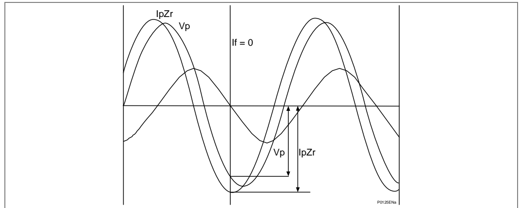
Figure 90 - Fault locator selection of fault current zero
