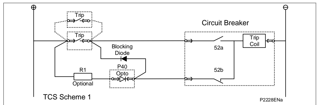
Figure 20 - TCS scheme 1
