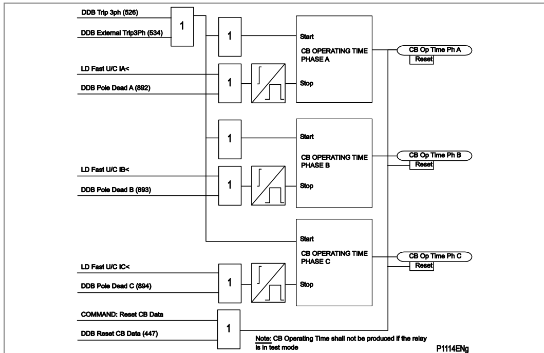
Figure 85 - Circuit breaker condition monitoring - operation time
