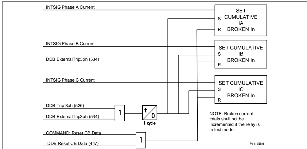
Figure 84 - Circuit breaker condition monitoring - broken current
