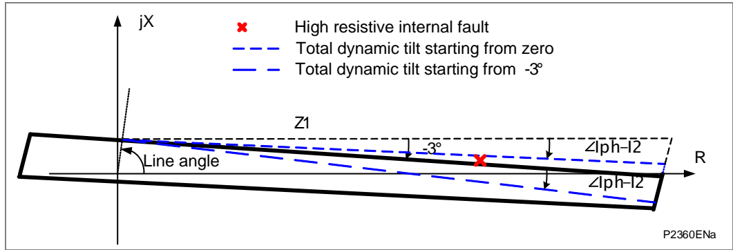
Figure 4 - Example of high resistive zone 1 fault that falls outside zone 1 characteristic when the starting tilt angle of -3° is set (over-tilting effect)
