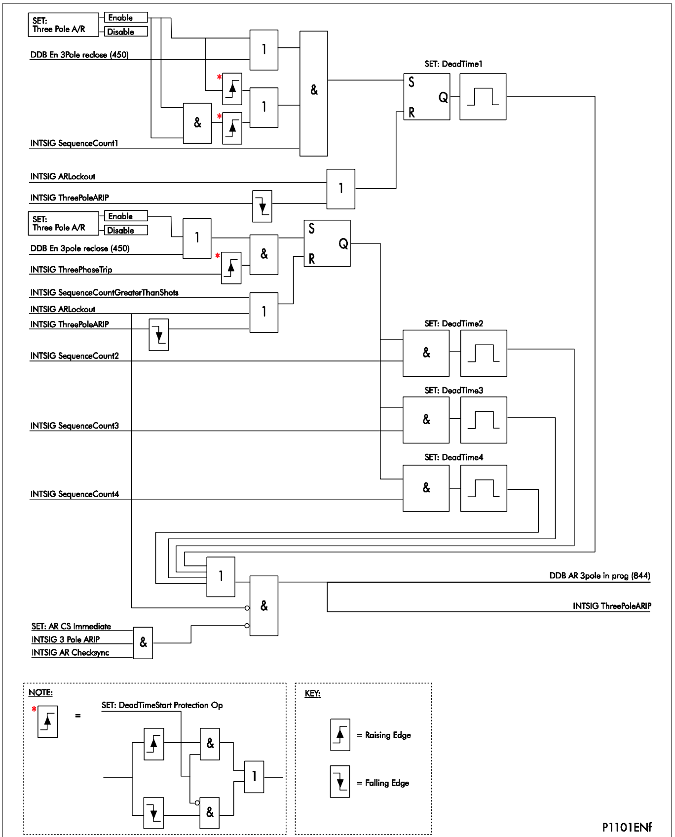
Figure 76 - Auto-reclose cycles
