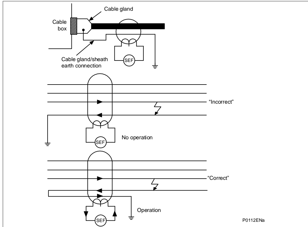
Figure 13 - Positioning of core balance current transformers
