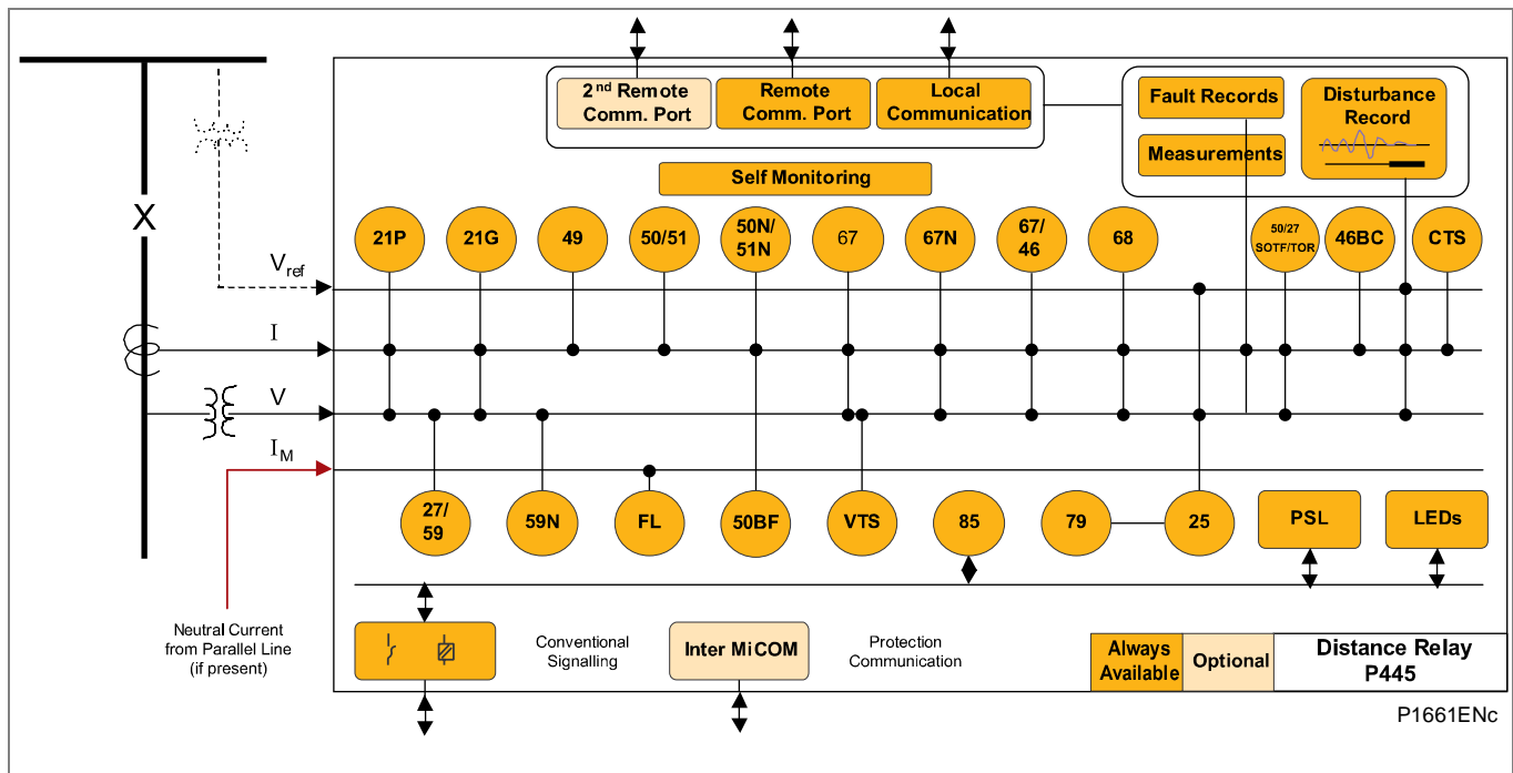
Figure 1 - Functional diagram
