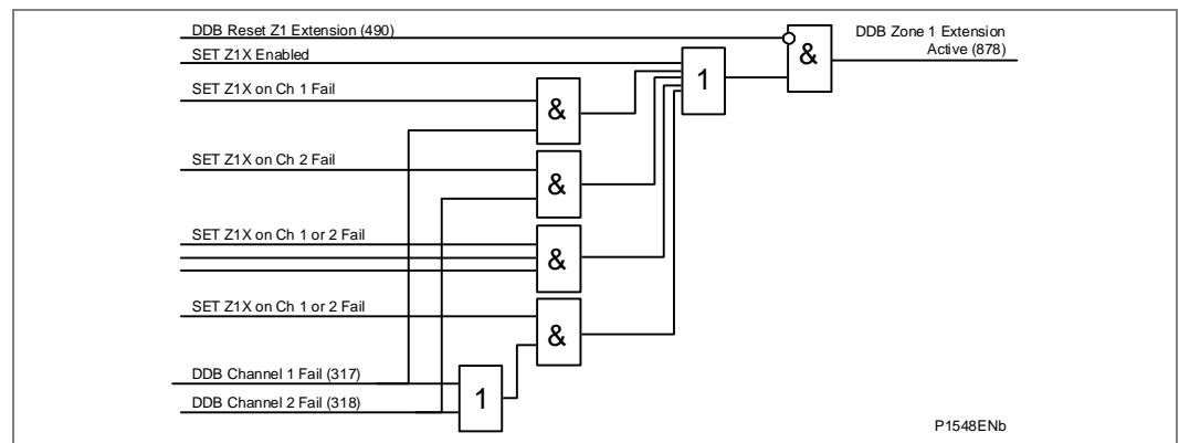
Figure 35 - Zone 1 extension
