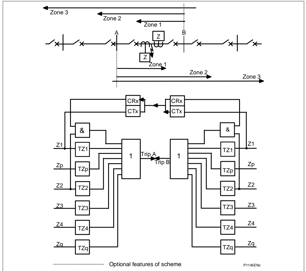
Figure 22 - Permissive underreach transfer trip scheme (PUR)
