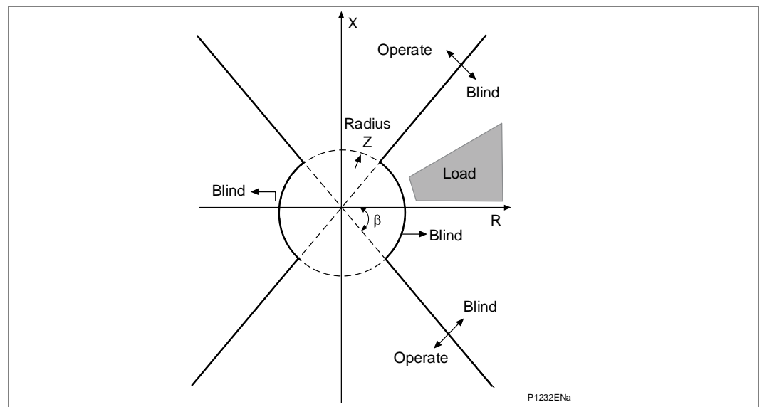
Figure 11 - Load blinder characteristics
