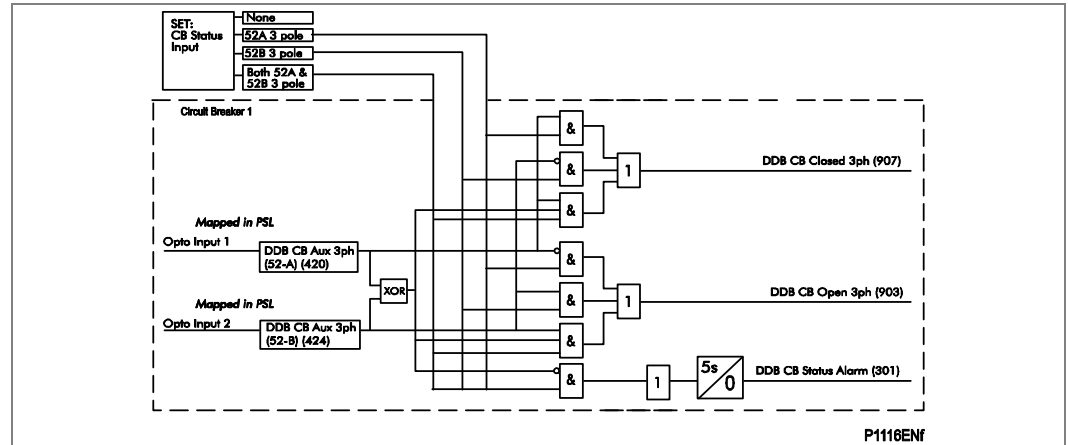
Figure 83 - Circuit breaker state monitor
