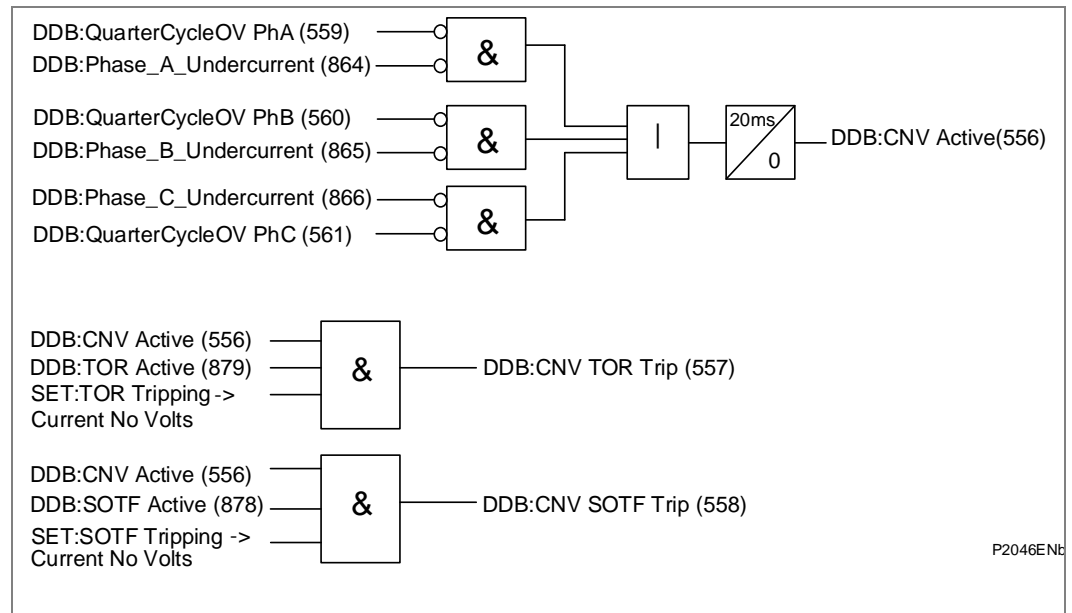
Figure 16 - Trip on close based on CNV level detectors
