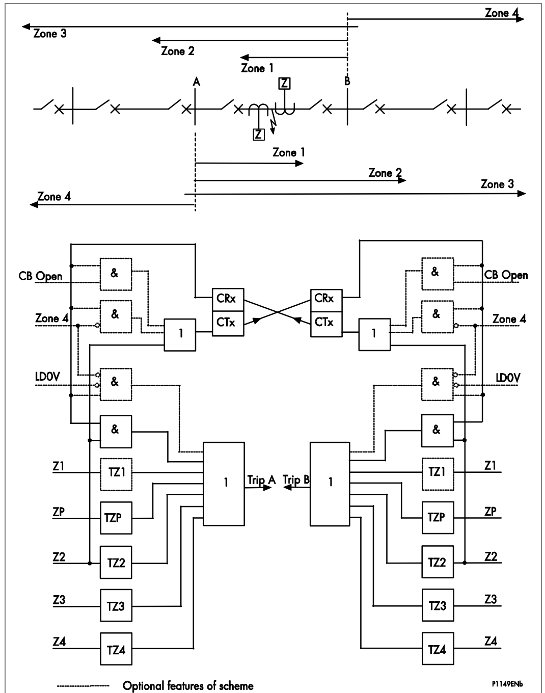
Figure 24 - Permissive OverReach (POR) transfer trip scheme
