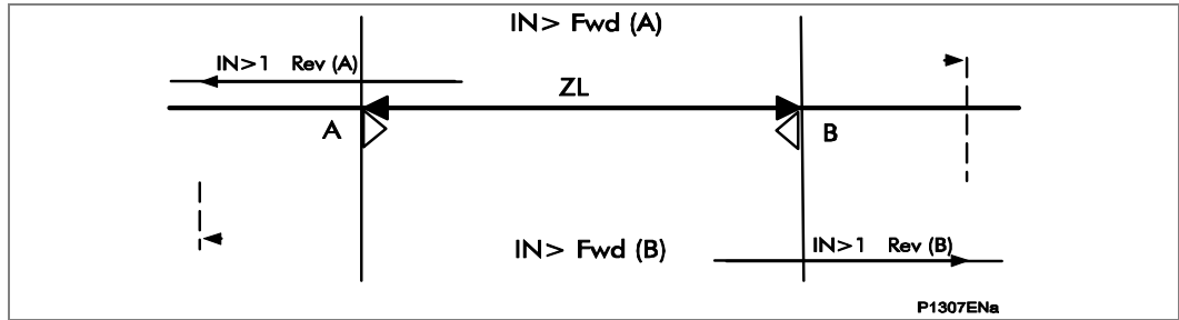
Figure 32 - The DEF blocking scheme
