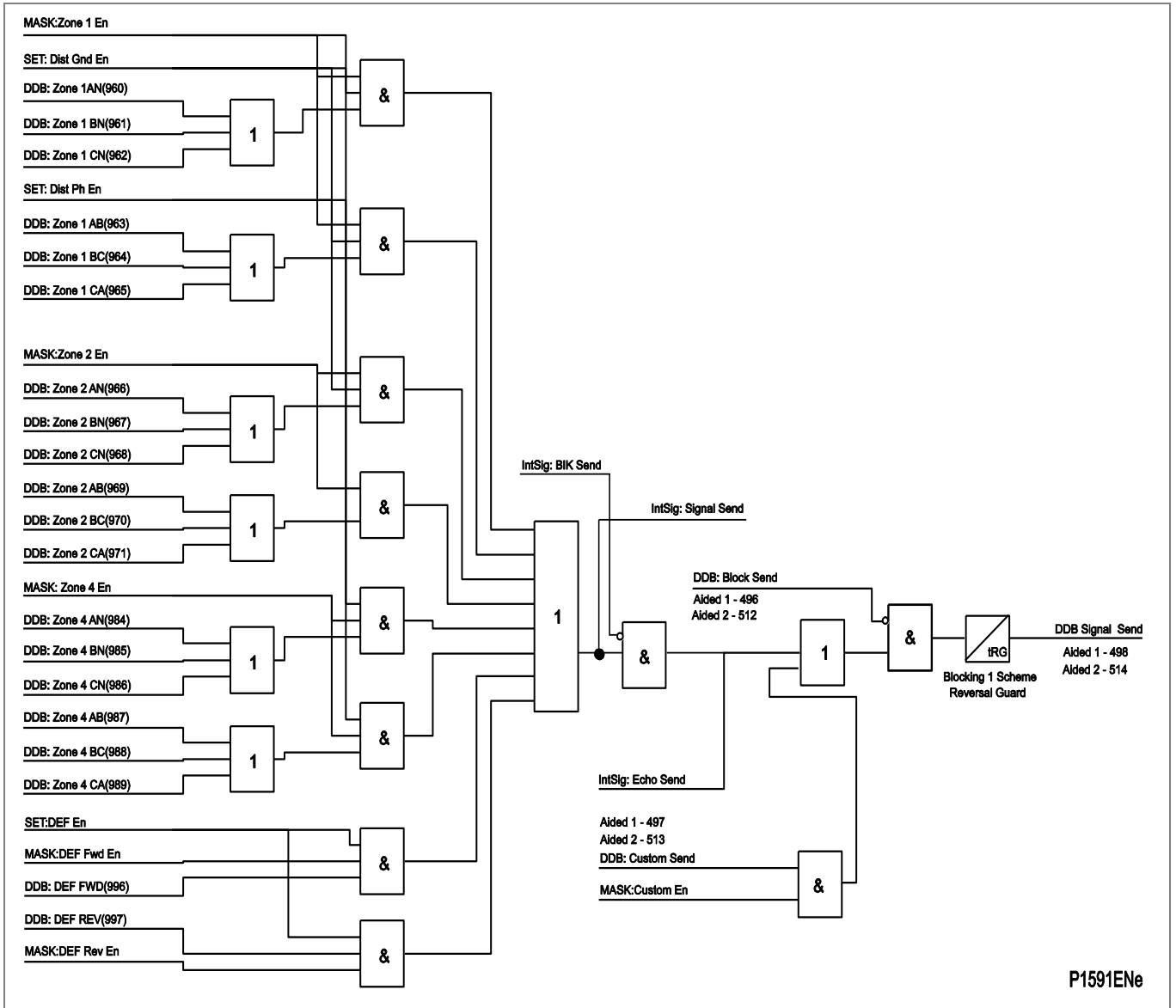
Figure 19 - Send logic
