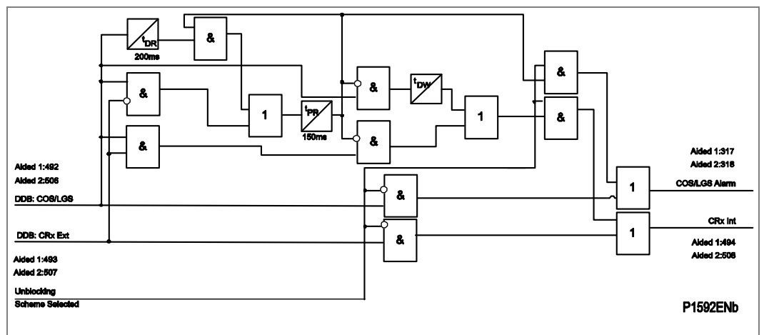
Figure 20 - Receive logic
