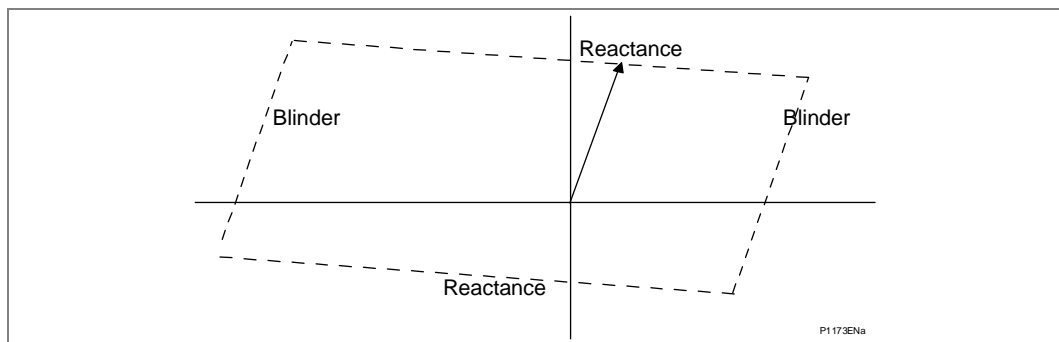
Figure 7 - Offset quadrilateral for zone 3
