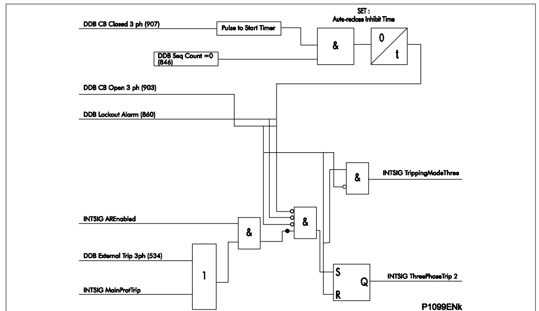
Figure 74 - Auto-reclose tripping
