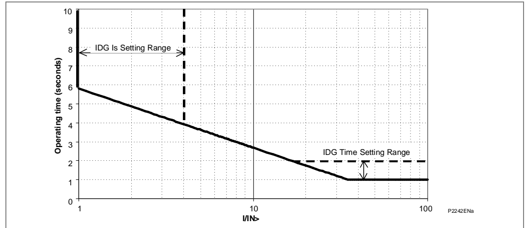
Figure 52 - IDG characteristic
