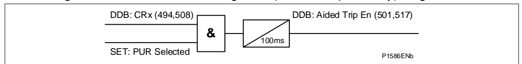
Figure 23 - PUR
