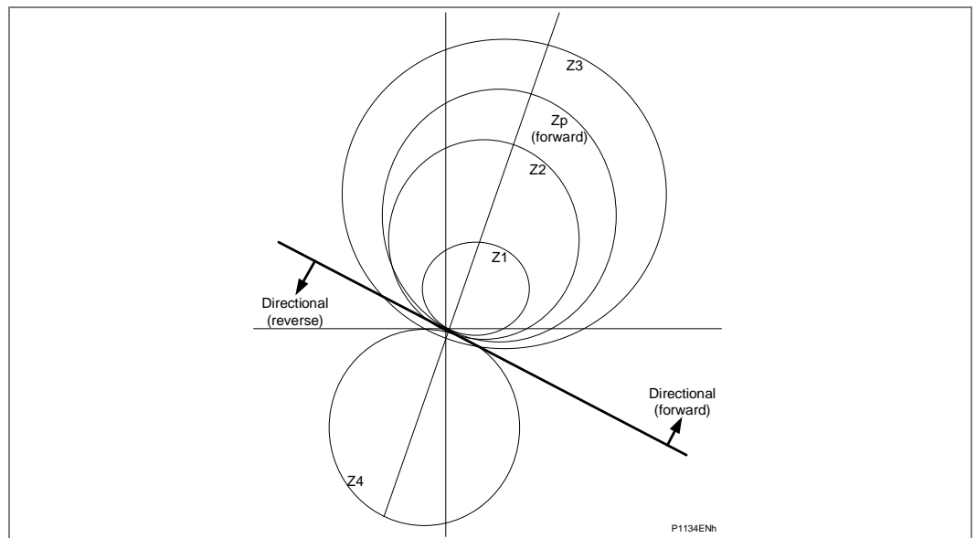
Figure 1 - Phase fault Mho characteristics
