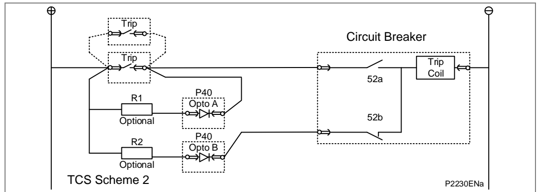
Figure 22 - TCS scheme 2a
