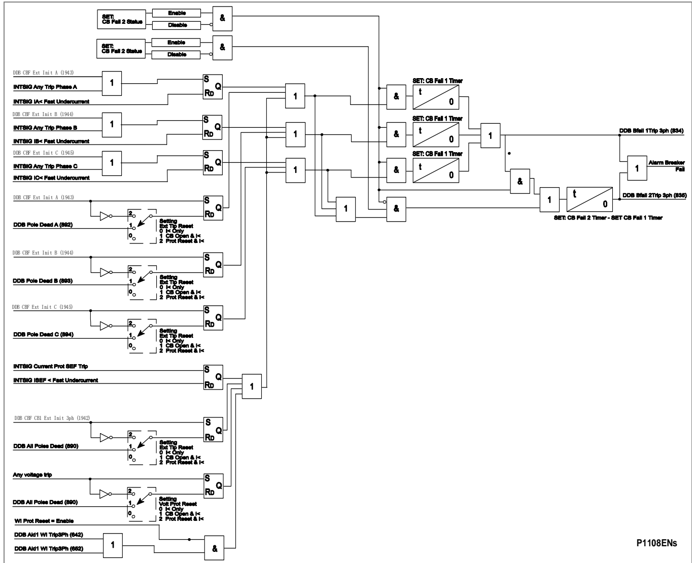
Figure 63 - CB failure for MiCOM P445
