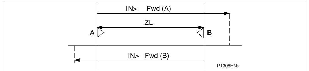
Figure 30 - The DEF permissive scheme
