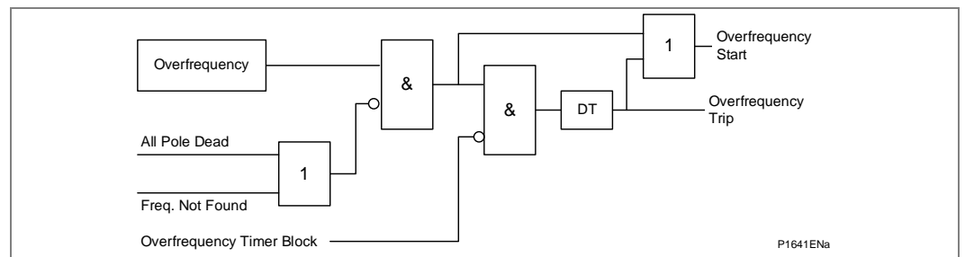
Figure 66 - Overfrequency logic (single stage)
