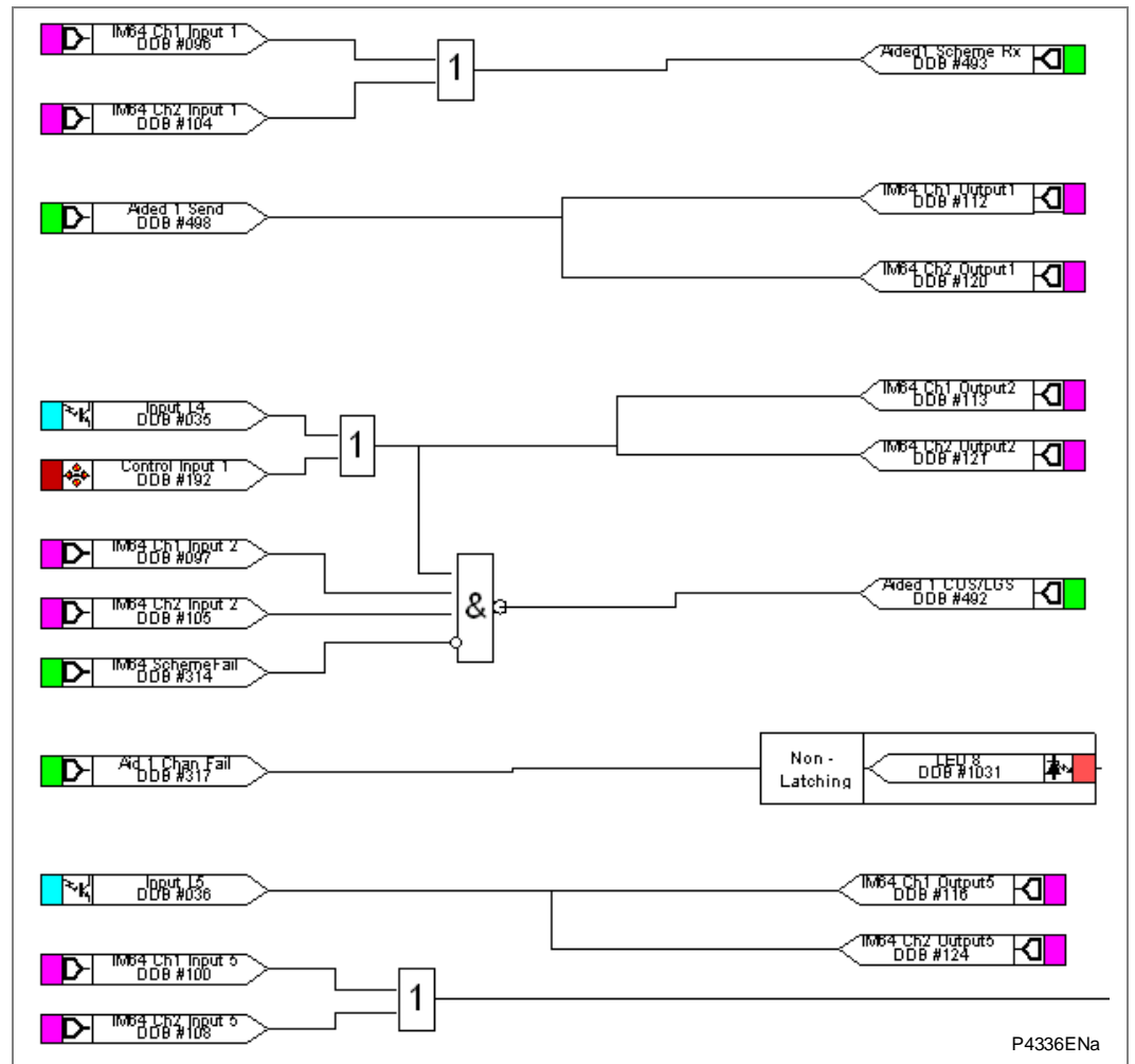
Figure 27 - InterMiCOM 64 mapping in a three ended application
