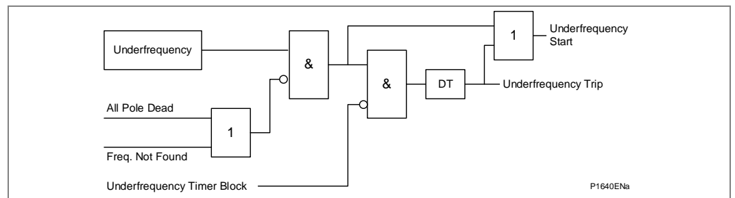
Figure 65 - Underfrequency logic (single stage)
