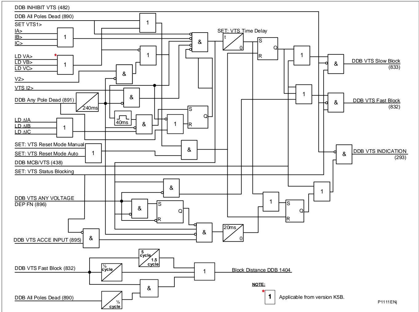
Figure 81 - VTS logic
