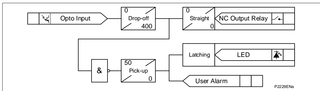
Figure 21 - PSL for TCS schemes 1 and 3
