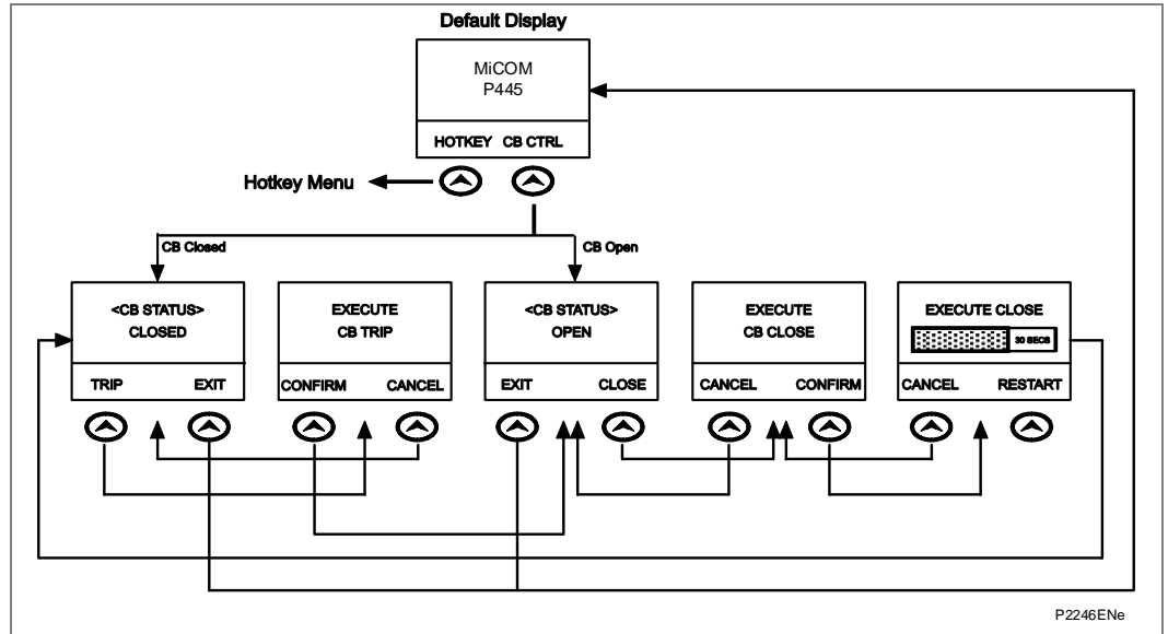
Figure 89 - CB control hotkey menu
