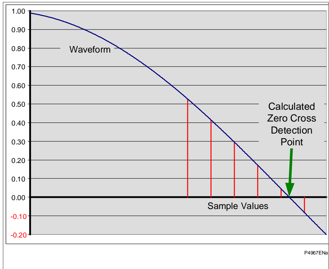
Figure 62 - Calculating a Zero Cross Detection Point using sample values
