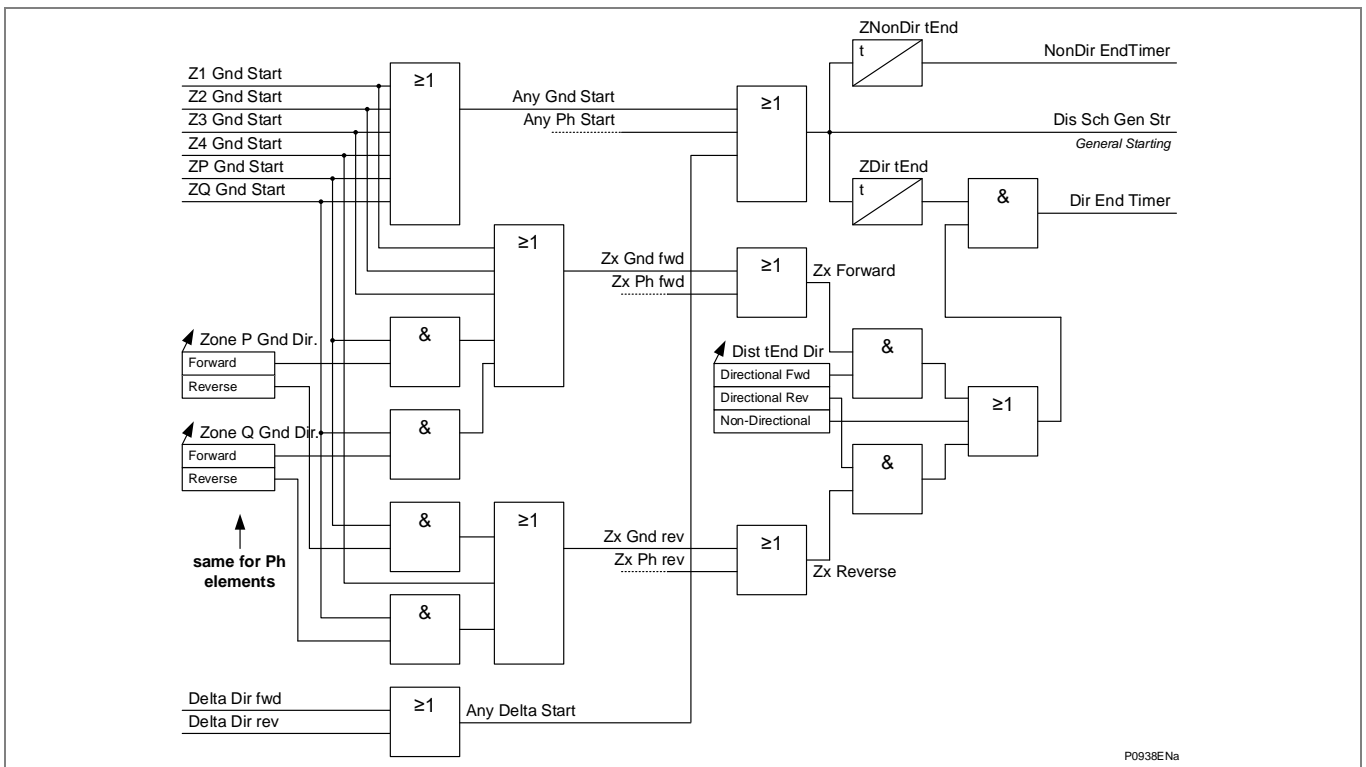
Figure 3 - General starting logic and end timers
