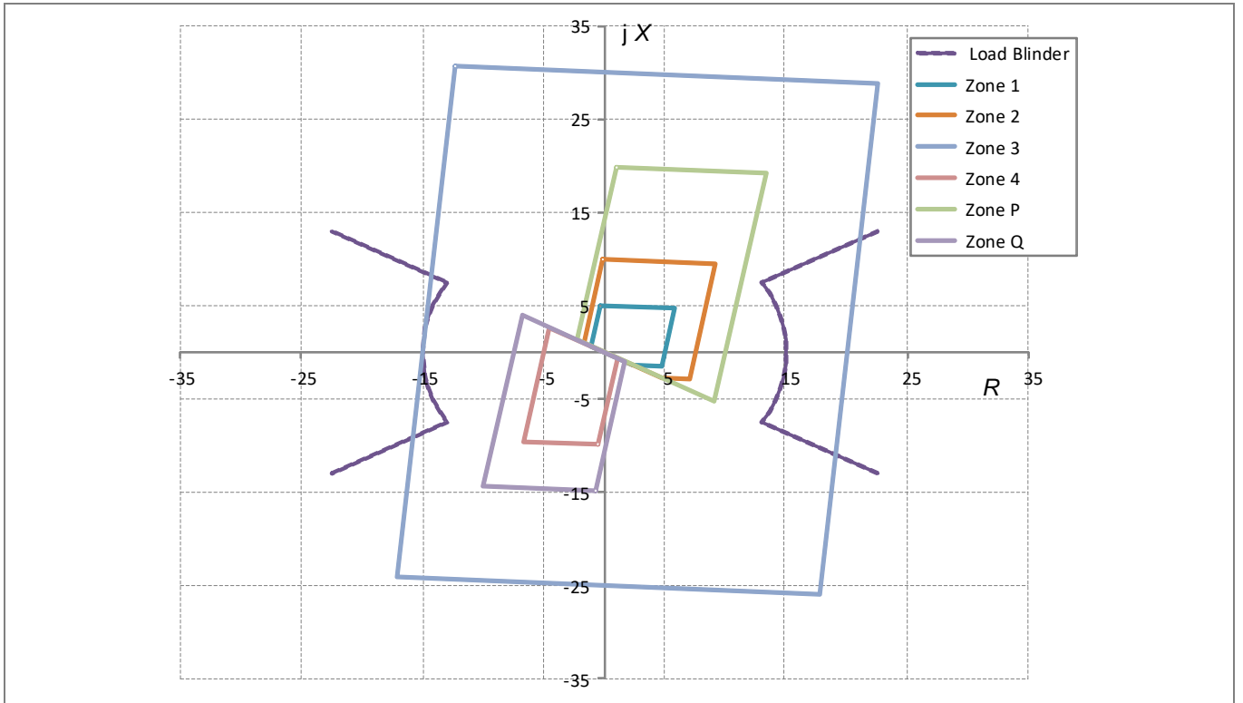
Figure 1 - Zone reach setting with load blinders and underimpedance starting for application example
