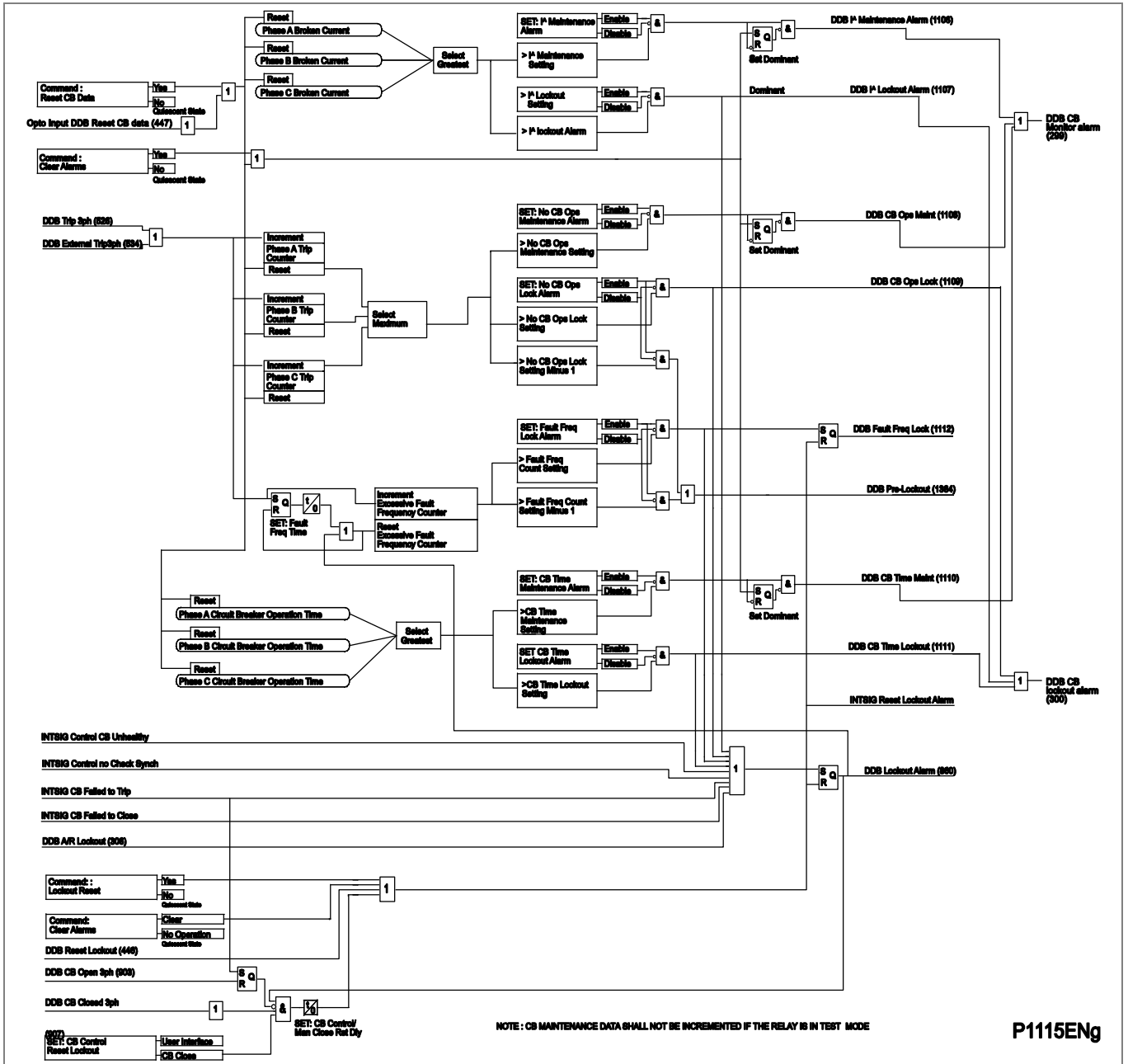
Figure 86 - CB monitoring
