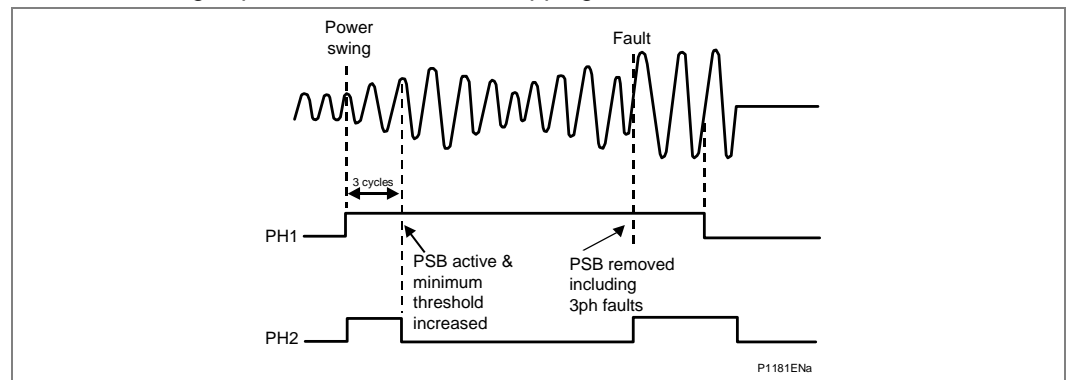
Figure 13 - Power swing detected for 3 cycles continuous \Delta I
