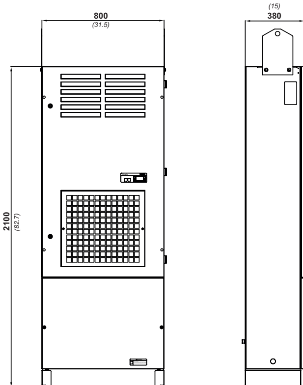
NSYCU8K3P4 - NSYCU8K3P460 - NSYCU10K3P4 - NSYCU10K3P460 (mm / inch)
