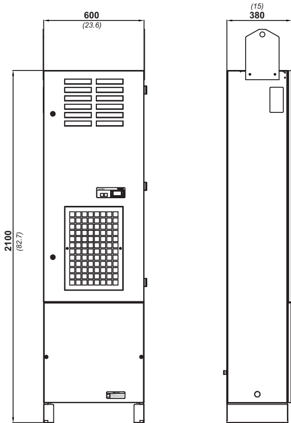
NSYCU8K3P4 - NSYCU8K3P460 - NSYCU10K3P4 - NSYCU10K3P460 (mm / inch)
